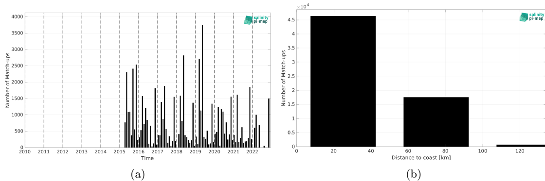
Figure 1: Number of match-ups between ICES and SMAP SSS L3 v5.0 - Monthly (JPL) SSS as a function of time (a) and as function of the distance to coast (b) over the Baltic Sea Pi-MEP region and for the full satellite product period.
