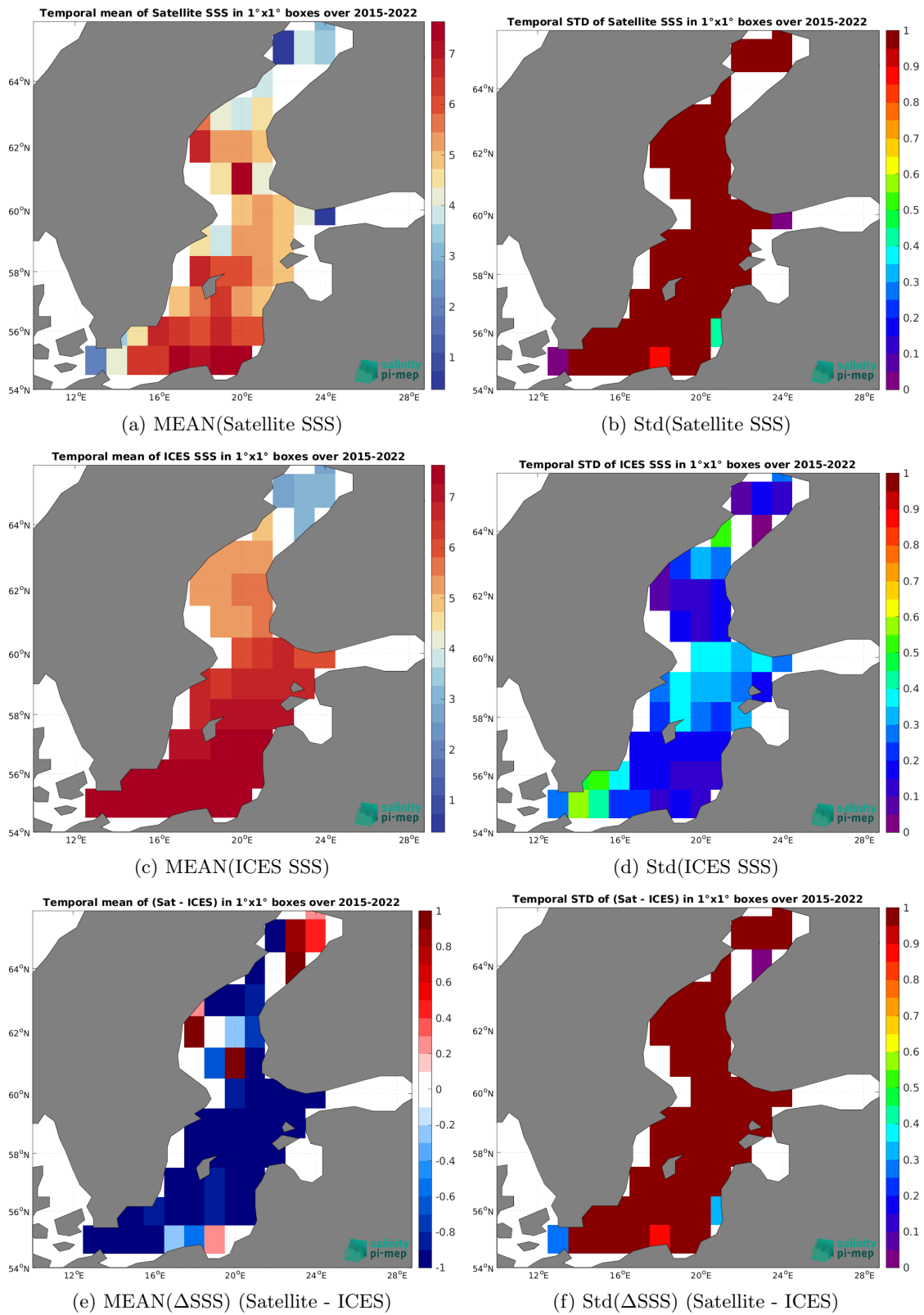
Figure 6: Temporal mean (left) and Std (right) of SSS from SMAP SSS L3 v5.0 - Monthly (JPL) (top), ICES (middle), and of \Delta SSS (Satellite - ICES). Only match-up pairs are used to generate these maps.
