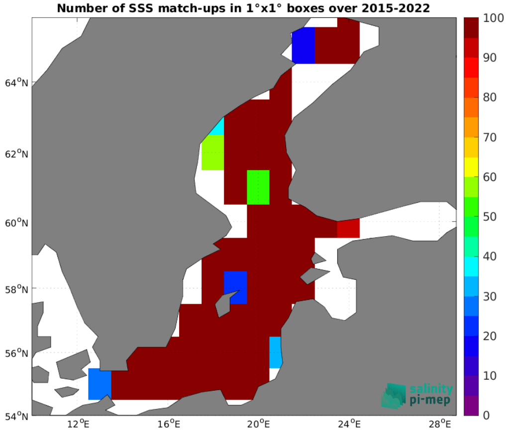
Figure 4: Number of SSS match-ups between ICES SSS and the SMAP SSS L3 v5.0 - Monthly (JPL) SSS product for the Baltic Sea Pi-MEP region over 1^\circ \times 1^\circ boxes and for the full satellite product period.
