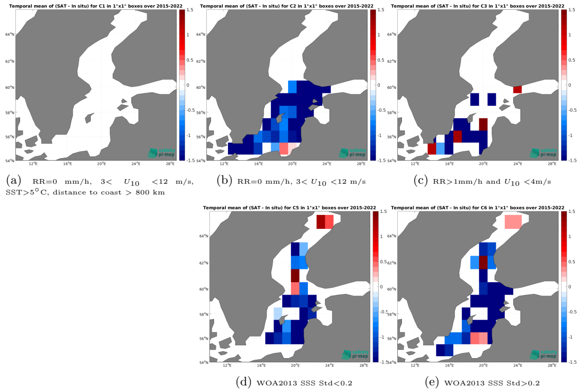
Figure 12: Temporal mean gridded over spatial boxes of size 1^{\circ}\times 1^{\circ} of \Delta\text{SSS} (SMAP SSS L3 v5.0 - Monthly (JPL) - ICES) for 5 different subdatasets corresponding to: \text{RR}=0 mm/h, 3 < U_{10} < 12 m/s, \text{SST} > 5^{\circ}\text{C} , distance to coast > 800 km (a), \text{RR}=0 mm/h, 3 < U_{10} < 12 m/s (b), \text{RR} > 1\text{mm/h} and U_{10} < 4\text{m/s} (c), WOA2013 SSS Std < 0.2 (d), WOA2013 SSS Std > 0.2 (e).
