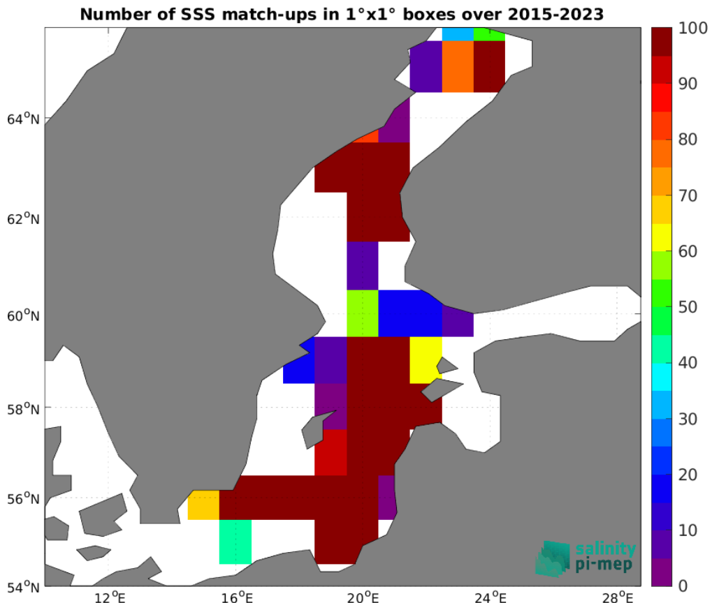
Figure 4: Number of SSS match-ups between Argo SSS and the SMAP SSS L3 v5.0 - Monthly (JPL) SSS product for the Baltic Sea Pi-MEP region over 1°x1° boxes and for the full satellite product period.
