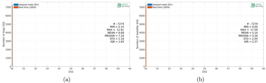
Figure 2: Histograms of SSS from Argo (a) and SMAP SSS L3 v5.0 - Monthly (JPL) (b) considering all match-up pairs per bins of 0.1 over the Baltic Sea Pi-MEP region and for the full satellite product period.
