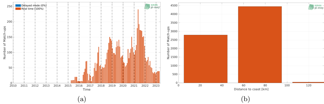
Figure 1: Number of match-ups between Argo and SMAP SSS L3 v5.0 - Monthly (JPL) SSS as a function of time (a) and as function of the distance to coast (b) over the Baltic Sea Pi-MEP region and for the full satellite product period.
