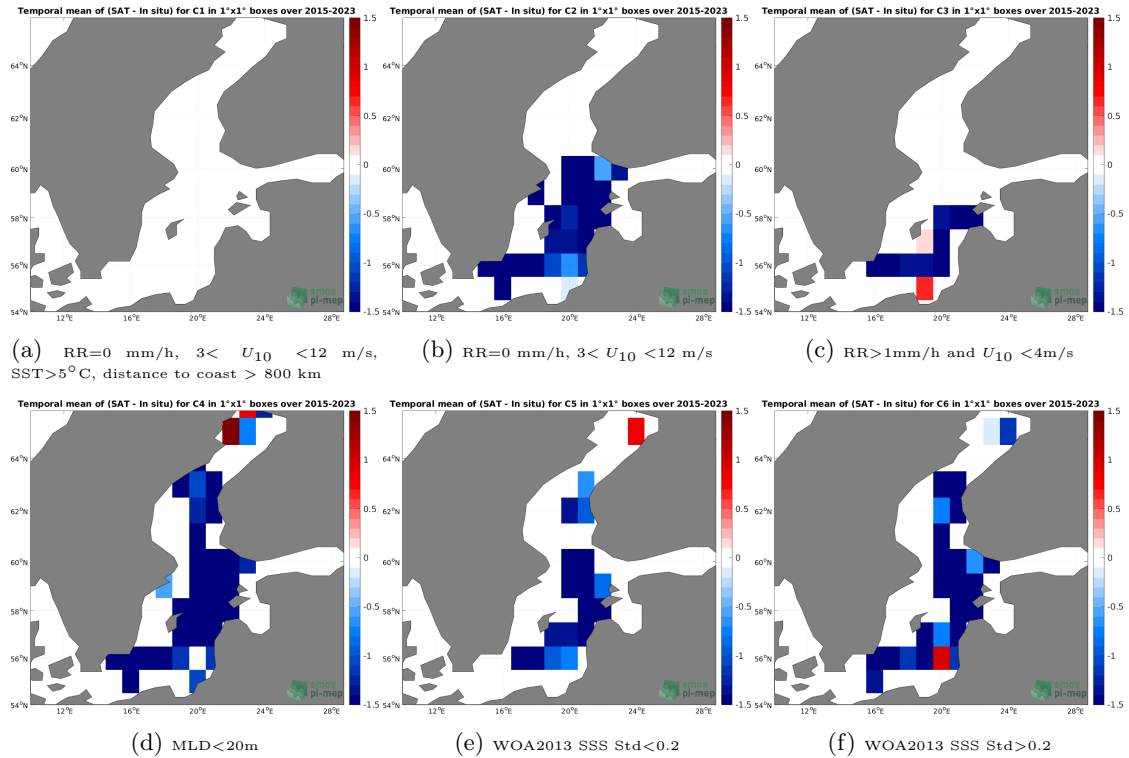
Figure 12: Temporal mean gridded over spatial boxes of size 1^{\circ}\times 1^{\circ} of \Delta\text{SSS} (SMAP SSS L3 v5.0 - Monthly (JPL) - Argo) for 6 different subdatasets corresponding to:RR=0 mm/h, 3 < U_{10} < 12 m/s, SST >5^{\circ}\text{C} , distance to coast > 800 km (a), RR=0 mm/h, 3 < U_{10} < 12 m/s (b), RR >1 mm/h and U_{10} < 4 m/s (c),MLD <20 m (d),WOA2013 SSS Std <0.2 (e),WOA2013 SSS Std >0.2 (f).
