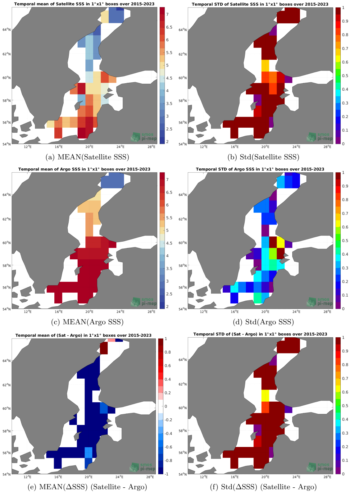
Figure 6: Temporal mean (left) and Std (right) of SSS from SMAP SSS L3 v5.0 - Monthly (JPL) (top), Argo (middle), and of \Delta SSS (Satellite - Argo). Only match-up pairs are used to generate these maps.
