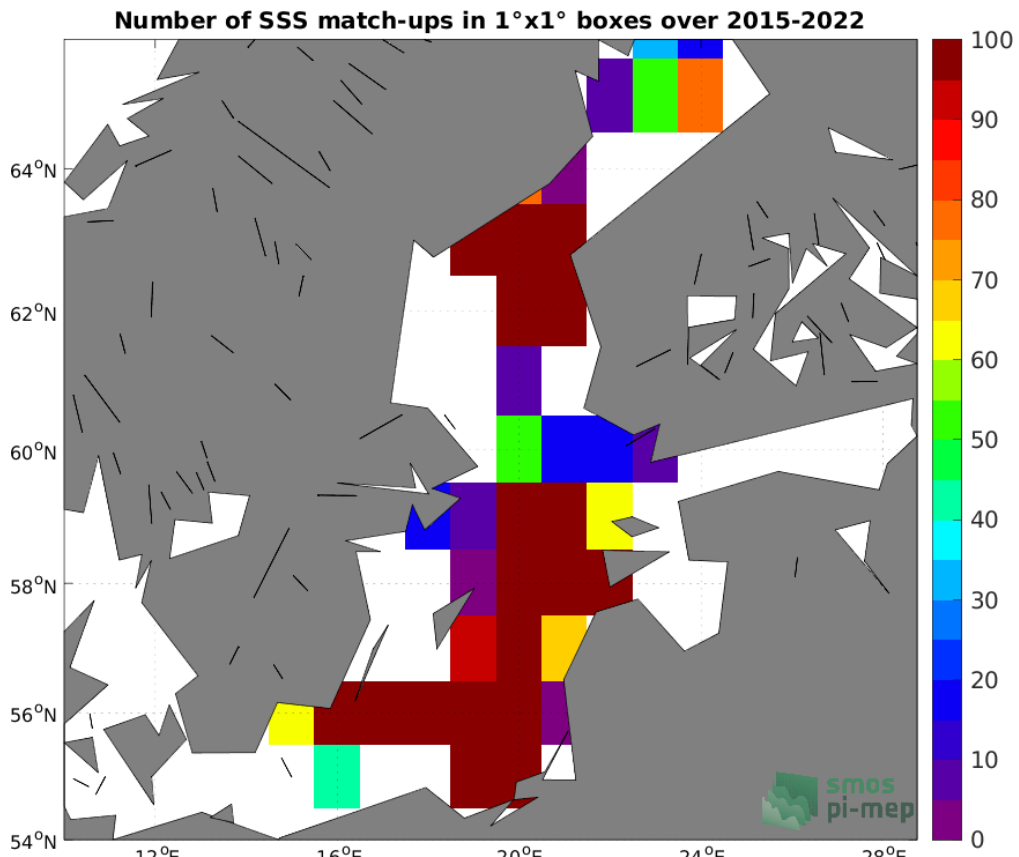
Figure 4: Number of SSS match-ups between Argo SSS and the SMAP SSS L3 v5.0 - Monthly (JPL) SSS product for the Baltic Sea Pi-MEP region over 1^\circ \times 1^\circ boxes and for the full satellite product period.
