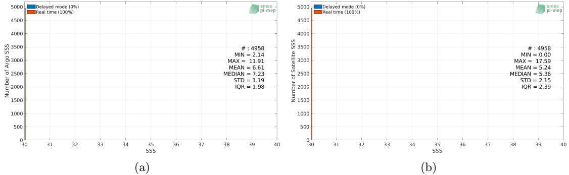
Figure 2: Histograms of SSS from Argo (a) and SMAP SSS L3 v5.0 - Monthly (JPL) (b) considering all match-up pairs per bins of 0.1 over the Baltic Sea Pi-MEP region and for the full satellite product period.
