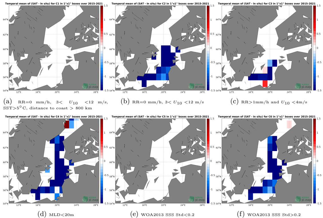
Figure 12: Temporal mean gridded over spatial boxes of size 1^{\circ}\times 1^{\circ} of \Delta\text{SSS} (SMAP SSS L3 v5.0 - Monthly (JPL) - Argo) for 6 different subdatasets corresponding to: RR=0 mm/h, 3 < U_{10} < 12 m/s, SST > 5^{\circ}\text{C} , distance to coast > 800 km (a), RR=0 mm/h, 3 < U_{10} < 12 m/s (b), RR > 1 mm/h and U_{10} < 4 m/s (c), MLD < 20\text{m} (d), WOA2013 SSS Std < 0.2 (e), WOA2013 SSS Std > 0.2 (f).
