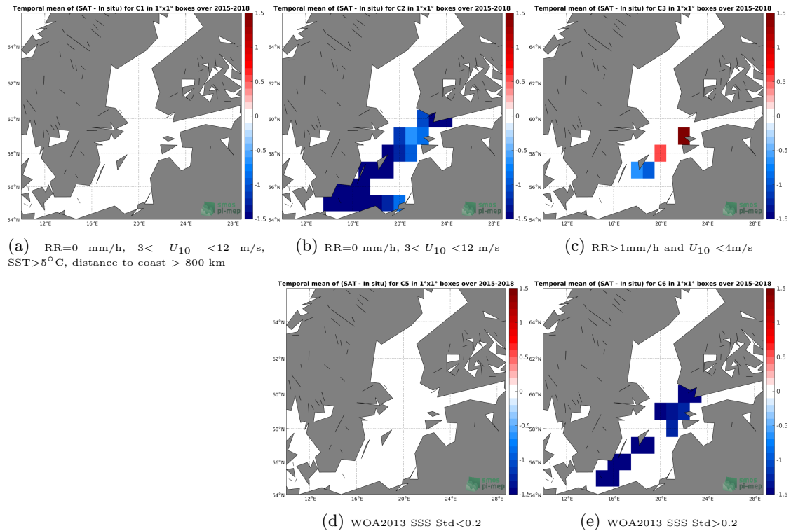
Figure 12: Temporal mean gridded over spatial boxes of size 1^{\circ}\times 1^{\circ} of \Delta\text{SSS} (SMAP-L3-JPL-V4.3-MONTHLY-60KM - TSG-LEGOS-DM) for 5 different subdatasets corresponding to:RR=0 mm/h, 3 < U_{10} < 12 m/s, SST > 5^{\circ}\text{C} , distance to coast > 800 km (a), RR=0 mm/h, 3 < U_{10} < 12 m/s (b), RR > 1 mm/h and U_{10} < 4 m/s (c), WOA2013 SSS Std < 0.2 (d), WOA2013 SSS Std > 0.2 (e).
