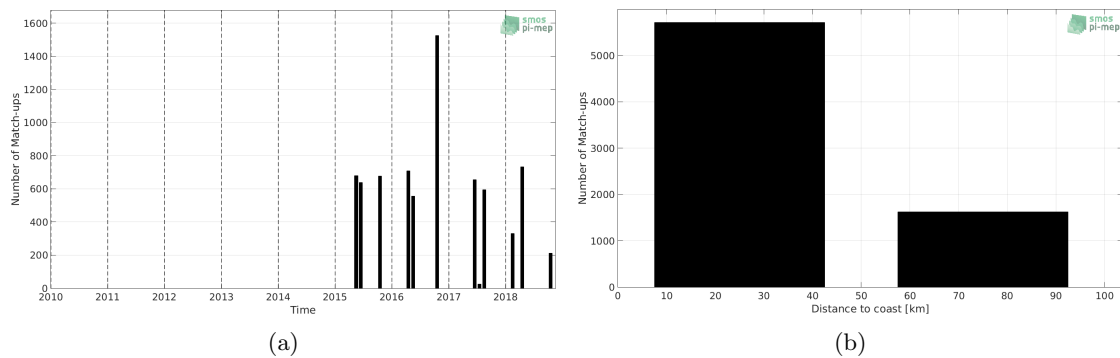
Figure 1: Number of match-ups between TSG-LEGOS-DM and SMAP-L3-JPL-V4.3-MONTHLY-60KM SSS as a function of time (a) and as function of the distance to coast (b) over the Baltic Sea Pi-MEP region and for the full satellite product period.
