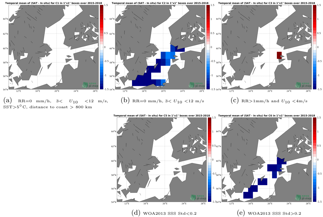
Figure 12: Temporal mean gridded over spatial boxes of size 1^\circ \times 1^\circ of \Delta SSS (SMAP-L3-JPL-V4.3-MONTHLY-60KM - TSG-LEGOS-DM) for 5 different subdatasets corresponding to:RR=0 mm/h, 3 < U_{10} < 12 m/s, SST >5^\circ C, distance to coast > 800 km (a), RR=0 mm/h, 3 < U_{10} < 12 m/s (b), RR >1 mm/h and U_{10} < 4 m/s (c), WOA2013 SSS Std <0.2 (d), WOA2013 SSS Std >0.2 (e).
