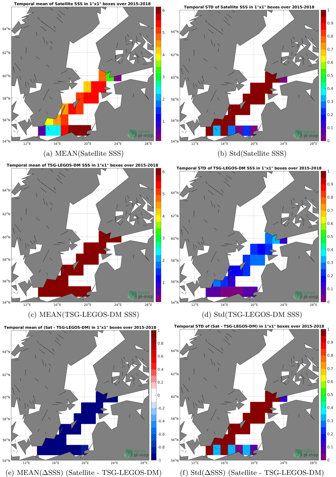
Figure 6: Temporal mean (left) and Std (right) of SSS from SMAP-L3-JPL-V4.3-MONTHLY-60KM (top), TSG-LEGOS-DM (middle), and \Delta SSS (Satellite - TSG-LEGOS-DM). Only match-up pairs are used to generate these maps.
