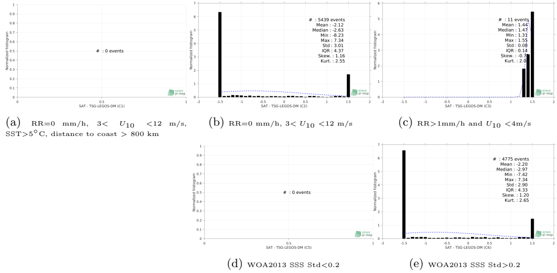
Figure 13: Normalized histogram of \Delta SSS (SMAP-L3-JPL-V4.3-MONTHLY-60KM - TSG-LEGOS-DM) for 5 different subdatasets corresponding to: RR=0 mm/h, 3 < U_{10} < 12 m/s, SST>5°C, distance to coast > 800 km (a), RR=0 mm/h, 3 < U_{10} < 12 m/s (b), RR>1mm/h and U_{10} < 4 m/s (c), WOA2013 SSS Std<0.2 (d), WOA2013 SSS Std>0.2 (e).
