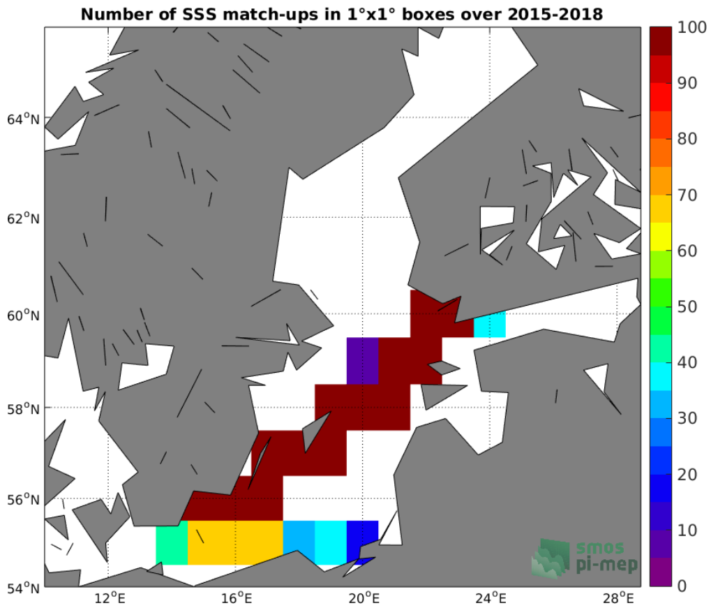
Figure 4: Number of SSS match-ups between TSG-LEGOS-DM SSS and the SMAP-L3-JPL-V4.3-MONTHLY-60KM SSS product for the Baltic Sea Pi-MEP region over 1°x1° boxes and for the full satellite product period.
