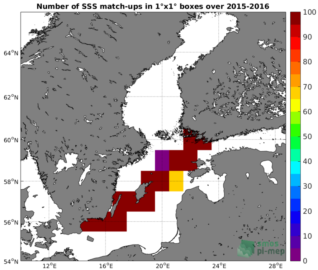
Figure 4: Number of SSS match-ups between TSG-LEGOS-DM SSS and the SMAP-L3-JPL-V4-8DAY-RUNNING-60KM SSS product for the Baltic Sea Pi-MEP region over 1°x1° boxes and for the full satellite product period.
