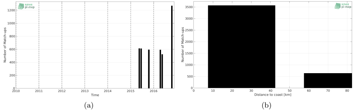
Figure 1: Number of match-ups between TSG-LEGOS-DM and SMAP-L3-JPL-V4-8DAY-RUNNING-60KM SSS as a function of time (a) and as function of the distance to coast (b) over the Baltic Sea Pi-MEP region and for the full satellite product period.
