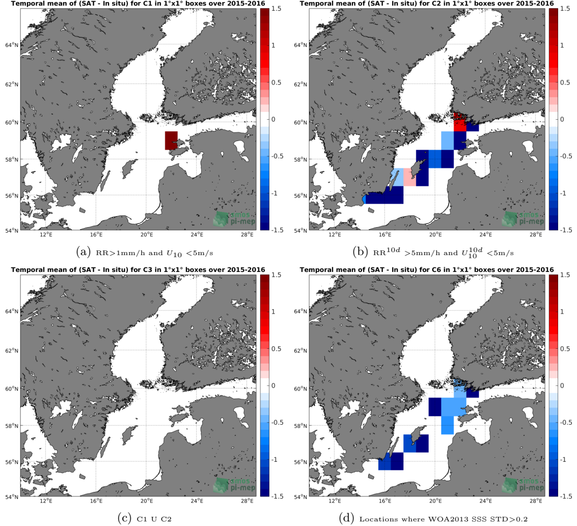
Figure 12: Temporal mean gridded over spatial boxes of size 1^\circ \times 1^\circ of \Delta SSS (SMAP-L3-JPL-V4-8DAY-RUNNING-60KM - TSG-LEGOS-DM) for 4 different subdatasets corresponding to: RR > 1\text{mm/h} and U_{10} < 5\text{m/s} (a), RR^{10d} > 5\text{mm/h} and U_{10}^{10d} < 5\text{m/s} (b), C1 U C2 (c), Locations where WOA2013 SSS STD > 0.2 (d).
