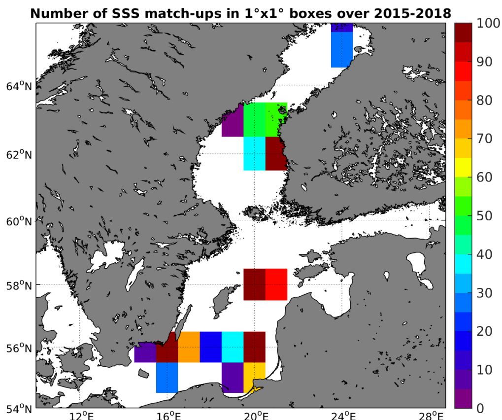
Figure 4: Number of SSS match-ups between Argo SSS and the SMAP-L3-JPL-V4-8DAY-RUNNING-60KM SSS product for the Baltic Sea Pi-MEP region over 1°x1° boxes and for the full satellite product period.
