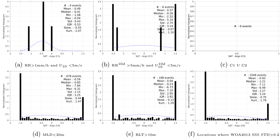
Figure 13: Normalized histogram of \Delta SSS (SMAP-L3-JPL-V4-8DAY-RUNNING-60KM - Argo) for 6 different subdatasets corresponding to: RR > 1\text{mm/h} and U_{10} < 5\text{m/s} (a), RR^{10d} > 5\text{mm/h} and U_{10}^{10d} < 5\text{m/s} (b), C1 U C2 (c), MLD < 20m (d), BLT > 10m (e), Locations where WOA2013 SSS STD > 0.2 (f).
