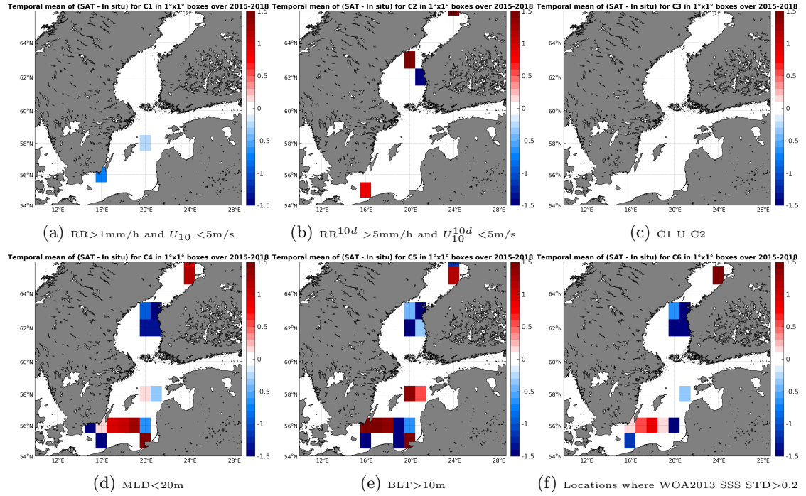
Figure 12: Temporal mean gridded over spatial boxes of size 1^\circ \times 1^\circ of \Delta SSS (SMAP-L3-JPL-V4-8DAY-RUNNING-60KM - Argo) for 6 different subdatasets corresponding to: RR > 1mm/h and U_{10} < 5 m/s (a), RR^{10d} > 5 mm/h and U_{10}^{10d} < 5 m/s (b), C1 U C2 (c), MLD < 20m (d), BLT > 10m (e), Locations where WOA2013 SSS STD > 0.2 (f).
