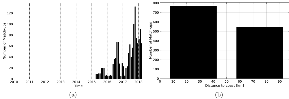
Figure 1: Number of match-ups between Argo and SMAP-L3-JPL-V4-8DAY-RUNNING-60KM SSS as a function of time (a) and as function of the distance to coast (b) over the Baltic Sea Pi-MEP region and for the full satellite product period.
