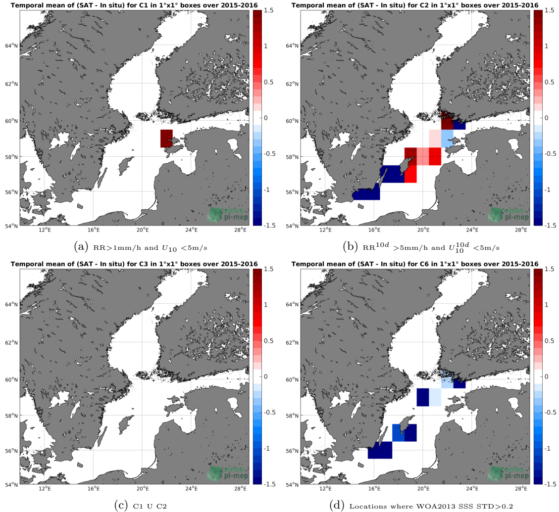
Figure 12: Temporal mean gridded over spatial boxes of size 1^\circ \times 1^\circ of \Delta SSS (SMAP-L3-JPL-V4-MONTHLY-60KM - TSG-LEGOS-DM) for 4 different subdatasets corresponding to: RR > 1\text{mm/h} and U_{10} < 5\text{m/s} (a), RR^{10d} > 5\text{mm/h} and U_{10}^{10d} < 5\text{m/s} (b), C1 U C2 (c), Locations where WOA2013 SSS STD > 0.2 (d).
