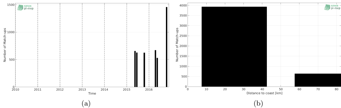
Figure 1: Number of match-ups between TSG-LEGOS-DM and SMAP-L3-JPL-V4-MONTHLY-60KM SSS as a function of time (a) and as function of the distance to coast (b) over the Baltic Sea Pi-MEP region and for the full satellite product period.
