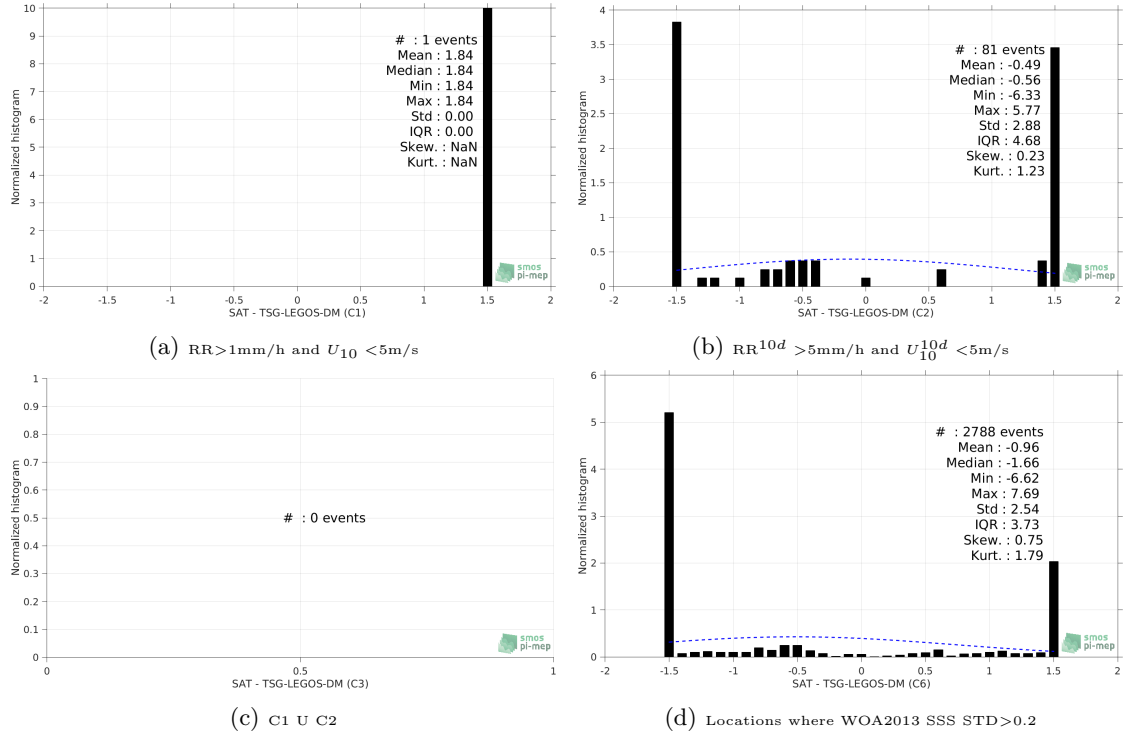
Figure 13: Normalized histogram of \Delta\text{SSS} (SMAP-L3-JPL-V4-MONTHLY-60KM - TSG-LEGOS-DM) for 6 different subdatasets corresponding to: RR > 1\text{mm/h} and U_{10} < 5\text{m/s} (a), RR^{10d} > 5\text{mm/h} and U_{10}^{10d} < 5\text{m/s} (b), C1 U C2 (c), Locations where WOA2013 SSS STD > 0.2 (d).
