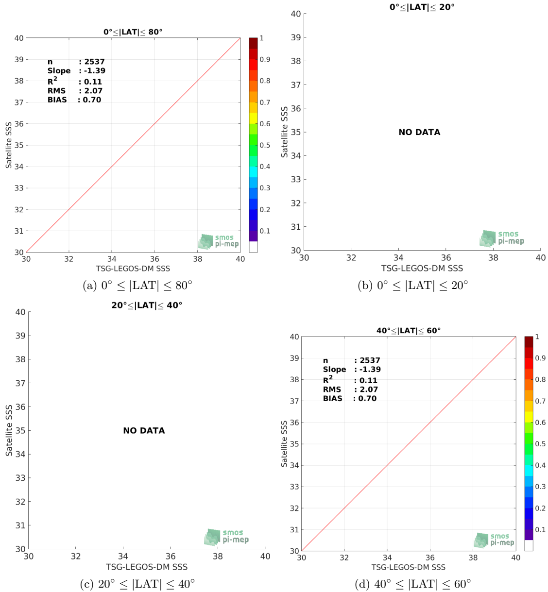
Figure 9: Contour maps of the concentration of SMAP-L3-JPL-V4-MONTHLY-60KM SSS (y-axis) versus TSG-LEGOS-DM SSS (x-axis) at match-up pairs for different latitude bands. For each plot, the red line shows x=y . The black thin and dashed lines indicate a linear fit through the data cloud and the \pm 95\% confidence levels, respectively. The number match-up pairs n , the slope and R^2 coefficient of the linear fit, the root mean square (RMS) and the mean bias between satellite and in situ data are indicated for each latitude band in each plots.
