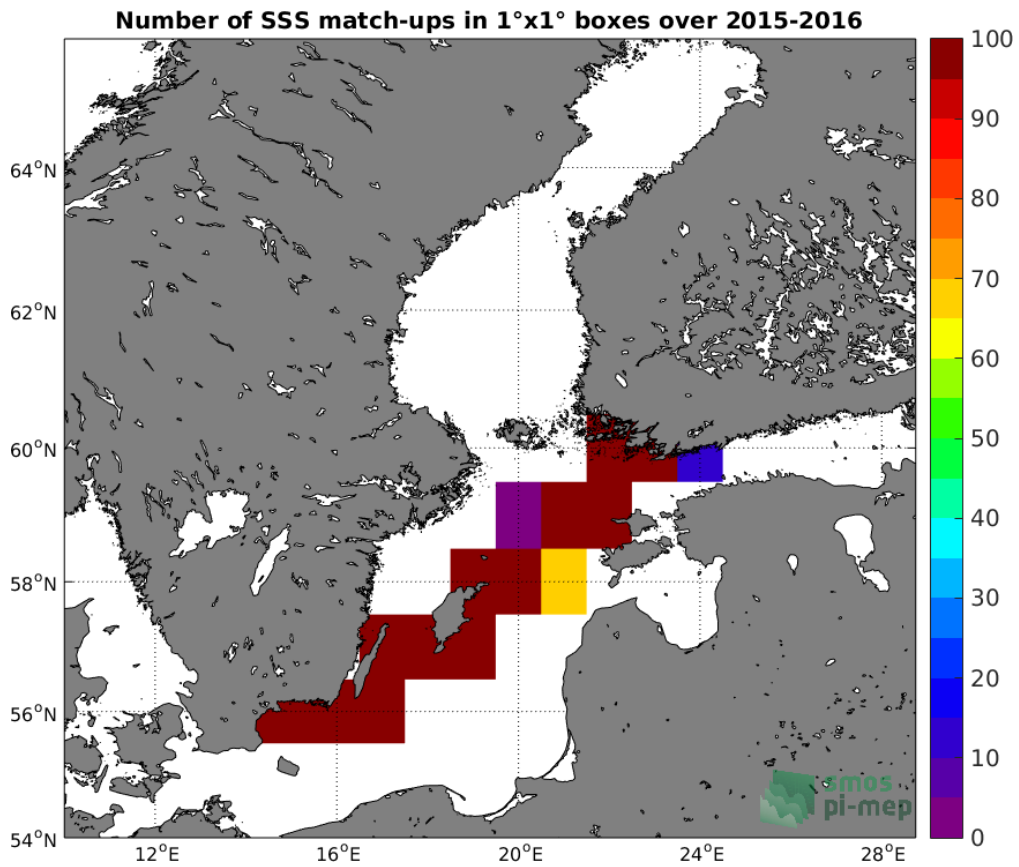
Figure 4: Number of SSS match-ups between TSG-LEGOS-DM SSS and the SMAP-L3-JPL-V4-MONTHLY-60KM SSS product for the Baltic Sea Pi-MEP region over 1°x1° boxes and for the full satellite product period.
