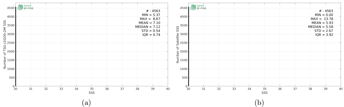
Figure 2: Histograms of SSS from TSG-LEGOS-DM (a) and SMAP-L3-JPL-V4-MONTHLY-60KM (b) considering all match-up pairs per bins of 0.1 over the Baltic Sea Pi-MEP region and for the full satellite product period.
