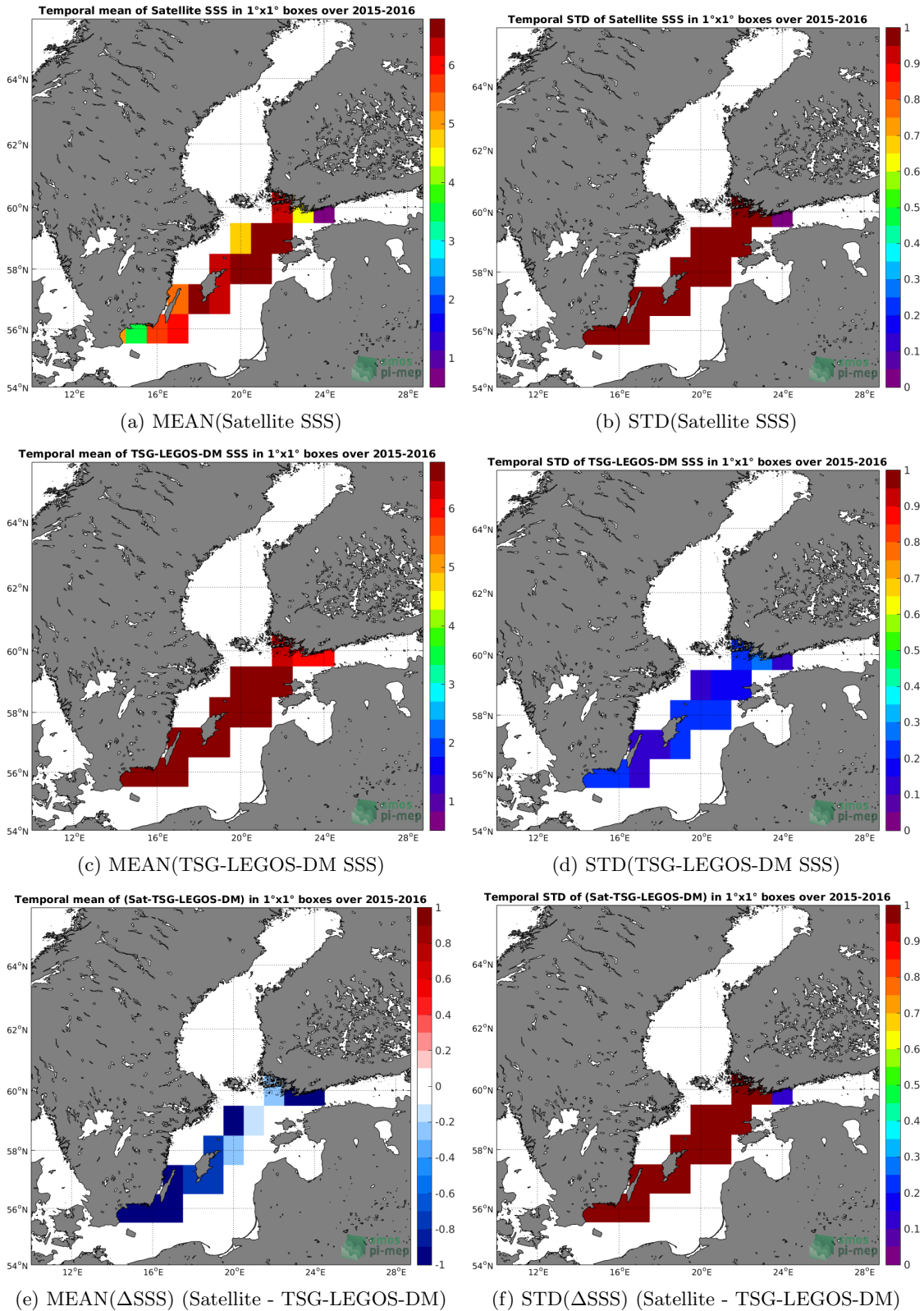
Figure 6: Temporal mean (left) and STD (right) of SSS from SMAP-L3-JPL-V4-MONTHLY-60KM (top), TSG-LEGOS-DM (middle), and \Delta SSS (Satellite - TSG-LEGOS-DM). Only match-up pairs are used to generate these maps.
