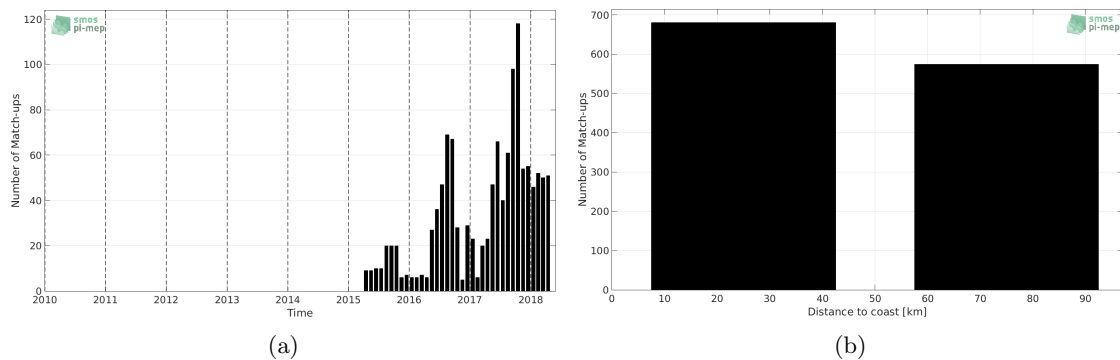
Figure 1: Number of match-ups between Argo and SMAP-L3-JPL-V4-MONTHLY-60KM SSS as a function of time (a) and as function of the distance to coast (b) over the Baltic Sea Pi-MEP region and for the full satellite product period.
