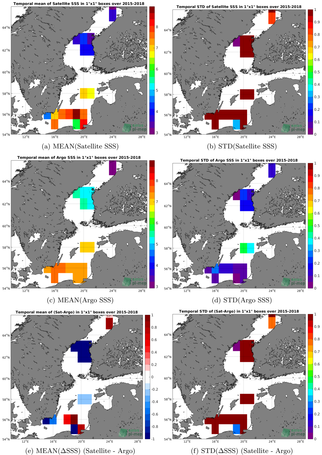
Figure 6: Temporal mean (left) and STD (right) of SSS from SMAP-L3-JPL-V4-MONTHLY-60KM (top), Argo (middle), and of \Delta SSS (Satellite - Argo). Only match-up pairs are used to generate these maps.
