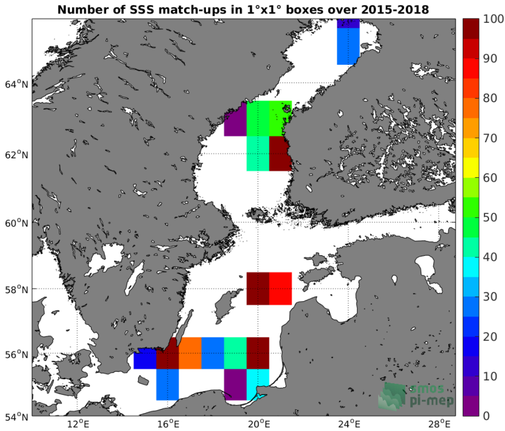
Figure 4: Number of SSS match-ups between Argo SSS and the SMAP-L3-JPL-V4-MONTHLY-60KM SSS product for the Baltic Sea Pi-MEP region over 1°x1° boxes and for the full satellite product period.
