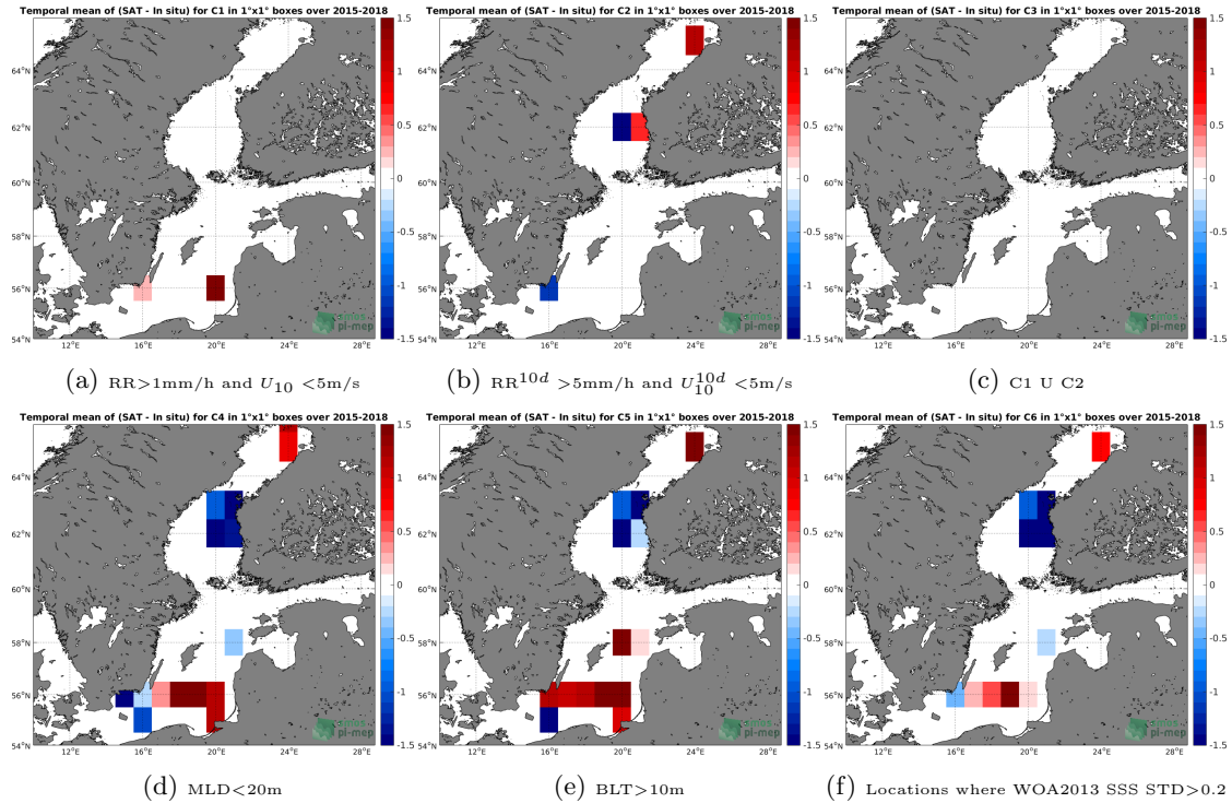
Figure 12: Temporal mean gridded over spatial boxes of size 1^\circ \times 1^\circ of \Delta\text{SSS} (SMAP-L3-JPL-V4-MONTHLY-60KM - Argo) for 6 different subdatasets corresponding to:RR >1\text{mm/h} and U_{10} < 5\text{m/s} (a), RR^{10d} > 5\text{mm/h} and U_{10}^{10d} < 5\text{m/s} (b), C1 U C2 (c),MLD <20\text{m} (d),BLT >10\text{m} (e),Locations where WOA2013 SSS STD >0.2 (f).
