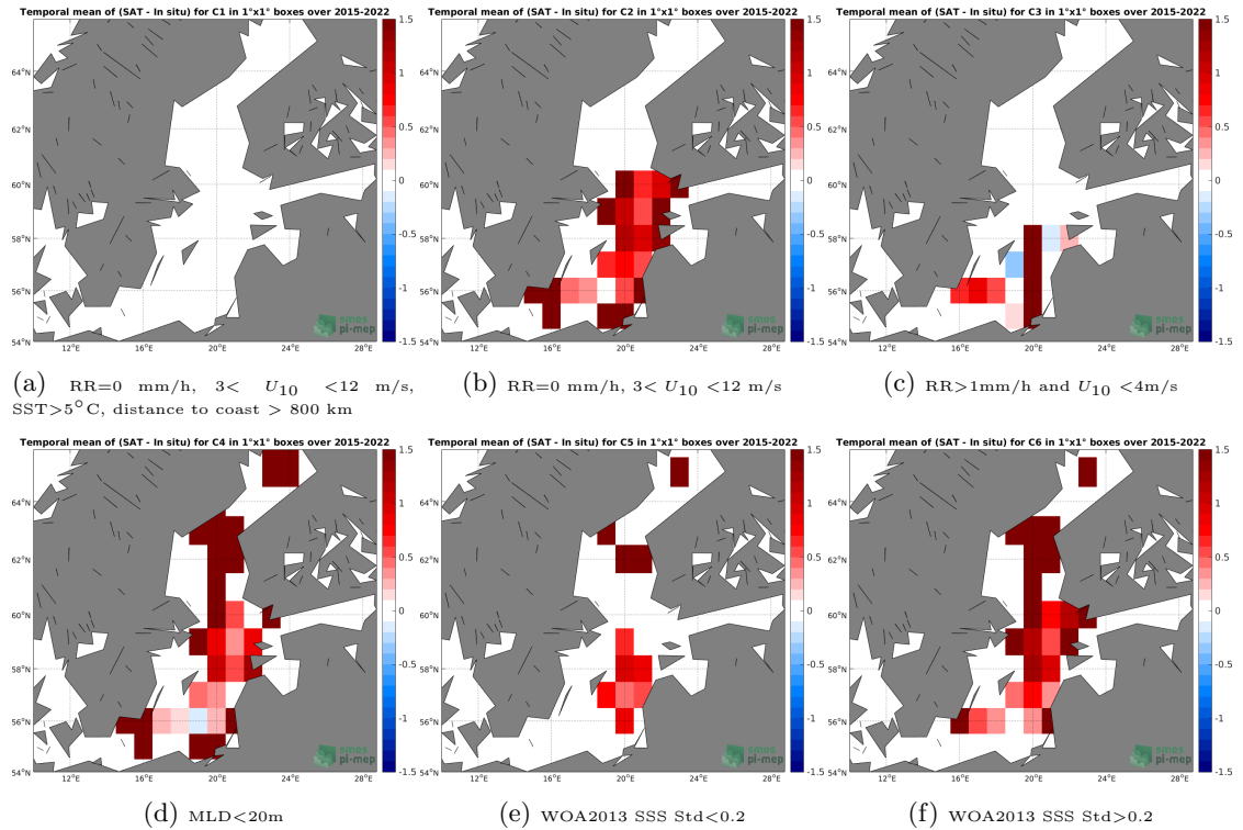
Figure 12: Temporal mean gridded over spatial boxes of size 1^{\circ}\times 1^{\circ} of \Delta\text{SSS} (SMAP SSS L2-AVERAGED v5 (RSS) - Argo) for 6 different subdatasets corresponding to:RR=0 mm/h, 3 < U_{10} < 12 m/s, SST >5^{\circ}\text{C} , distance to coast > 800 km (a), RR=0 mm/h, 3 < U_{10} < 12 m/s (b), RR >1\text{mm/h} and U_{10} < 4\text{m/s} (c),MLD <20\text{m} (d),WOA2013 SSS Std <0.2 (e),WOA2013 SSS Std >0.2 (f).
