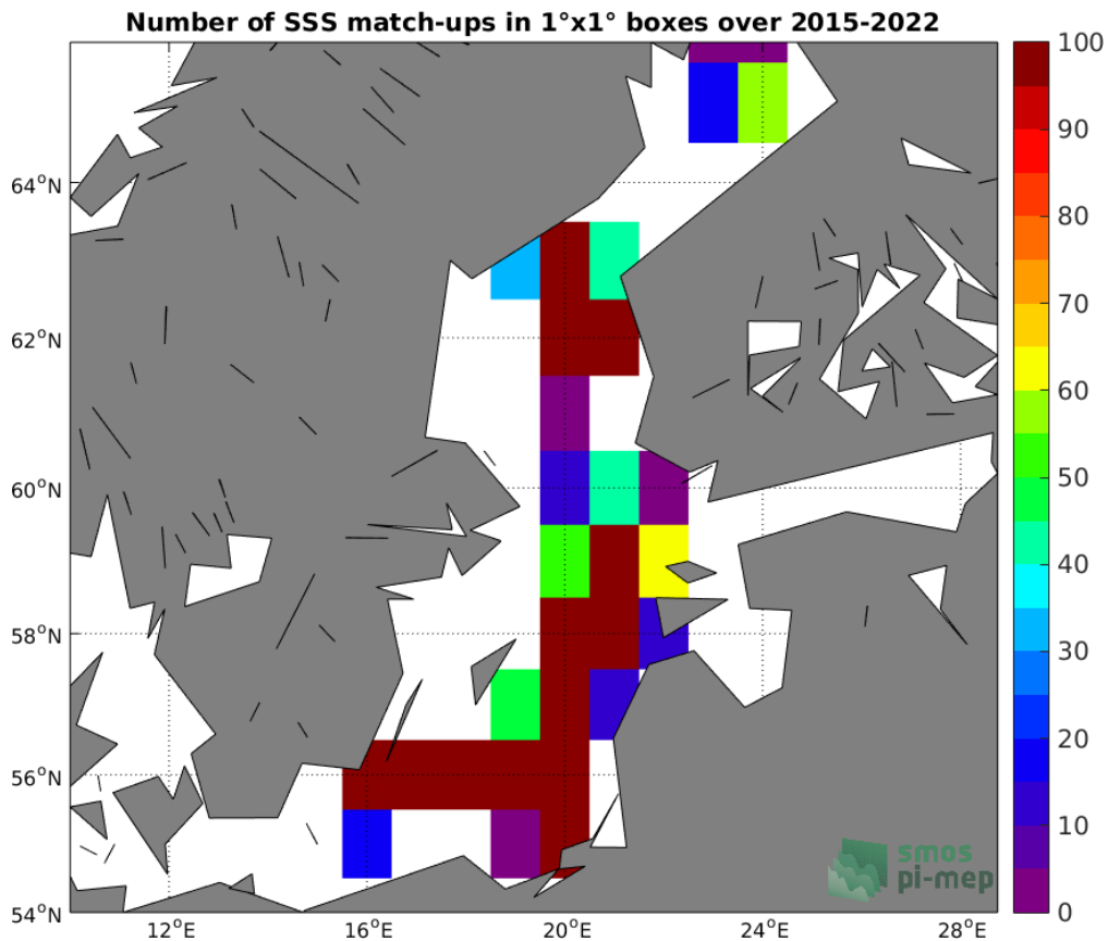
Figure 4: Number of SSS match-ups between Argo SSS and the SMAP SSS L2-AVERAGED v5 (RSS) SSS product for the Baltic Sea Pi-MEP region over 1°×1° boxes and for the full satellite product period.
