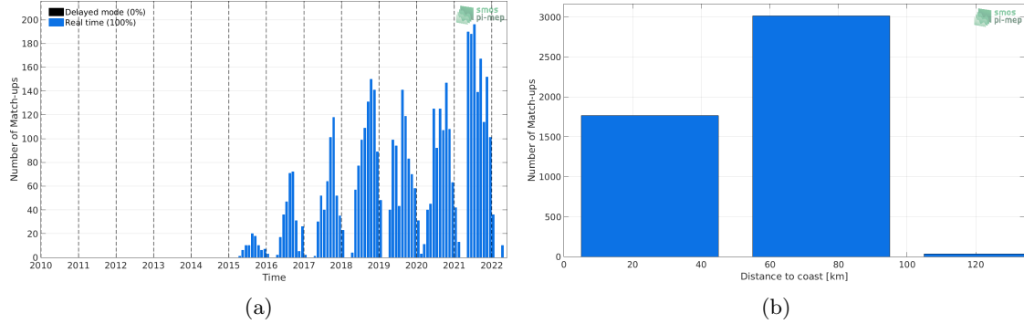
Figure 1: Number of match-ups between Argo and SMAP SSS L2-AVERAGED v5 (RSS) SSS as a function of time (a) and as function of the distance to coast (b) over the Baltic Sea Pi-MEP region and for the full satellite product period.
