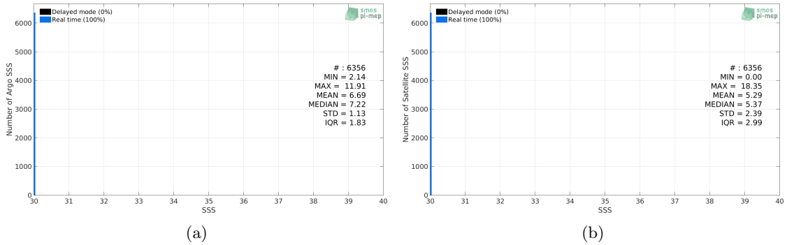
Figure 2: Histograms of SSS from Argo (a) and SMAP SSS L2-AVERAGED v5.0 (JPL) (b) considering all match-up pairs per bins of 0.1 over the Baltic Sea Pi-MEP region and for the full satellite product period.
