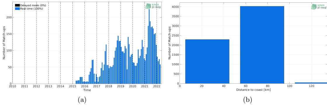
Figure 1: Number of match-ups between Argo and SMAP SSS L2-AVERAGED v5.0 (JPL) SSS as a function of time (a) and as function of the distance to coast (b) over the Baltic Sea Pi-MEP region and for the full satellite product period.
