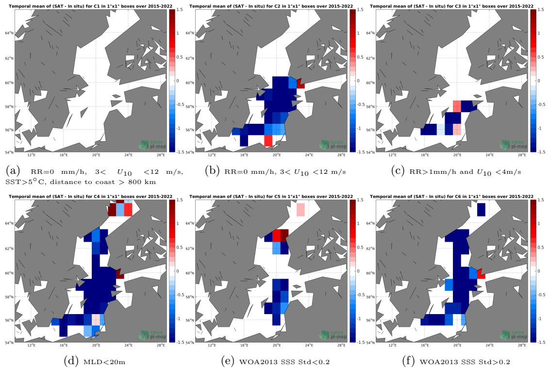
Figure 12: Temporal mean gridded over spatial boxes of size 1^{\circ}\times 1^{\circ} of \Delta\text{SSS} (SMAP SSS L2-AVERAGED v5.0 (JPL) - Argo) for 6 different subdatasets corresponding to:RR=0 mm/h, 3 < U_{10} < 12 m/s, SST >5^{\circ}\text{C} , distance to coast > 800 km (a), RR=0 mm/h, 3 < U_{10} < 12 m/s (b), RR >1\text{mm/h} and U_{10} < 4\text{m/s} (c),MLD <20\text{m} (d),WOA2013 SSS Std <0.2 (e),WOA2013 SSS Std >0.2 (f).
