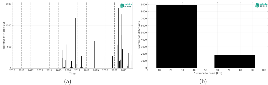
Figure 2: Number of match-ups between TSG (LEGOS-DM) and SMAP SSS L2 v6 - 40 km (RSS) SSS as a function of time (a) and as function of the distance to coast (b) over the Baltic Sea Pi-MEP region and for the full satellite product period.
