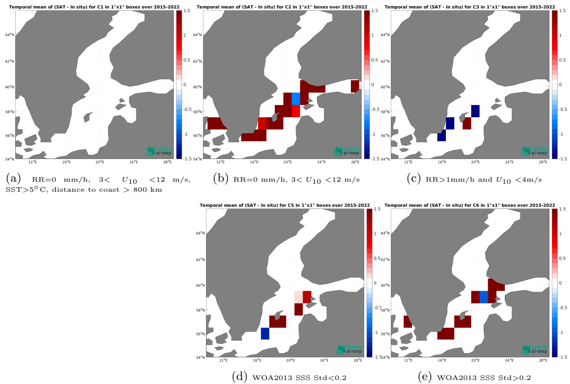
Figure 14: Temporal mean gridded over spatial boxes of size 1^\circ \times 1^\circ of \Delta\text{SSS} (SMAP SSS L2 v6 - 40 km (RSS) - TSG (LEGOS-DM)) for 5 different subdatasets corresponding to:RR=0 mm/h, 3 < U_{10} < 12 m/s, SST >5^\circ\text{C} , distance to coast > 800 km (a), RR=0 mm/h, 3 < U_{10} < 12 m/s (b), RR >1 mm/h and U_{10} < 4 m/s (c), WOA2013 SSS Std <0.2 (d), WOA2013 SSS Std >0.2 (e).
