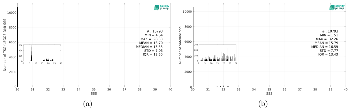
Figure 3: Histograms of SSS from TSG (LEGOS-DM) (a) and SMAP SSS L2 v6 - 40 km (RSS) (b) considering all match-up pairs per bins of 0.1 over the Baltic Sea Pi-MEP region and for the full satellite product period.
