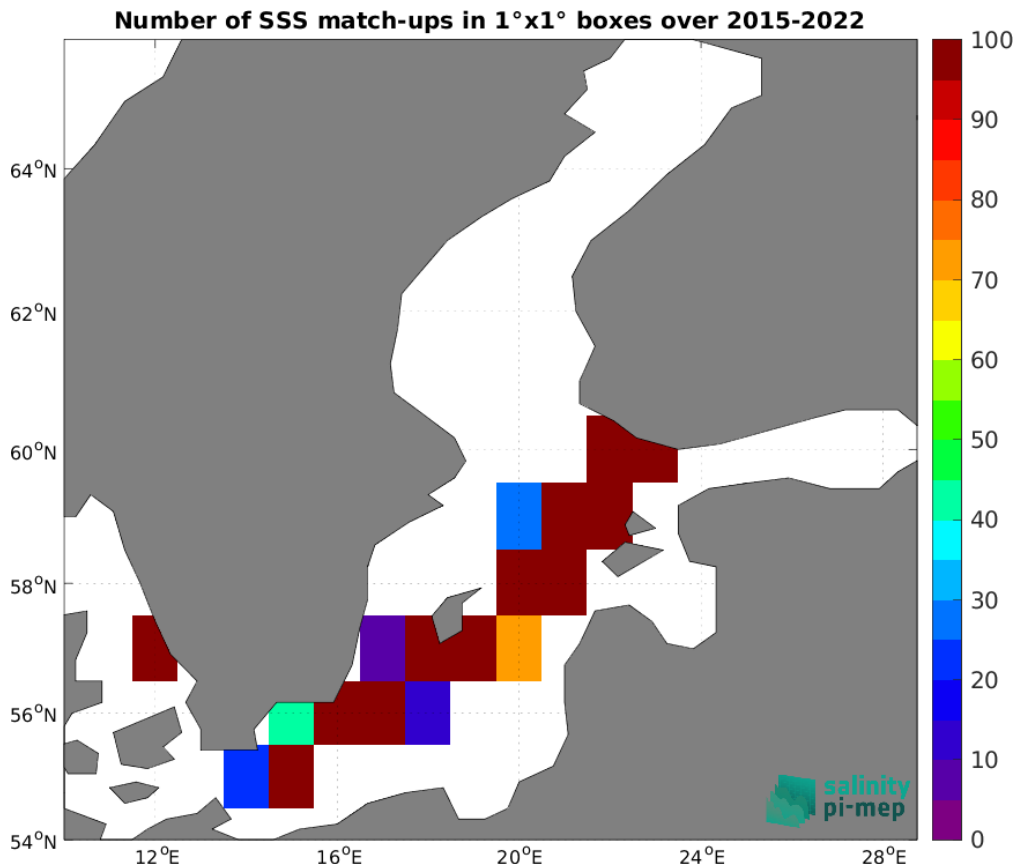
Figure 4: Number of SSS match-ups between TSG (LEGOS-DM) SSS and the SMAP SSS L2 v5 (RSS) SSS product for the Baltic Sea Pi-MEP region over 1^\circ \times 1^\circ boxes and for the full satellite product period.
