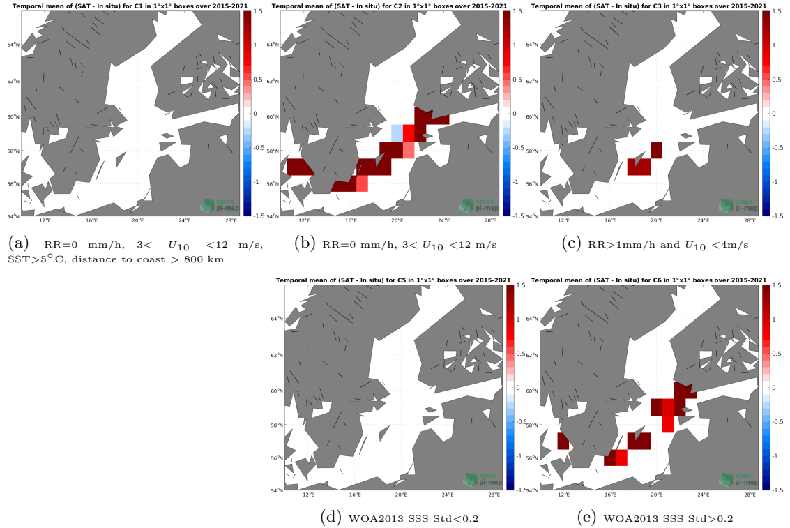
Figure 12: Temporal mean gridded over spatial boxes of size 1^{\circ}\times 1^{\circ} of \Delta\text{SSS} (SMAP SSS L2 v5 (RSS) - TSG (LEGOS-DM)) for 5 different subdatasets corresponding to: \text{RR}=0 mm/h, 3 < U_{10} < 12 m/s, \text{SST} > 5^{\circ}\text{C} , distance to coast > 800 km (a), \text{RR}=0 mm/h, 3 < U_{10} < 12 m/s (b), \text{RR} > 1\text{mm/h} and U_{10} < 4\text{m/s} (c), WOA2013 SSS Std < 0.2 (d), WOA2013 SSS Std > 0.2 (e).
