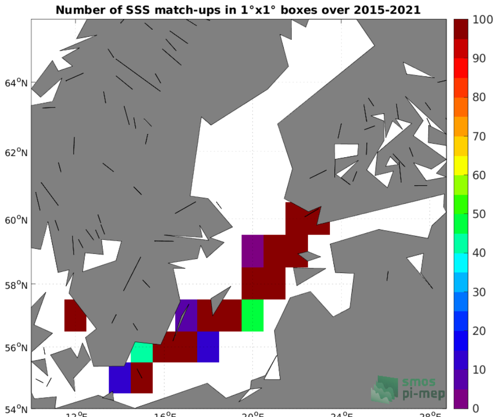
Figure 4: Number of SSS match-ups between TSG (LEGOS-DM) SSS and the SMAP SSS L2 v5 (RSS) SSS product for the Baltic Sea Pi-MEP region over 1°×1° boxes and for the full satellite product period.
