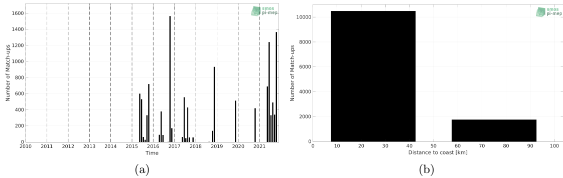
Figure 1: Number of match-ups between TSG (LEGOS-DM) and SMAP SSS L2 v5 (RSS) SSS as a function of time (a) and as function of the distance to coast (b) over the Baltic Sea Pi-MEP region and for the full satellite product period.
