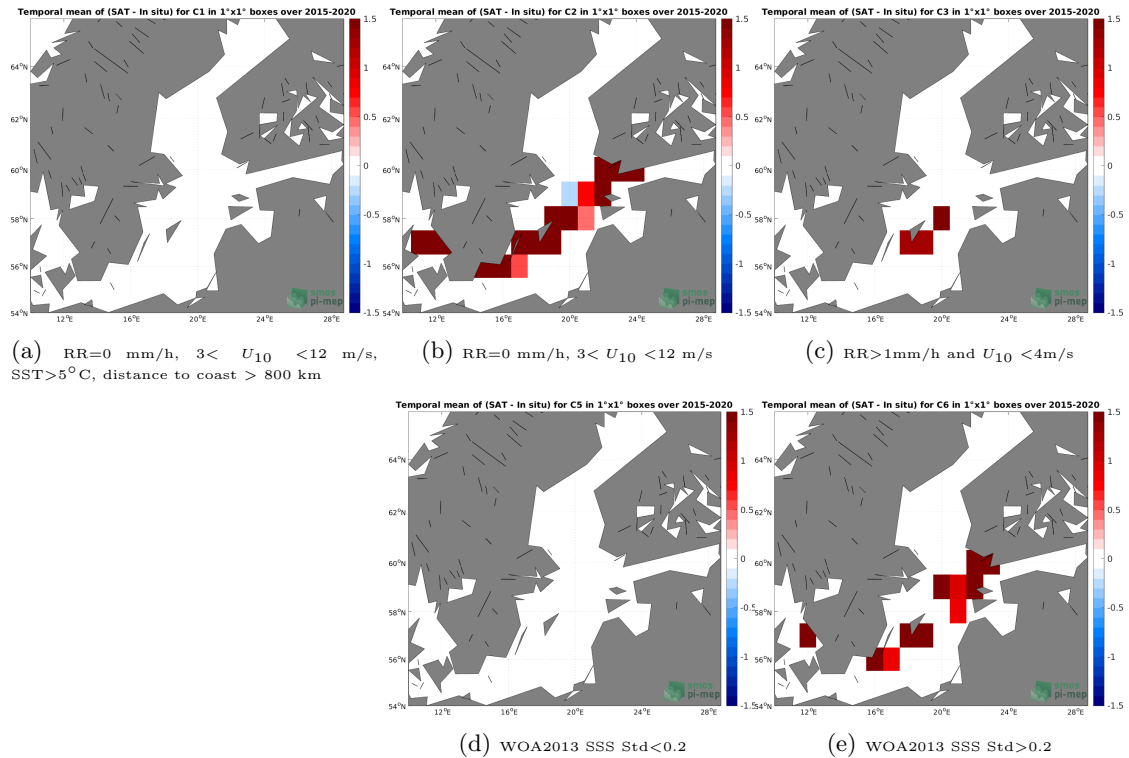
Figure 12: Temporal mean gridded over spatial boxes of size 1^{\circ}\times 1^{\circ} of \Delta\text{SSS} (SMAP SSS L2 v5 (RSS) - TSG (LEGOS-DM)) for 5 different subdatasets corresponding to:RR=0 mm/h, 3 < U_{10} < 12 m/s, SST >5^{\circ}\text{C} , distance to coast > 800 km (a), RR=0 mm/h, 3 < U_{10} < 12 m/s (b), RR >1 mm/h and U_{10} < 4 m/s (c), WOA2013 SSS Std <0.2 (d), WOA2013 SSS Std >0.2 (e).
