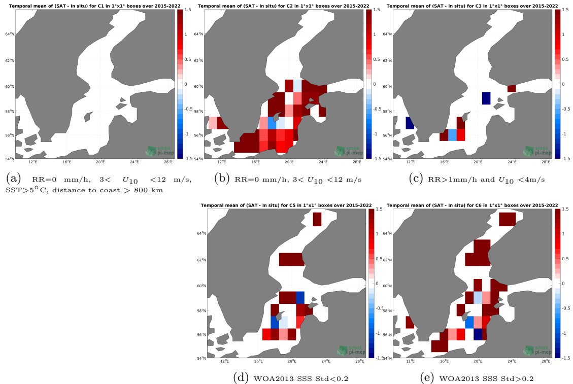
Figure 12: Temporal mean gridded over spatial boxes of size 1^{\circ}\times 1^{\circ} of \Delta\text{SSS} (SMAP SSS L2 v5 (RSS) - ICES) for 5 different subdatasets corresponding to:RR=0 mm/h, 3 < U_{10} < 12 m/s, SST >5^{\circ}\text{C} , distance to coast > 800 km (a), RR=0 mm/h, 3 < U_{10} < 12 m/s (b), RR >1 mm/h and U_{10} < 4 m/s (c), WOA2013 SSS Std <0.2 (d), WOA2013 SSS Std >0.2 (e).
