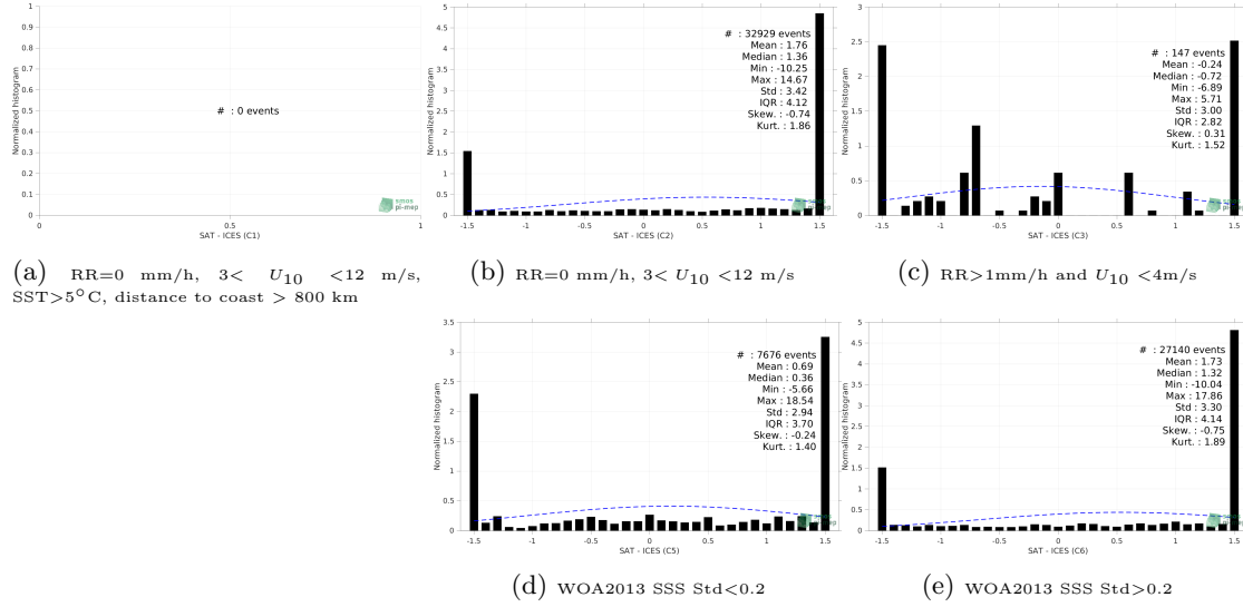
Figure 13: Normalized histogram of \Delta SSS (SMAP SSS L2 v5 (RSS) - ICES) for 5 different subdatasets corresponding to: RR=0 mm/h, 3 < U_{10} < 12 m/s, SST > 5°C, distance to coast > 800 km (a), RR=0 mm/h, 3 < U_{10} < 12 m/s (b), RR > 1mm/h and U_{10} < 4 m/s (c), WOA2013 SSS Std < 0.2 (d), WOA2013 SSS Std > 0.2 (e).
