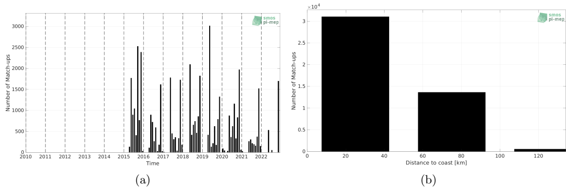
Figure 1: Number of match-ups between ICES and SMAP SSS L2 v5 (RSS) SSS as a function of time (a) and as function of the distance to coast (b) over the Baltic Sea Pi-MEP region and for the full satellite product period.
