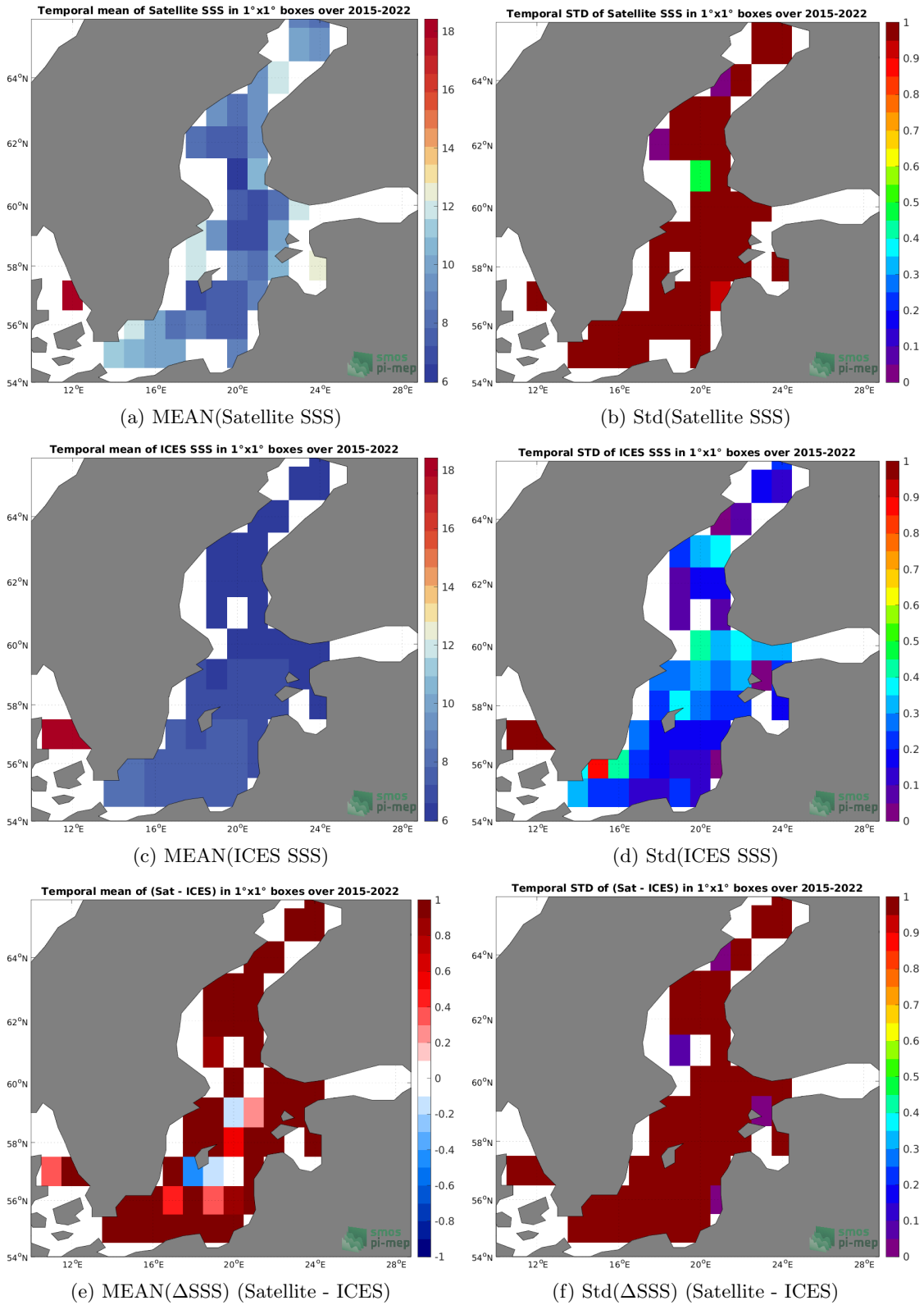
Figure 6: Temporal mean (left) and Std (right) of SSS from SMAP SSS L2 v5 (RSS) (top), ICES (middle), and of \Delta SSS (Satellite - ICES). Only match-up pairs are used to generate these maps.
