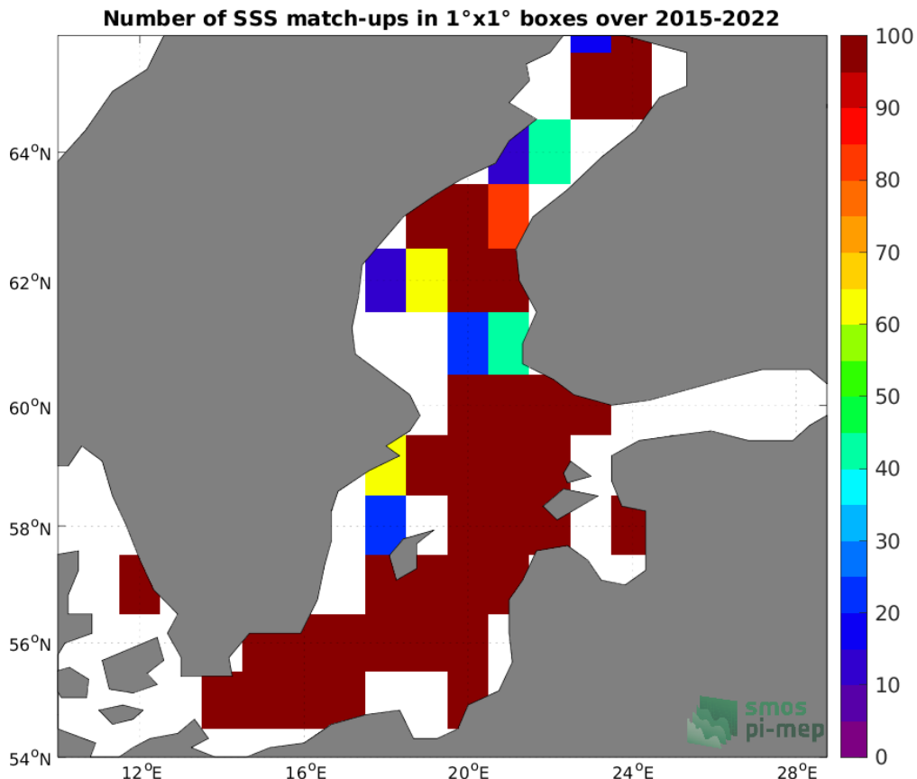
Figure 4: Number of SSS match-ups between ICES SSS and the SMAP SSS L2 v5 (RSS) SSS product for the Baltic Sea Pi-MEP region over 1°x1° boxes and for the full satellite product period.
