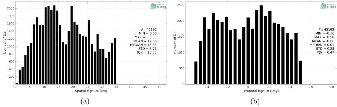
Figure 5: Histograms of the spatial (a) and temporal (b) lags between the location/time of the ICES measurement and the date of the corresponding SMAP SSS L2 v5 (RSS) SSS pixel.
