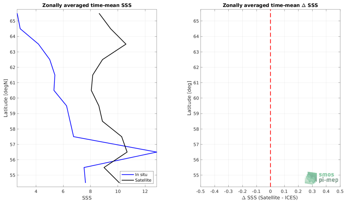
Figure 8: Left panel: Zonal mean SSS from SMAP SSS L2 v5 (RSS) satellite product (black) and from ICES (blue). Right panel: Zonal mean of \Delta SSS (Satellite - ICES) for all the collected Pi-MEP match-up pairs estimated over the full satellite product period.
