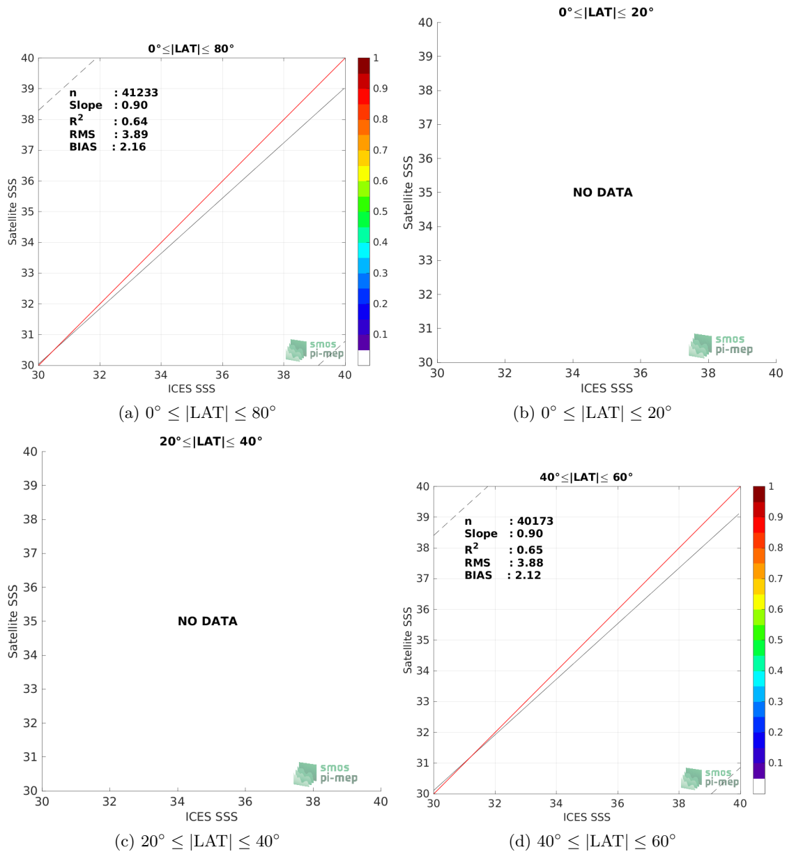
Figure 9: Contour maps of the concentration of SMAP SSS L2 v5 (RSS) SSS (y-axis) versus ICES SSS (x-axis) at match-up pairs for different latitude bands. For each plot, the red line shows x=y . The black thin and dashed lines indicate a linear fit through the data cloud and the \pm 95\% confidence levels, respectively. The number match-up pairs n , the slope and R^2 coefficient of the linear fit, the root mean square (RMS) and the mean bias between satellite and in situ data are indicated for each latitude band in each plots.
