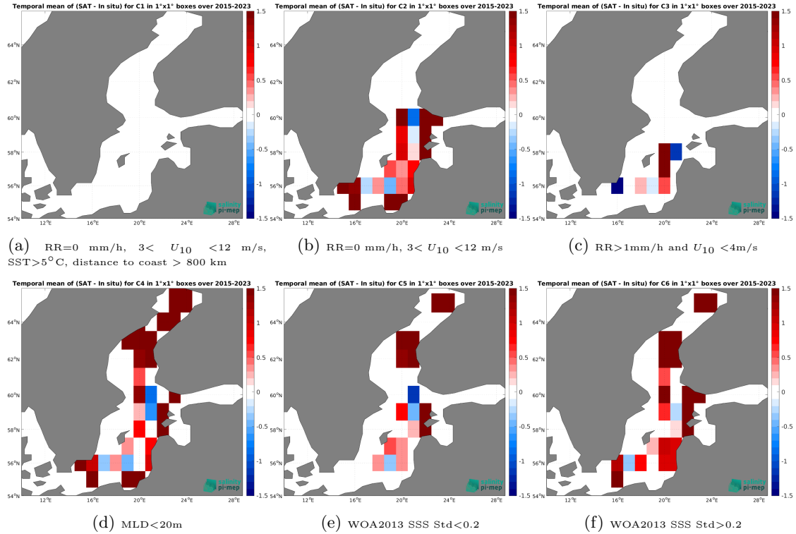
Figure 12: Temporal mean gridded over spatial boxes of size 1^{\circ}\times 1^{\circ} of \Delta\text{SSS} (SMAP SSS L2 v5 (RSS) - Argo) for 6 different subdatasets corresponding to: \text{RR}=0 mm/h, 3 < U_{10} < 12 m/s, \text{SST} > 5^{\circ}\text{C} , distance to coast > 800 km (a), \text{RR}=0 mm/h, 3 < U_{10} < 12 m/s (b), \text{RR} > 1\text{mm/h} and U_{10} < 4\text{m/s} (c), \text{MLD} < 20\text{m} (d), \text{WOA2013 SSS Std} < 0.2 (e), \text{WOA2013 SSS Std} > 0.2 (f).
