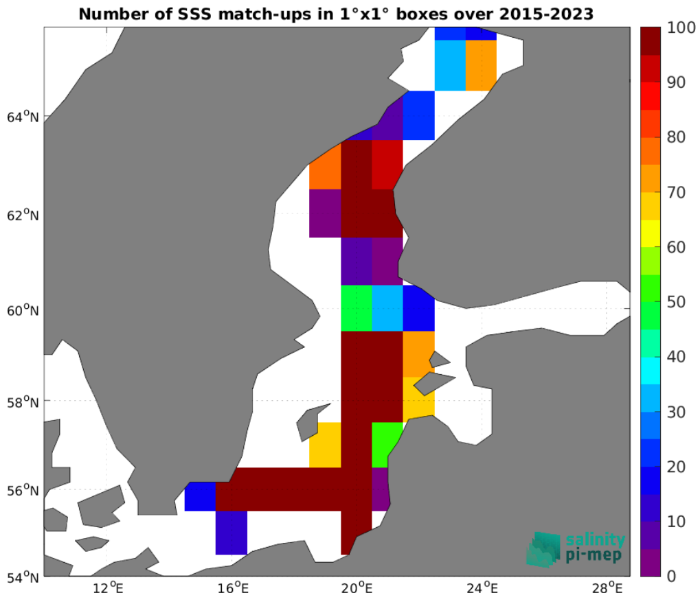
Figure 4: Number of SSS match-ups between Argo SSS and the SMAP SSS L2 v5 (RSS) SSS product for the Baltic Sea Pi-MEP region over 1^\circ \times 1^\circ boxes and for the full satellite product period.
