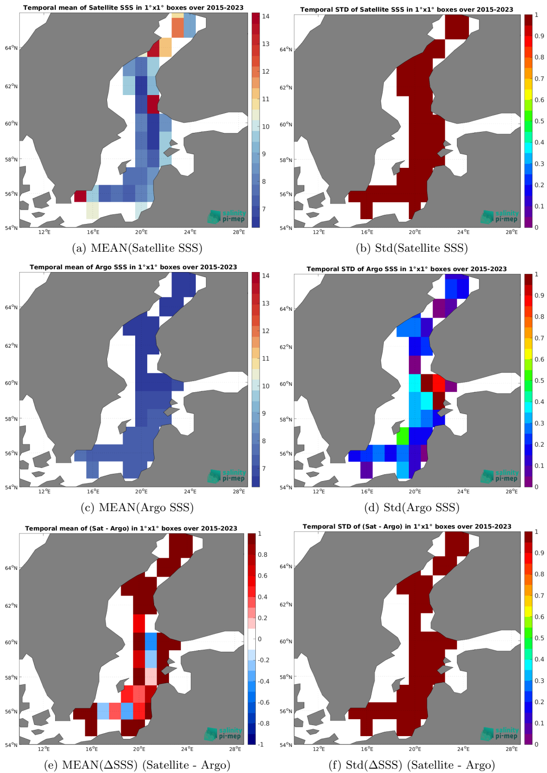
Figure 6: Temporal mean (left) and Std (right) of SSS from SMAP SSS L2 v5 (RSS) (top), Argo (middle), and of \Delta SSS (Satellite - Argo). Only 16 match-up pairs are used to generate these maps.
