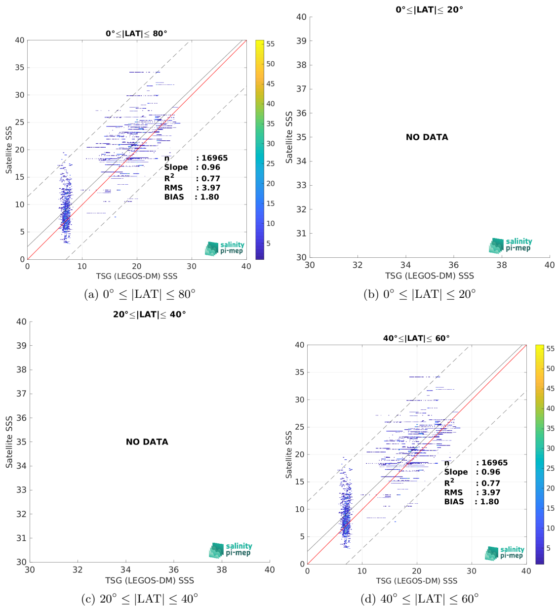
Figure 10: Contour maps of the concentration of SMAP SSS L2 v5.3 (RSS) SSS (y-axis) versus TSG (LEGOS-DM) SSS (x-axis) at match-up pairs for different latitude bands. For each plot, the red line shows x=y . The black thin and dashed lines indicate a linear fit through the data cloud and the \pm 95\% confidence levels, respectively. The number match-up pairs n , the slope and R^2 coefficient of the linear fit, the root mean square (RMS) and the mean bias between satellite and in situ data are indicated for each latitude band in each plot.
