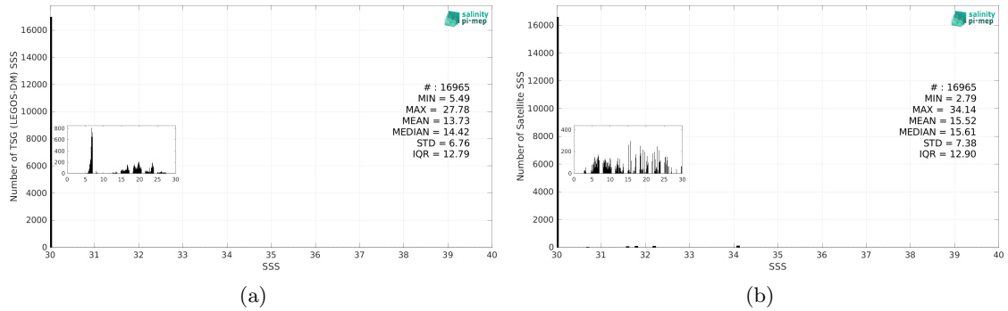
Figure 3: Histograms of SSS from TSG (LEGOS-DM) (a) and SMAP SSS L2 v5.3 (RSS) (b) considering all match-up pairs per bins of 0.1 over the Baltic Sea Pi-MEP region and for the full satellite product period.
