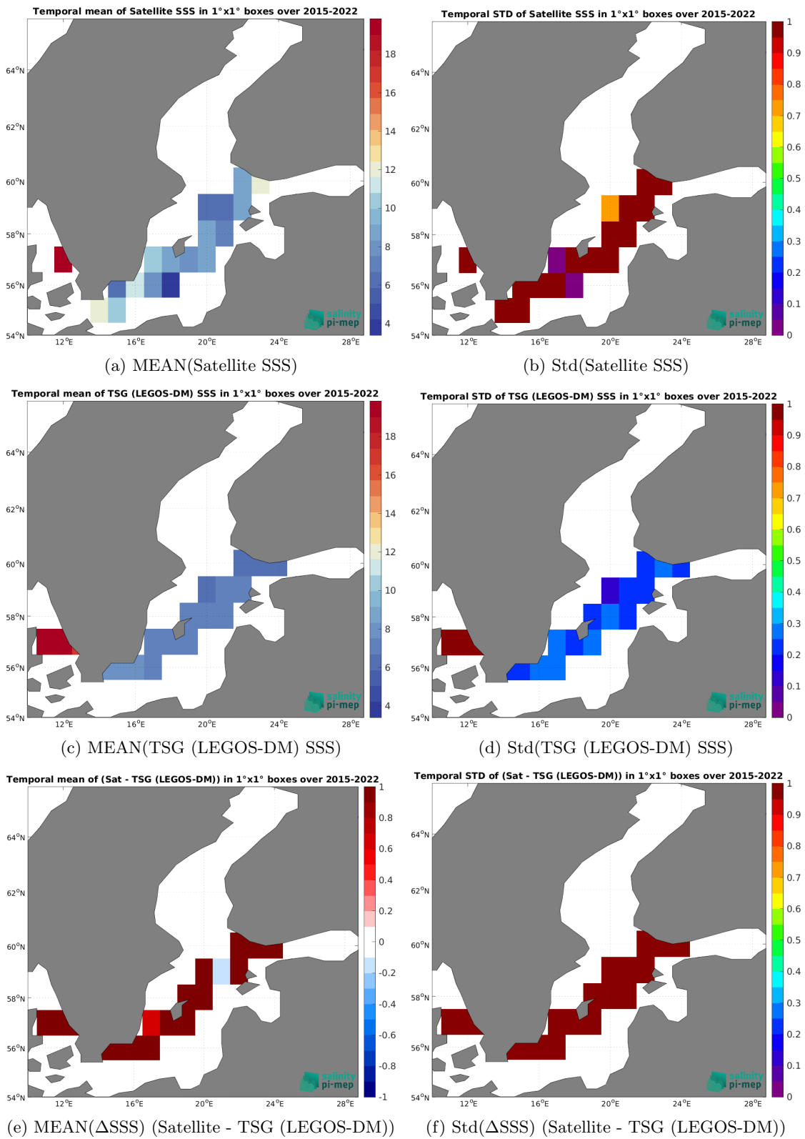
Figure 7: Temporal mean (left) and Std (right) of SSS from SMAP SSS L2 v5.3 (RSS) (top), TSG (LEGOS-DM) (middle), and of \Delta SSS (Satellite - TSG (LEGOS-DM)). Only match-up pairs are used to generate these maps.
