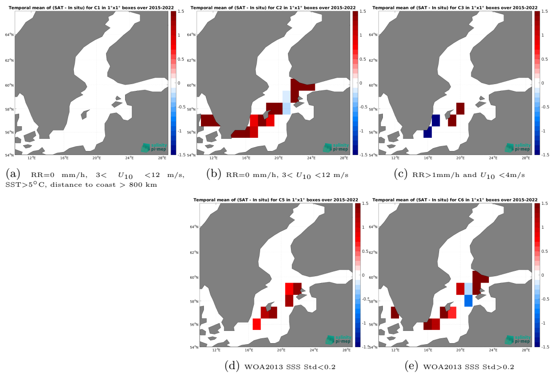
Figure 14: Temporal mean gridded over spatial boxes of size 1^\circ \times 1^\circ of \Delta SSS (SMAP SSS L2 v5.3 (RSS) - TSG (LEGOS-DM)) for 5 different subdatasets corresponding to:RR=0 mm/h, 3 < U_{10} < 12 m/s, SST >5^\circ\text{C} , distance to coast > 800 km (a), RR=0 mm/h, 3 < U_{10} < 12 m/s (b), RR >1 mm/h and U_{10} < 4 m/s (c), WOA2013 SSS Std <0.2 (d), WOA2013 SSS Std >0.2 (e).
