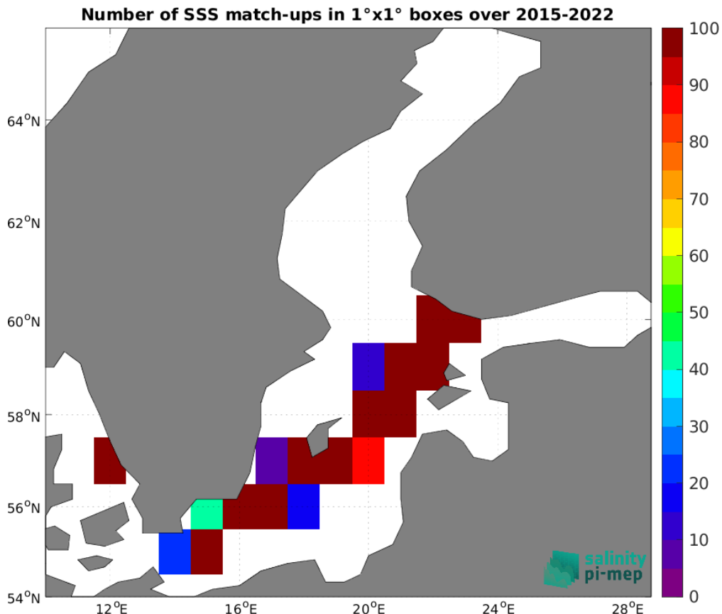
Figure 5: Number of SSS match-ups between TSG (LEGOS-DM) SSS and the SMAP SSS L2 v5.3 (RSS) SSS product for the Baltic Sea Pi-MEP region over 1^\circ \times 1^\circ boxes and for the full satellite product period.
