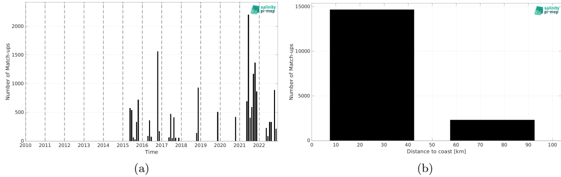
Figure 2: Number of match-ups between TSG (LEGOS-DM) and SMAP SSS L2 v5.3 (RSS) SSS as a function of time (a) and as function of the distance to coast (b) over the Baltic Sea Pi-MEP region and for the full satellite product period.
