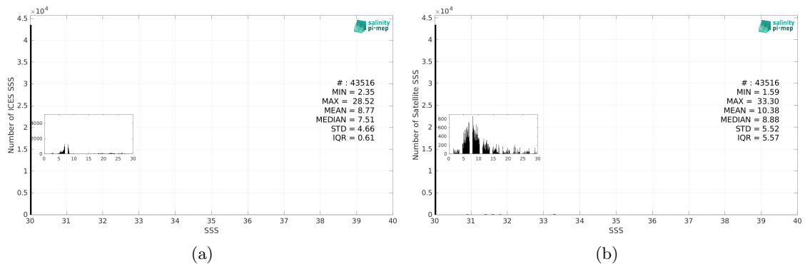
Figure 3: Histograms of SSS from ICES (a) and SMAP SSS L2 v5.3 (RSS) (b) considering all match-up pairs per bins of 0.1 over the Baltic Sea Pi-MEP region and for the full satellite product period.
