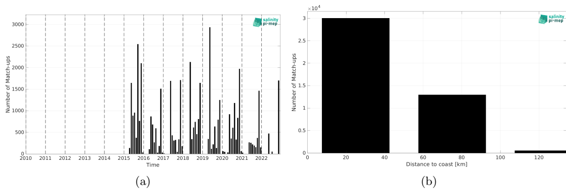
Figure 2: Number of match-ups between ICES and SMAP SSS L2 v5.3 (RSS) SSS as a function of time (a) and as function of the distance to coast (b) over the Baltic Sea Pi-MEP region and for the full satellite product period.
