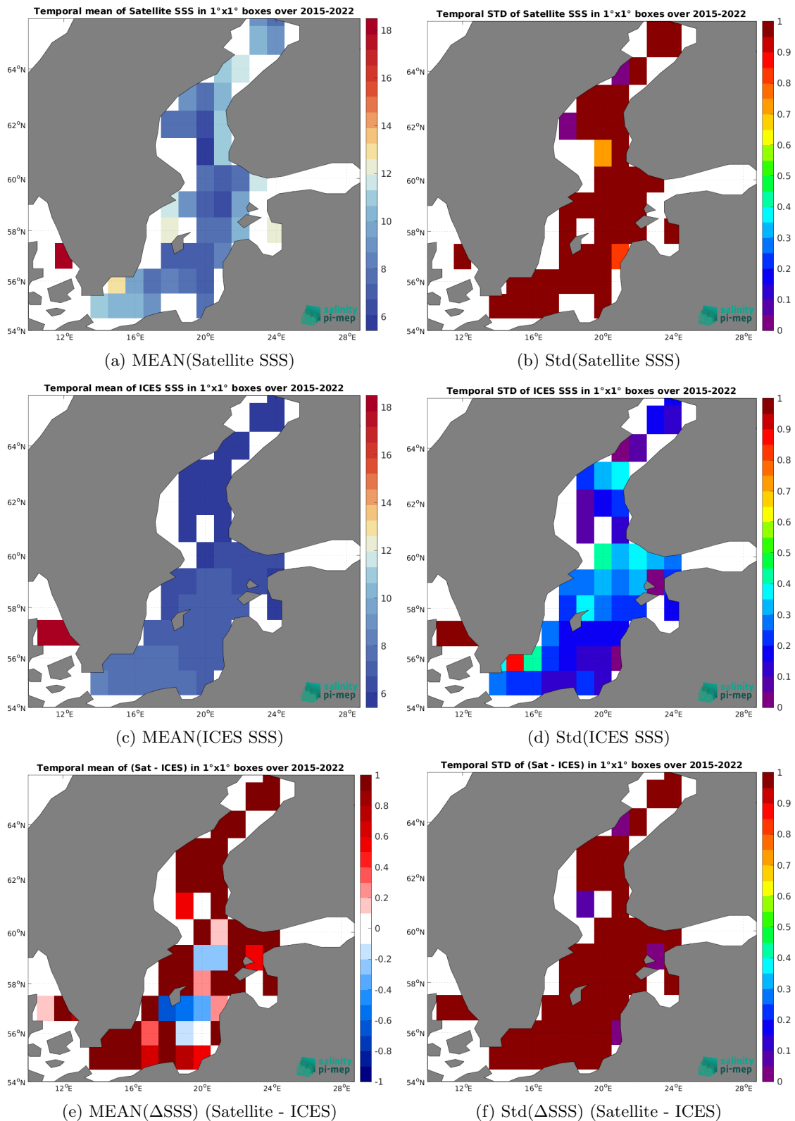
Figure 7: Temporal mean (left) and Std (right) of SSS from SMAP SSS L2 v5.3 (RSS) (top), ICES (middle), and of \Delta SSS (Satellite - ICES) (bottom). Only match-up pairs are used to generate these maps.
