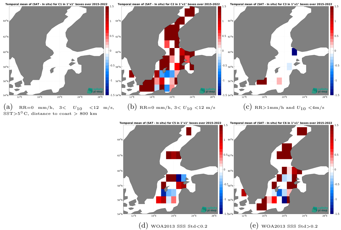
Figure 14: Temporal mean gridded over spatial boxes of size 1^\circ \times 1^\circ of \Delta SSS (SMAP SSS L2 v5.3 (RSS) - ICES) for 5 different subdatasets corresponding to:RR=0 mm/h, 3 < U_{10} < 12 m/s, SST>5°C, distance to coast > 800 km (a), RR=0 mm/h, 3 < U_{10} < 12 m/s (b), RR>1mm/h and U_{10} < 4 m/s (c), WOA2013 SSS Std<0.2 (d), WOA2013 SSS Std>0.2 (e).
