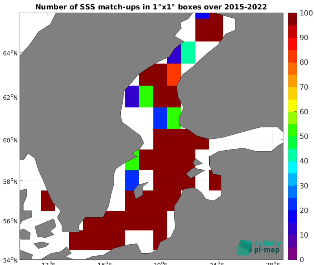
Figure 5: Number of SSS match-ups between ICES SSS and the SMAP SSS L2 v5.3 (RSS) SSS product for the Baltic Sea Pi-MEP region over 1°x1° boxes and for the full satellite product period.
