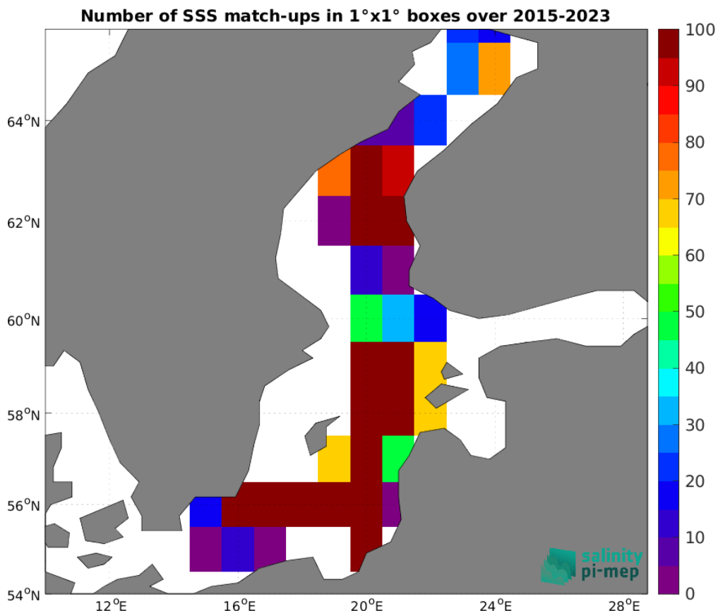
Figure 5: Number of SSS match-ups between Argo SSS and the SMAP SSS L2 v5.3 (RSS) SSS product for the Baltic Sea Pi-MEP region over 1^\circ \times 1^\circ boxes and for the full satellite product period.
