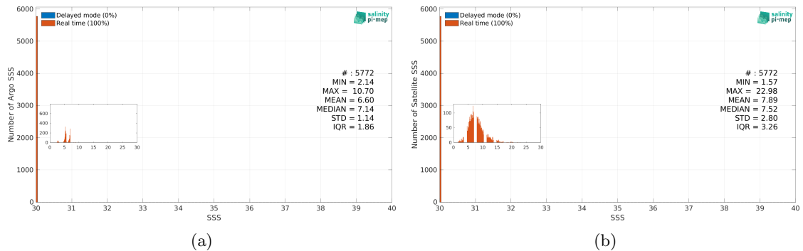
Figure 3: Histograms of SSS from Argo (a) and SMAP SSS L2 v5.3 (RSS) (b) considering all match-up pairs per bins of 0.1 over the Baltic Sea Pi-MEP region and for the full satellite product period.
