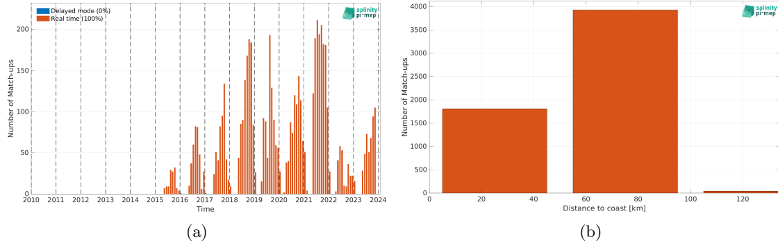
Figure 2: Number of match-ups between Argo and SMAP SSS L2 v5.3 (RSS) SSS as a function of time (a) and as function of the distance to coast (b) over the Baltic Sea Pi-MEP region and for the full satellite product period.
