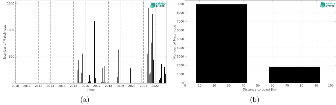
Figure 2: Number of match-ups between TSG (LEGOS-DM) and SMAP SSS L2 v5.3 - 40 km (RSS) SSS as a function of time (a) and as function of the distance to coast (b) over the Baltic Sea Pi-MEP region and for the full satellite product period.
