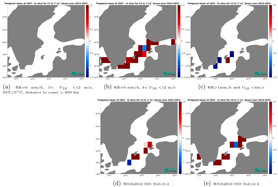
Figure 14: Temporal mean gridded over spatial boxes of size 1^\circ \times 1^\circ of \Delta\text{SSS} (SMAP SSS L2 v5.3 - 40 km (RSS) - TSG (LEGOS-DM)) for 5 different subdatasets corresponding to:RR=0 mm/h, 3 < U_{10} < 12 m/s, SST>5°C, distance to coast > 800 km (a), RR=0 mm/h, 3 < U_{10} < 12 m/s (b), RR>1mm/h and U_{10} < 4 m/s (c), WOA2013 SSS Std<0.2 (d), WOA2013 SSS Std>0.2 (e).
