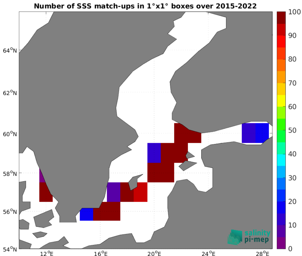
Figure 5: Number of SSS match-ups between TSG (LEGOS-DM) SSS and the SMAP SSS L2 v5.3 - 40 km (RSS) SSS product for the Baltic Sea Pi-MEP region over 1^\circ \times 1^\circ boxes and for the full satellite product period.
