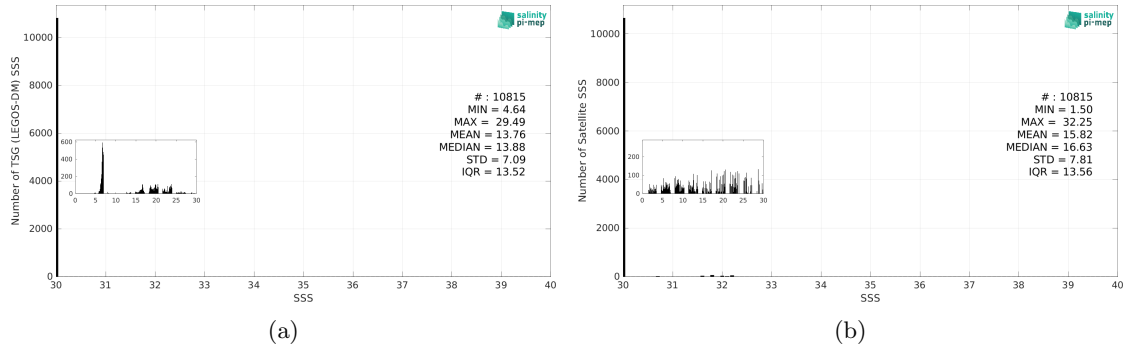
Figure 3: Histograms of SSS from TSG (LEGOS-DM) (a) and SMAP SSS L2 v5.3 - 40 km (RSS) (b) considering all match-up pairs per bins of 0.1 over the Baltic Sea Pi-MEP region and for the full satellite product period.
