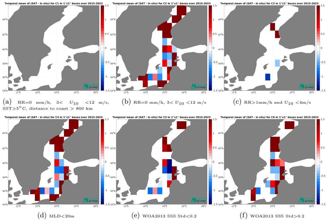
Figure 14: Temporal mean gridded over spatial boxes of size 1^\circ \times 1^\circ of \Delta SSS (SMAP SSS L2 v5.3 - 40 km (RSS) - Argo) for 6 different subdatasets corresponding to:RR=0 mm/h, 3 < U_{10} < 12 m/s, SST>5°C, distance to coast > 800 km (a), RR=0 mm/h, 3 < U_{10} < 12 m/s (b), RR>1mm/h and U_{10} < 4 m/s (c),MLD<20m (d),WOA2013 SSS Std<0.2 (e),WOA2013 SSS Std>0.2 (f).
