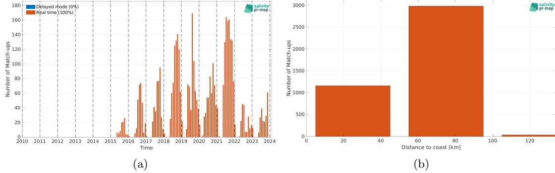
Figure 2: Number of match-ups between Argo and SMAP SSS L2 v5.3 - 40 km (RSS) SSS as a function of time (a) and as function of the distance to coast (b) over the Baltic Sea Pi-MEP region and for the full satellite product period.
