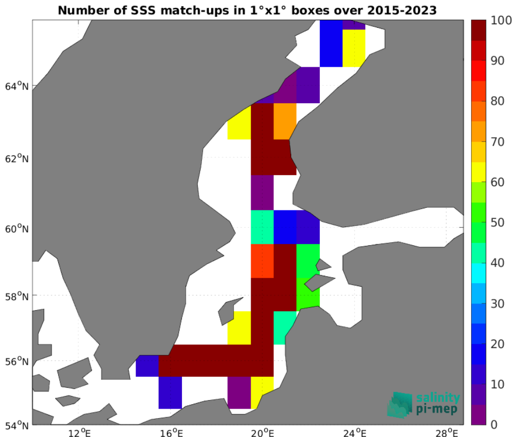
Figure 5: Number of SSS match-ups between Argo SSS and the SMAP SSS L2 v5.3 - 40 km (RSS) SSS product for the Baltic Sea Pi-MEP region over 1^\circ \times 1^\circ boxes and for the full satellite product period.
