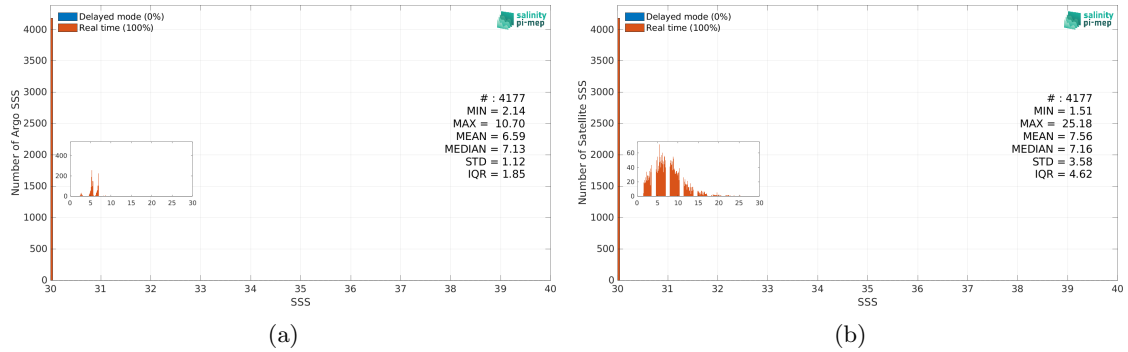
Figure 3: Histograms of SSS from Argo (a) and SMAP SSS L2 v5.3 - 40 km (RSS) (b) considering all match-up pairs per bins of 0.1 over the Baltic Sea Pi-MEP region and for the full satellite product period.
