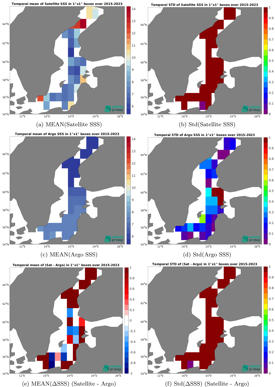
Figure 7: Temporal mean (left) and Std (right) of SSS from SMAP SSS L2 v5.3 - 40 km (RSS) (top), Argo (middle), and of \Delta SSS (Satellite - Argo). Only match-up pairs are used to generate these maps.
