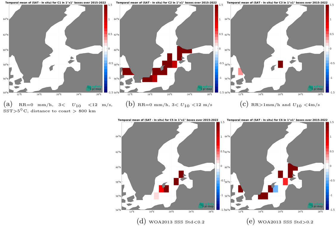
Figure 12: Temporal mean gridded over spatial boxes of size 1^{\circ}\times 1^{\circ} of \Delta\text{SSS} (SMAP SSS L2 v5 - 40 km (RSS) - TSG (LEGOS-DM)) for 5 different subdatasets corresponding to:RR=0 mm/h, 3 < U_{10} < 12 m/s, SST >5^{\circ}\text{C} , distance to coast > 800 km (a), RR=0 mm/h, 3 < U_{10} < 12 m/s (b), RR >1 mm/h and U_{10} < 4 m/s (c), WOA2013 SSS Std <0.2 (d), WOA2013 SSS Std >0.2 (e).
