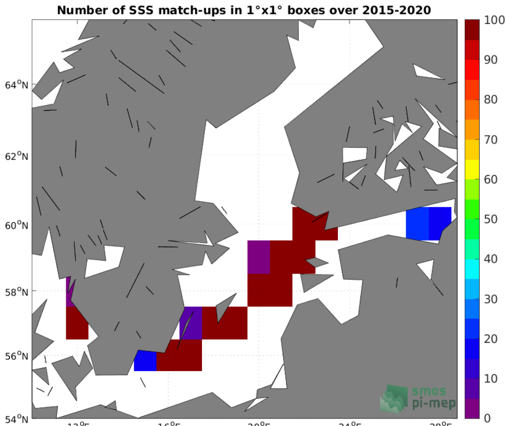
Figure 4: Number of SSS match-ups between TSG (LEGOS-DM) SSS and the SMAP SSS L2 v5 - 40 km (RSS) SSS product for the Baltic Sea Pi-MEP region over 1°×1° boxes and for the full satellite product period.
