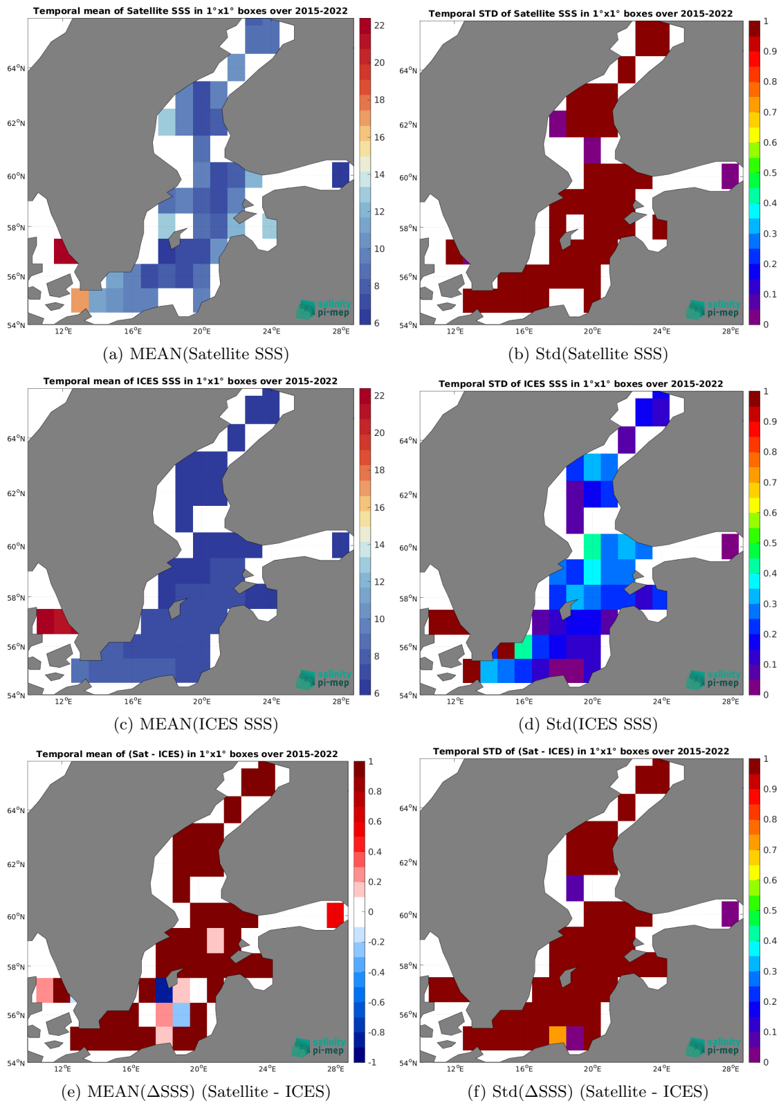
Figure 6: Temporal mean (left) and Std (right) of SSS from SMAP SSS L2 v5 - 40 km (RSS) (top), ICES (middle), and of \Delta SSS (Satellite - ICES). Only match-up pairs are used to generate these maps.
