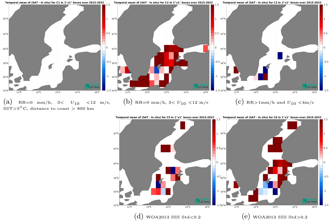
Figure 12: Temporal mean gridded over spatial boxes of size 1^{\circ}\times 1^{\circ} of \Delta\text{SSS} (SMAP SSS L2 v5 - 40 km (RSS) - ICES) for 5 different subdatasets corresponding to:RR=0 mm/h, 3 < U_{10} < 12 m/s, SST > 5^{\circ}\text{C} , distance to coast > 800 km (a), RR=0 mm/h, 3 < U_{10} < 12 m/s (b), RR > 1 mm/h and U_{10} < 4 m/s (c), WOA2013 SSS Std < 0.2 (d), WOA2013 SSS Std > 0.2 (e).
