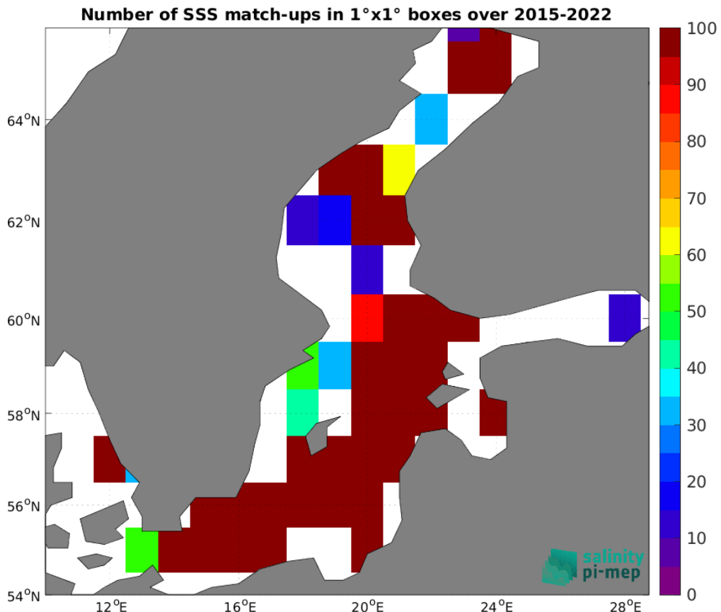
Figure 4: Number of SSS match-ups between ICES SSS and the SMAP SSS L2 v5 - 40 km (RSS) SSS product for the Baltic Sea Pi-MEP region over 1^\circ \times 1^\circ boxes and for the full satellite product period.
