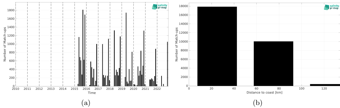
Figure 1: Number of match-ups between ICES and SMAP SSS L2 v5 - 40 km (RSS) SSS as a function of time (a) and as function of the distance to coast (b) over the Baltic Sea Pi-MEP region and for the full satellite product period.
