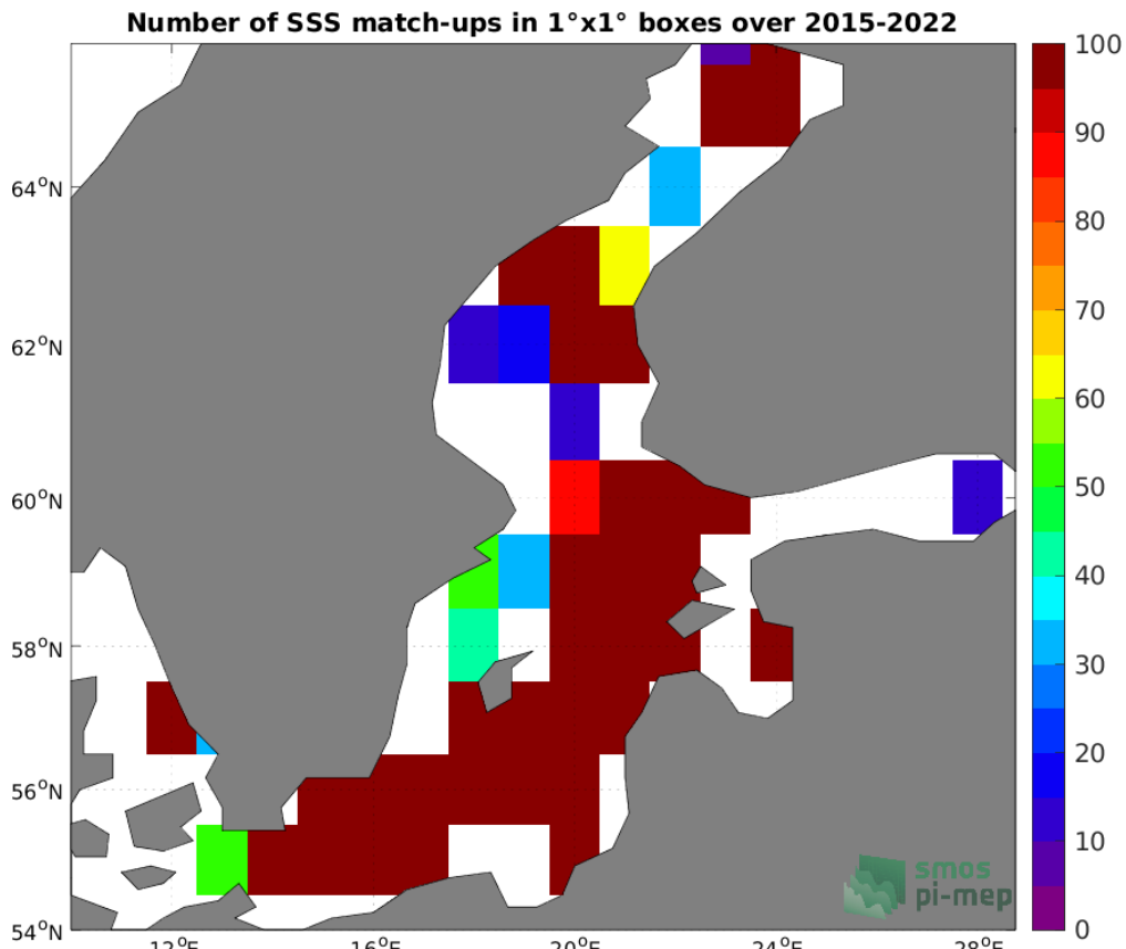
Figure 4: Number of SSS match-ups between ICES SSS and the SMAP SSS L2 v5 - 40 km (RSS) SSS product for the Baltic Sea Pi-MEP region over 1°×1° boxes and for the full satellite product period.
