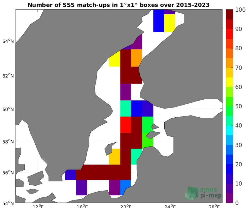
Figure 4: Number of SSS match-ups between Argo SSS and the SMAP SSS L2 v5 - 40 km (RSS) SSS product for the Baltic Sea Pi-MEP region over 1°×1° boxes and for the full satellite product period.
