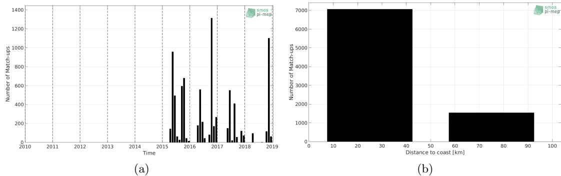
Figure 1: Number of match-ups between TSG (LEGOS-DM) and SMAP SSS L2 v4 (RSS) SSS as a function of time (a) and as function of the distance to coast (b) over the Baltic Sea Pi-MEP region and for the full satellite product period.
