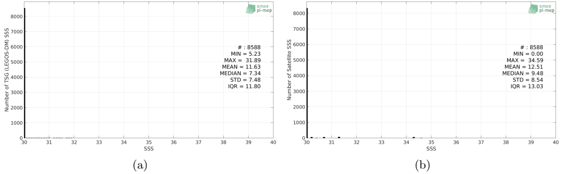
Figure 2: Histograms of SSS from TSG (LEGOS-DM) (a) and SMAP SSS L2 v4 (RSS) (b) considering all match-up pairs per bins of 0.1 over the Baltic Sea Pi-MEP region and for the full satellite product period.
