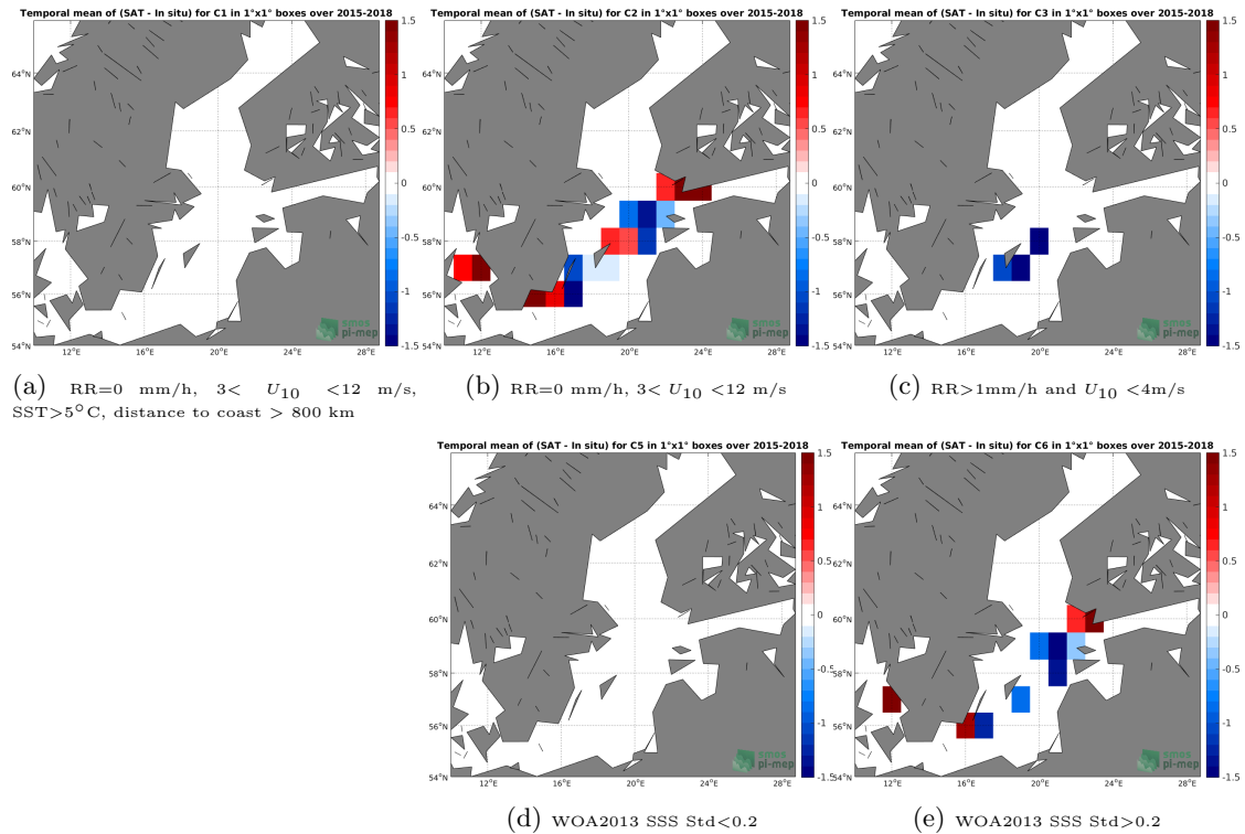
Figure 12: Temporal mean gridded over spatial boxes of size 1^{\circ}\times 1^{\circ} of \Delta\text{SSS} (SMAP SSS L2 v4 (RSS) - TSG (LEGOS-DM)) for 5 different subdatasets corresponding to:RR=0 mm/h, 3 < U_{10} < 12 m/s, SST >5^{\circ}\text{C} , distance to coast > 800 km (a), RR=0 mm/h, 3 < U_{10} < 12 m/s (b), RR >1 mm/h and U_{10} < 4 m/s (c), WOA2013 SSS Std <0.2 (d), WOA2013 SSS Std >0.2 (e).
