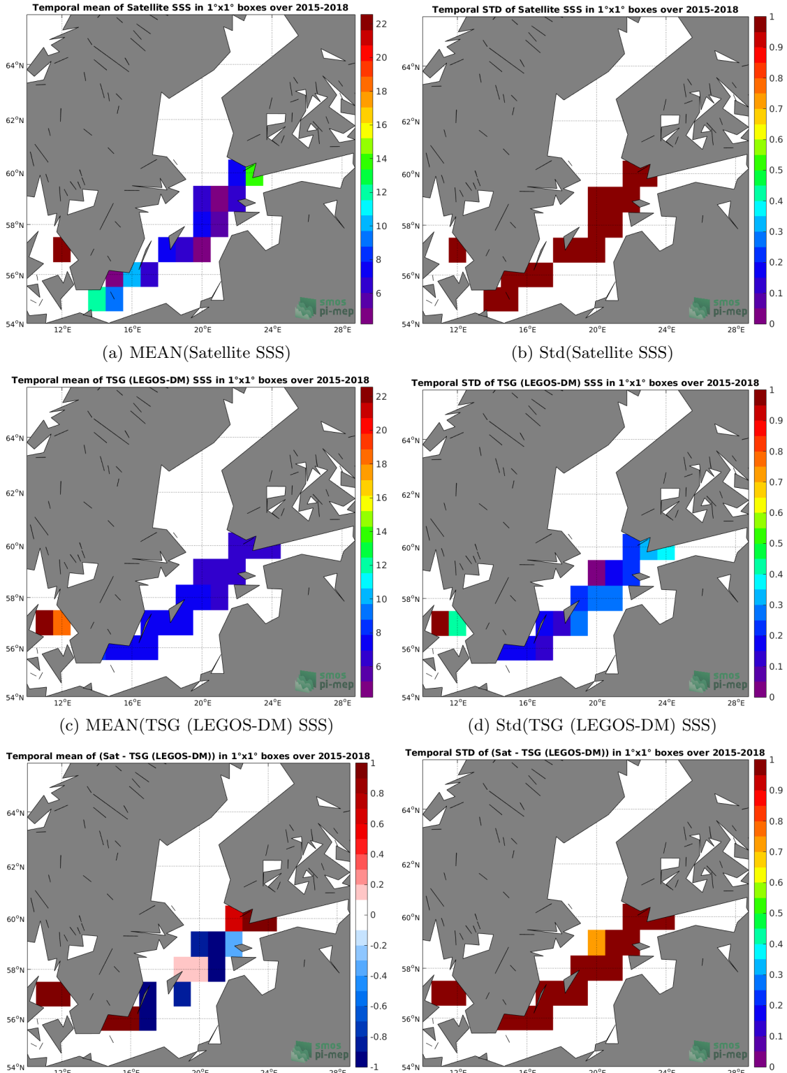
(a) MEAN(Satellite SSS) (b) Std(Satellite SSS) (c) MEAN(TSG (LEGOS-DM) SSS) (d) Std(TSG (LEGOS-DM) SSS) (e) MEAN( \Delta SSS) (Satellite - TSG (LEGOS-DM)) (f) Std( \Delta SSS) (Satellite - TSG (LEGOS-DM)) Figure 6: Temporal mean (left) and Std (right) of SSS from SMAP SSS L2 v4 (RSS) (top), TSG (LEGOS-DM) (middle), and of \Delta SSS (Satellite 22 - TSG (LEGOS-DM)). Only match-up pairs are used to generate these maps.
