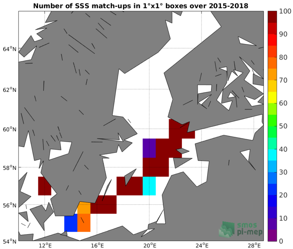
Figure 4: Number of SSS match-ups between TSG (LEGOS-DM) SSS and the SMAP SSS L2 v4 (RSS) SSS product for the Baltic Sea Pi-MEP region over 1°x1° boxes and for the full satellite product period.
