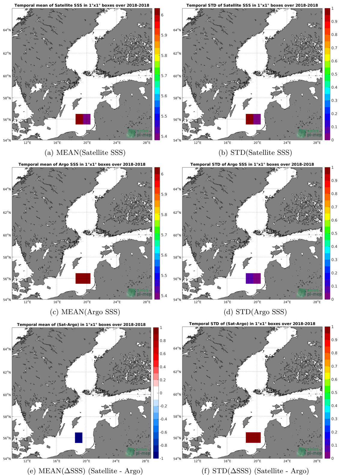
Figure 6: Temporal mean (left) and STD (right) of SSS from SMAP-L2-RSS-V3-70KM (top), Argo (middle), and of \Delta SSS (Satellite - Argo). Only match-up pairs are used to generate these maps.
