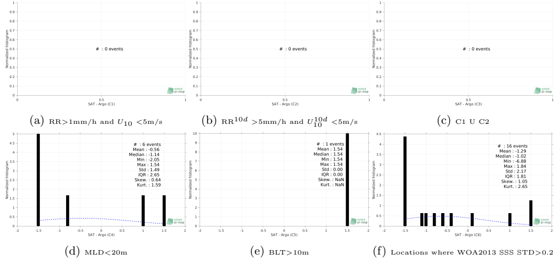
Figure 13: Normalized histogram of \Delta SSS (SMAP-L2-RSS-V3-70KM - Argo) for 6 different sub-datasets corresponding to: RR>1mm/h and U_{10} < 5 m/s (a), RR^{10d} > 5 mm/h and U_{10}^{10d} < 5 m/s (b), C1 U C2 (c),MLD<20m (d),BLT>10m (e),Locations where WOA2013 SSS STD>0.2 (f).
