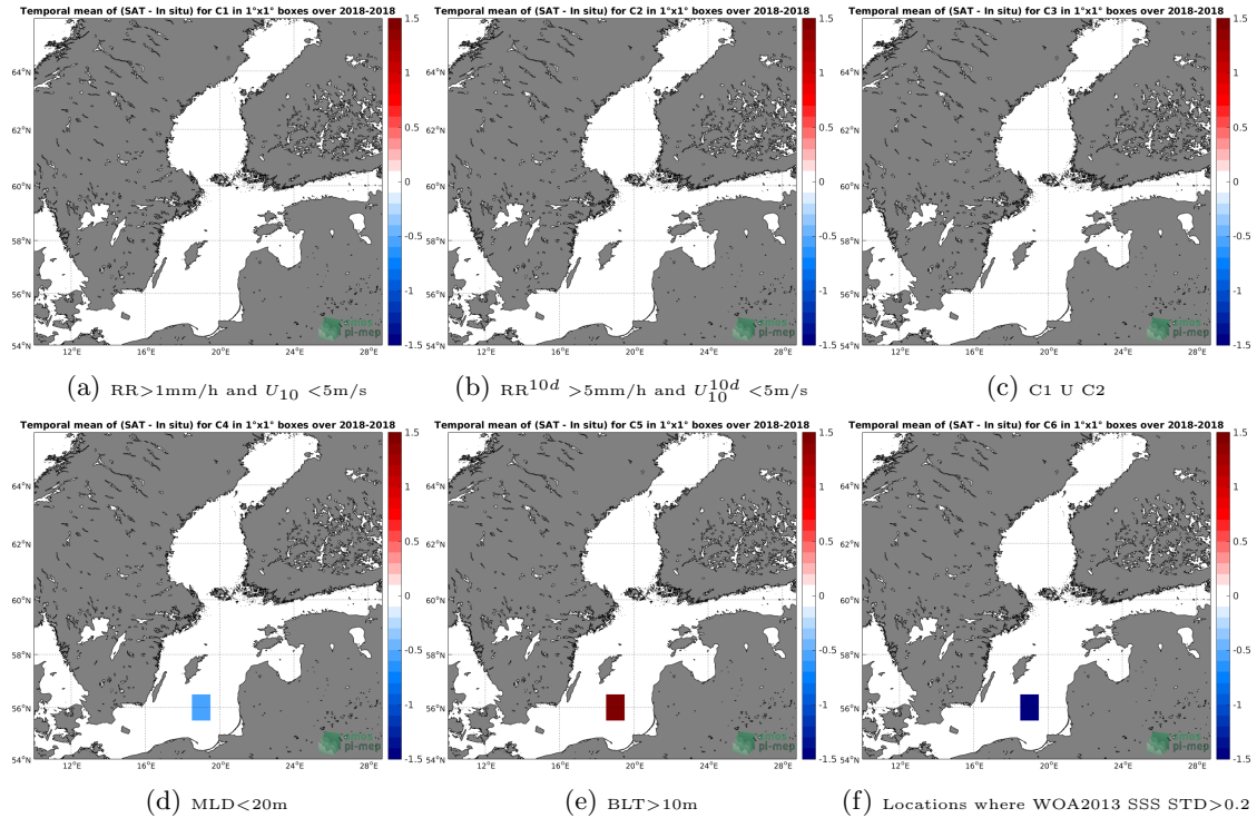
Figure 12: Temporal mean gridded over spatial boxes of size 1^\circ \times 1^\circ of \Delta\text{SSS} (SMAP-L2-RSS-V3-70KM - Argo) for 6 different subdatasets corresponding to: RR > 1\text{mm/h} and U_{10} < 5\text{m/s} (a), \text{RR}^{10d} > 5\text{mm/h} and U_{10}^{10d} < 5\text{m/s} (b), C1 U C2 (c), \text{MLD} < 20\text{m} (d), \text{BLT} > 10\text{m} (e), Locations where WOA2013 SSS STD > 0.2 (f).
