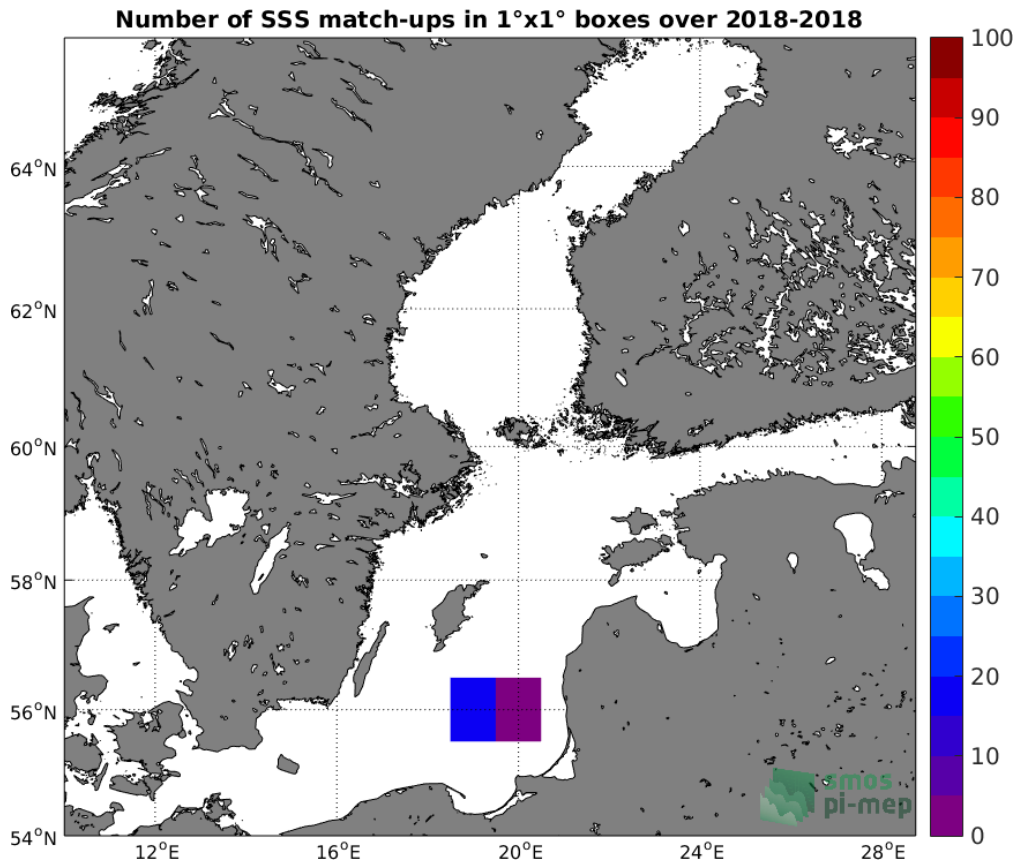
Figure 4: Number of SSS match-ups between Argo SSS and the SMAP-L2-RSS-V3-70KM SSS product for the Baltic Sea Pi-MEP region over 1°x1° boxes and for the full satellite product period.
