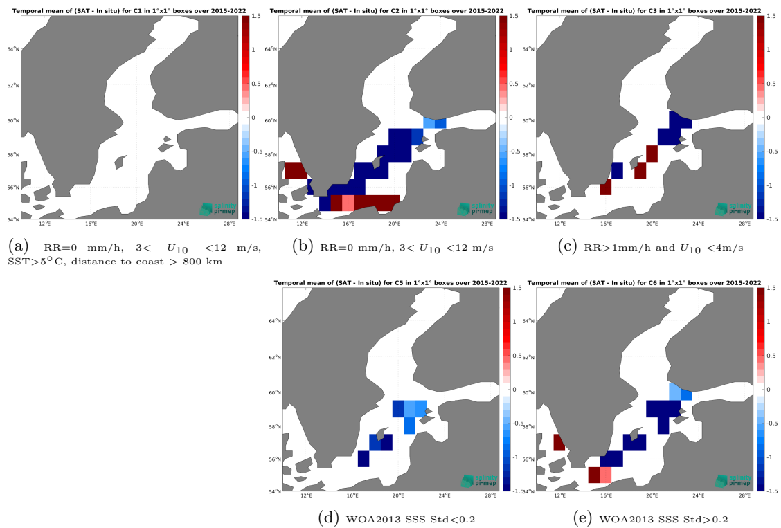
Figure 14: Temporal mean gridded over spatial boxes of size 1^\circ \times 1^\circ of \Delta\text{SSS} (SMAP SSS L2 v5.0 (JPL) - TSG (LEGOS-DM)) for 5 different subdatasets corresponding to:RR=0 mm/h, 3 < U_{10} < 12 m/s, SST >5^\circ\text{C} , distance to coast > 800 km (a), RR=0 mm/h, 3 < U_{10} < 12 m/s (b), RR >1 mm/h and U_{10} < 4 m/s (c), WOA2013 SSS Std <0.2 (d), WOA2013 SSS Std >0.2 (e).
