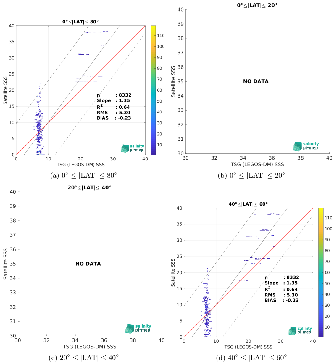
Figure 10: Contour maps of the concentration of SMAP SSS L2 v5.0 (JPL) SSS (y-axis) versus TSG (LEGOS-DM) SSS (x-axis) at match-up pairs for different latitude bands. For each plot, the red line shows x=y . The black thin and dashed lines indicate a linear fit through the data cloud and the \pm 95\% confidence levels, respectively. The number match-up pairs n , the slope and R^2 coefficient of the linear fit, the root mean square (RMS) and the mean bias between satellite and in situ data are indicated for each latitude band in each plot.
