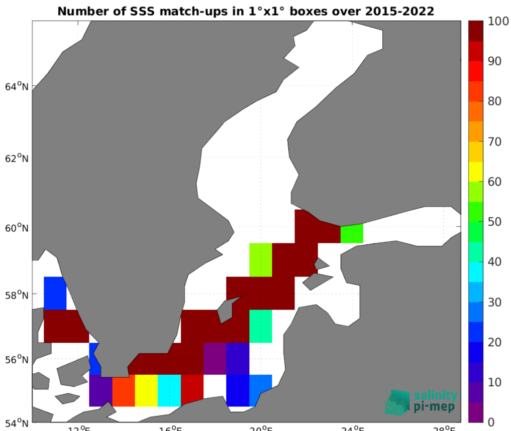
Figure 5: Number of SSS match-ups between TSG (LEGOS-DM) SSS and the SMAP SSS L2 v5.0 (JPL) SSS product for the Baltic Sea Pi-MEP region over 1^\circ \times 1^\circ boxes and for the full satellite product period.
