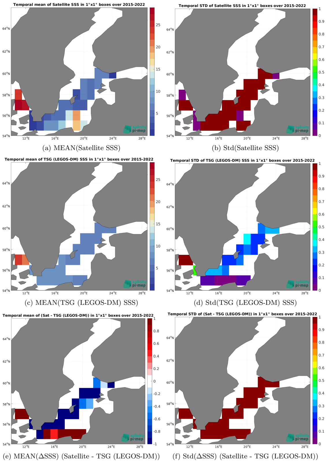
Figure 7: Temporal mean (left) and Std (right) of SSS from SMAP SSS L2 v5.0 (JPL) (top), TSG (LEGOS-DM) (middle), and of \Delta SSS (Satellite - TSG (LEGOS-DM)). Only match-up pairs are used to generate these maps.
