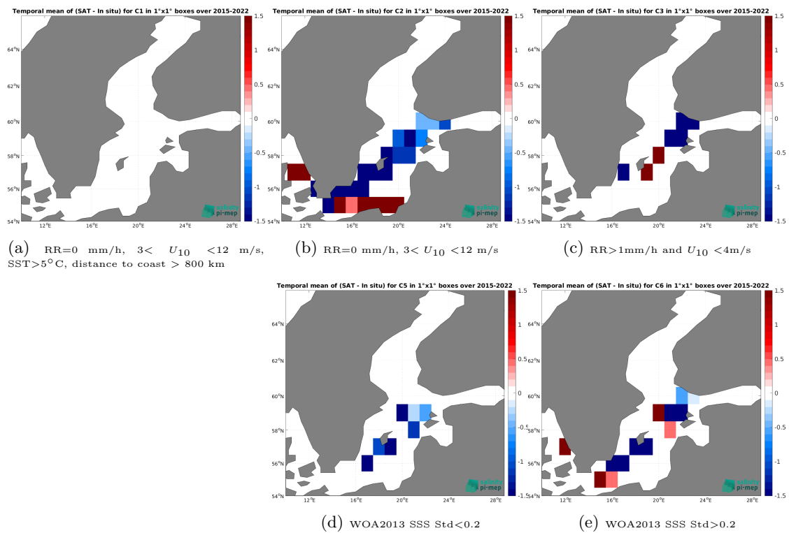
Figure 14: Temporal mean gridded over spatial boxes of size 1^\circ \times 1^\circ of \Delta SSS (SMAP SSS L2 v5.0 (JPL) - TSG (LEGOS-DM)) for 5 different subdatasets corresponding to:RR=0 mm/h, 3 < U_{10} < 12 m/s, SST >5^\circ\text{C} , distance to coast > 800 km (a), RR=0 mm/h, 3 < U_{10} < 12 m/s (b), RR >1 mm/h and U_{10} < 4 m/s (c), WOA2013 SSS Std <0.2 (d), WOA2013 SSS Std >0.2 (e).
