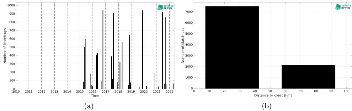
Figure 2: Number of match-ups between TSG (LEGOS-DM) and SMAP SSS L2 v5.0 (JPL) SSS as a function of time (a) and as function of the distance to coast (b) over the Baltic Sea Pi-MEP region and for the full satellite product period.
