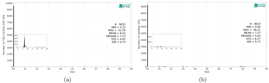
Figure 3: Histograms of SSS from TSG (LEGOS-DM) (a) and SMAP SSS L2 v5.0 (JPL) (b) considering all match-up pairs per bins of 0.1 over the Baltic Sea Pi-MEP region and for the full satellite product period.
