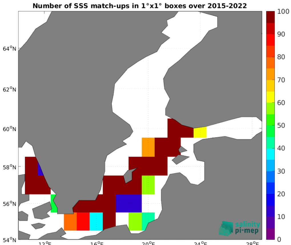
Figure 4: Number of SSS match-ups between TSG (LEGOS-DM) SSS and the SMAP SSS L2 v5.0 (JPL) SSS product for the Baltic Sea Pi-MEP region over 1^\circ \times 1^\circ boxes and for the full satellite product period.
