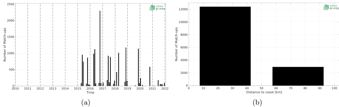
Figure 1: Number of match-ups between TSG (LEGOS-DM) and SMAP SSS L2 v5.0 (JPL) SSS as a function of time (a) and as function of the distance to coast (b) over the Baltic Sea Pi-MEP region and for the full satellite product period.
