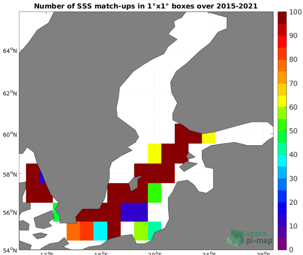
Figure 4: Number of SSS match-ups between TSG (LEGOS-DM) SSS and the SMAP SSS L2 v5.0 (JPL) SSS product for the Baltic Sea Pi-MEP region over 1°×1° boxes and for the full satellite product period.
