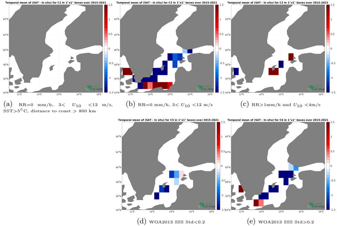
Figure 12: Temporal mean gridded over spatial boxes of size 1^{\circ}\times 1^{\circ} of \Delta\text{SSS} (SMAP SSS L2 v5.0 (JPL) - TSG (LEGOS-DM)) for 5 different subdatasets corresponding to:RR=0 mm/h, 3 < U_{10} < 12 m/s, SST >5^{\circ}\text{C} , distance to coast > 800 km (a), RR=0 mm/h, 3 < U_{10} < 12 m/s (b), RR >1 mm/h and U_{10} < 4 m/s (c), WOA2013 SSS Std <0.2 (d), WOA2013 SSS Std >0.2 (e).
