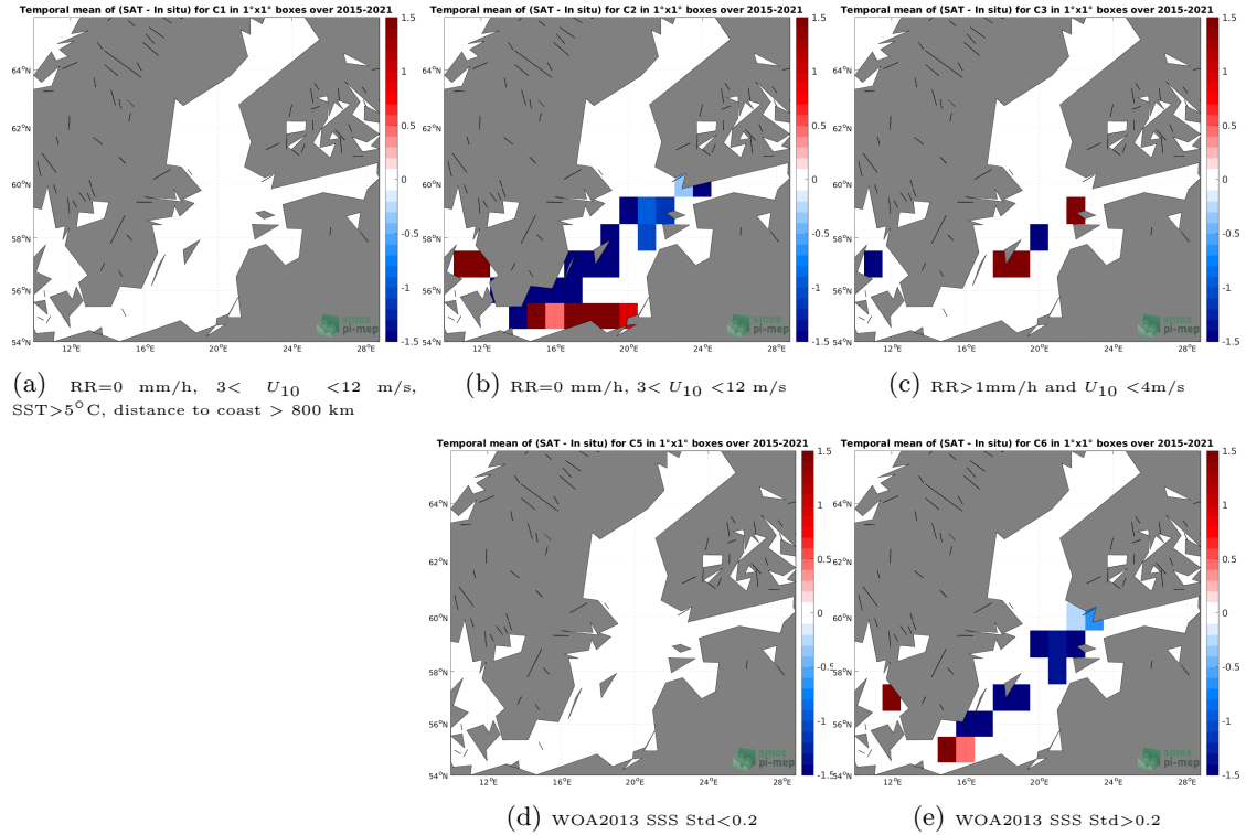
Figure 12: Temporal mean gridded over spatial boxes of size 1^{\circ}\times 1^{\circ} of \Delta\text{SSS} (SMAP SSS L2 v5.0 (JPL) - TSG (LEGOS-DM)) for 5 different subdatasets corresponding to: \text{RR}=0 mm/h, 3 < U_{10} < 12 m/s, \text{SST} > 5^{\circ}\text{C} , distance to coast > 800 km (a), \text{RR}=0 mm/h, 3 < U_{10} < 12 m/s (b), \text{RR} > 1\text{mm/h} and U_{10} < 4\text{m/s} (c), WOA2013 SSS Std < 0.2 (d), WOA2013 SSS Std > 0.2 (e).
