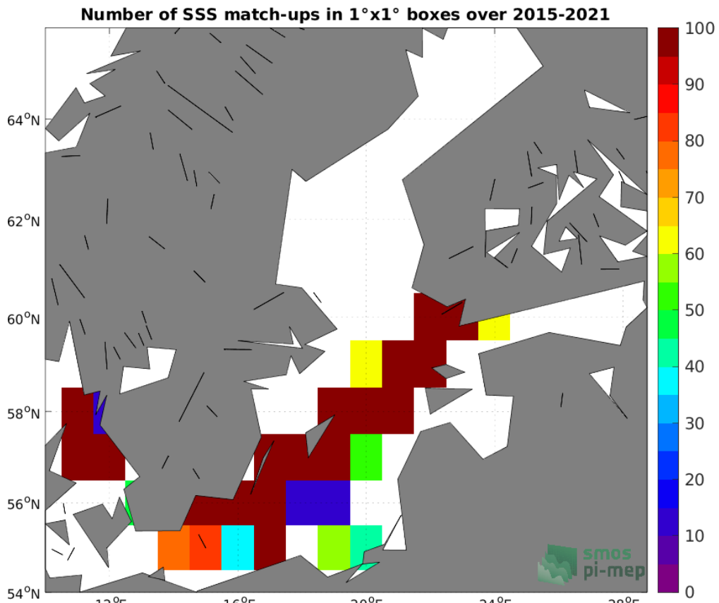
Figure 4: Number of SSS match-ups between TSG (LEGOS-DM) SSS and the SMAP SSS L2 v5.0 (JPL) SSS product for the Baltic Sea Pi-MEP region over 1°x1° boxes and for the full satellite product period.
