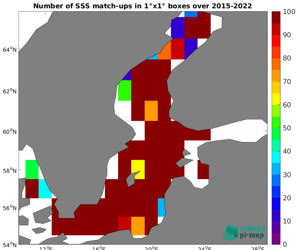
Figure 5: Number of SSS match-ups between ICES SSS and the SMAP SSS L2 v5.0 (JPL) SSS product for the Baltic Sea Pi-MEP region over 1°x1° boxes and for the full satellite product period.
