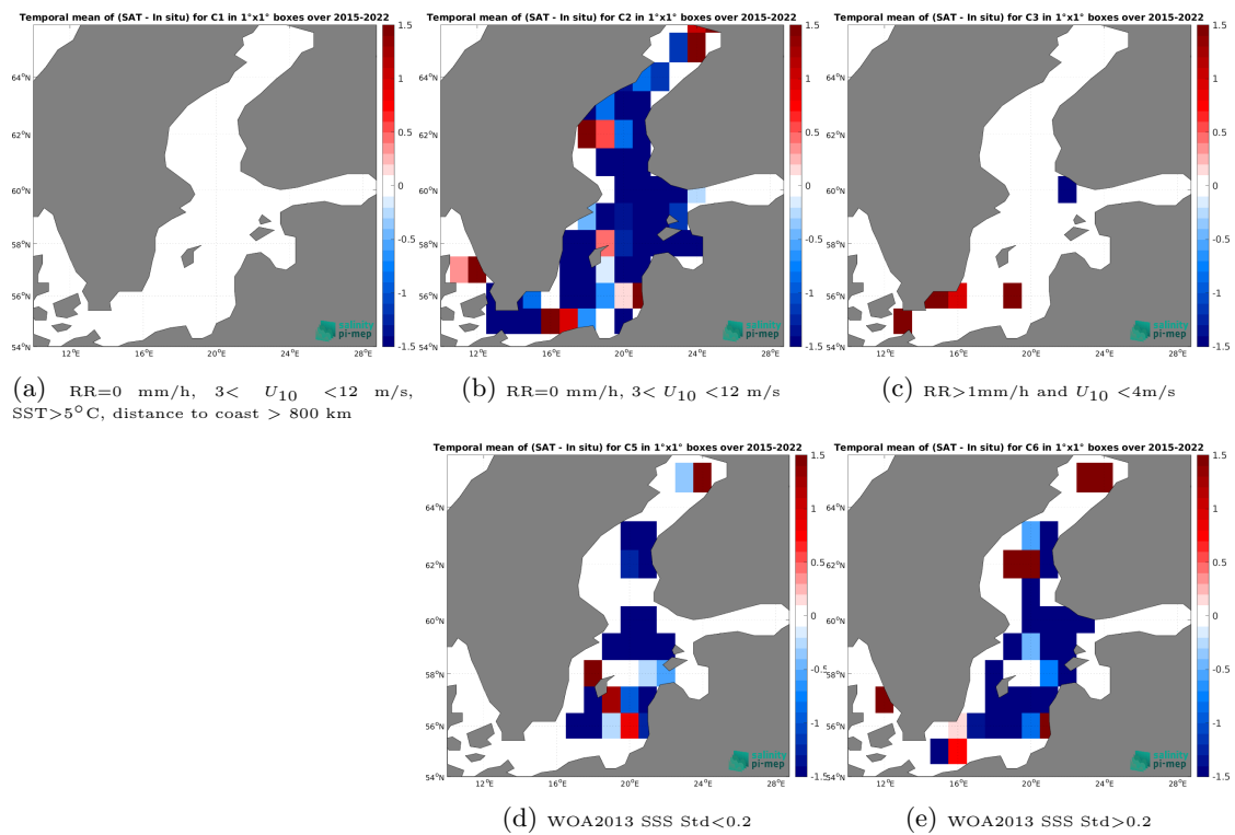
Figure 14: Temporal mean gridded over spatial boxes of size 1^\circ \times 1^\circ of \Delta\text{SSS} (SMAP SSS L2 v5.0 (JPL) - ICES) for 5 different subdatasets corresponding to: RR=0 mm/h, 3 < U_{10} < 12 m/s, SST > 5°C, distance to coast > 800 km (a), RR=0 mm/h, 3 < U_{10} < 12 m/s (b), RR > 1mm/h and U_{10} < 4 m/s (c), WOA2013 SSS Std < 0.2 (d), WOA2013 SSS Std > 0.2 (e).
