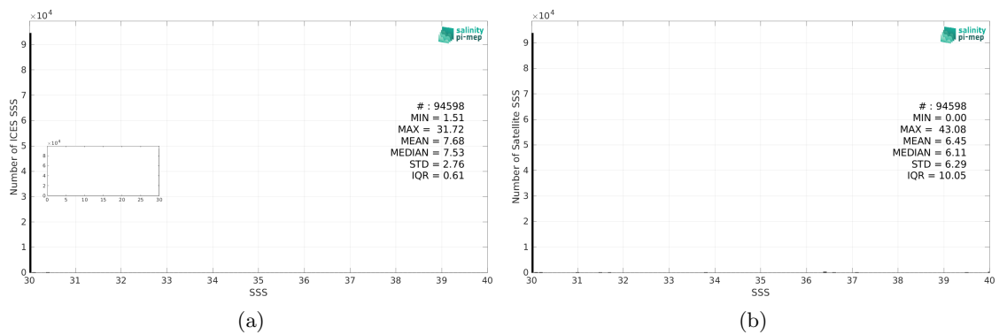
Figure 2: Histograms of SSS from ICES (a) and SMAP SSS L2 v5.0 (JPL) (b) considering all match-up pairs per bins of 0.1 over the Baltic Sea Pi-MEP region and for the full satellite product period.
