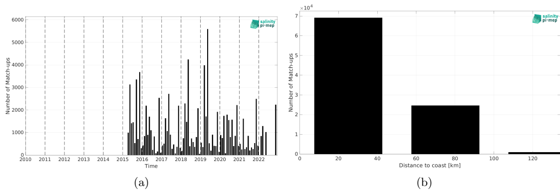
Figure 1: Number of match-ups between ICES and SMAP SSS L2 v5.0 (JPL) SSS as a function of time (a) and as function of the distance to coast (b) over the Baltic Sea Pi-MEP region and for the full satellite product period.
