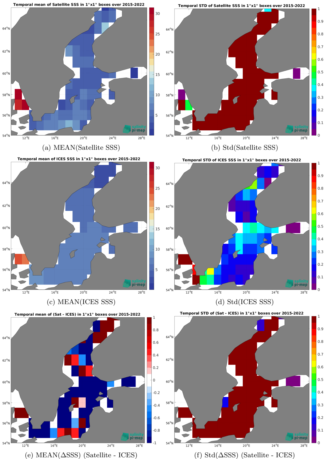
Figure 6: Temporal mean (left) and Std (right) of SSS from SMAP SSS L2 v5.0 (JPL) (top), ICES (middle), and of \Delta SSS (Satellite - ICES) (bottom). Only match-up pairs are used to generate these maps.
