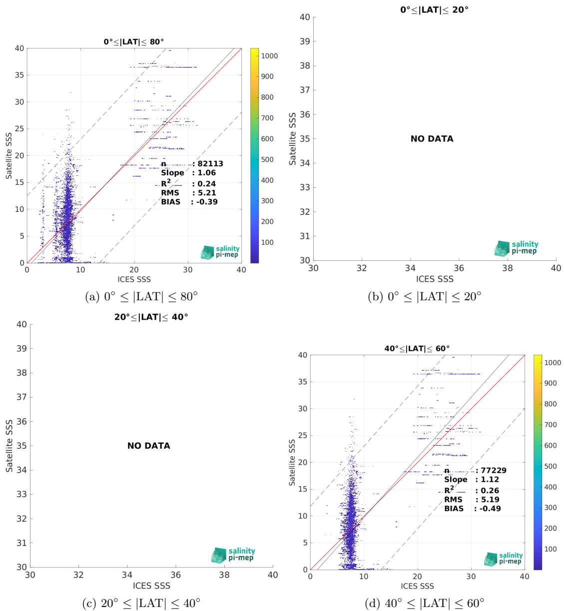
Figure 9: Contour maps of the concentration of SMAP SSS L2 v5.0 (JPL) SSS (y-axis) versus ICES SSS (x-axis) at match-up pairs for different latitude bands. For each plot, the red line shows x=y . The black thin and dashed lines indicate a linear fit through the data cloud and the \pm 95\% confidence levels, respectively. The number match-up pairs n , the slope and R^2 coefficient of the linear fit, the root mean square (RMS) and the mean bias between satellite and in situ data are indicated for each latitude band in each plots.
