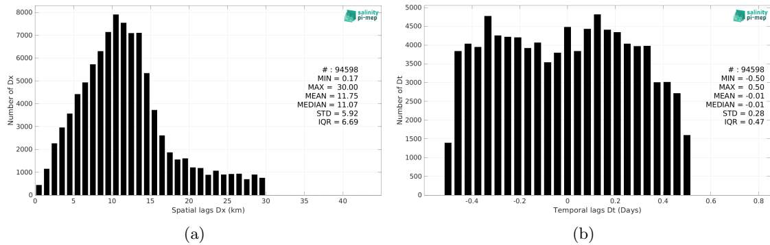
Figure 5: Histograms of the spatial (a) and temporal (b) lags between the location/time of the ICES measurement and the date of the corresponding SMAP SSS L2 v5.0 (JPL) SSS pixel.
