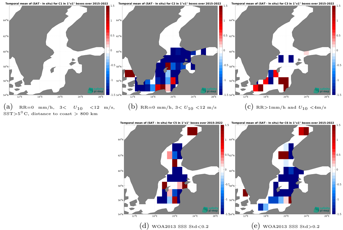
Figure 12: Temporal mean gridded over spatial boxes of size 1^{\circ}\times 1^{\circ} of \Delta\text{SSS} (SMAP SSS L2 v5.0 (JPL) - ICES) for 5 different subdatasets corresponding to:RR=0 mm/h, 3 < U_{10} < 12 m/s, SST >5^{\circ}\text{C} , distance to coast > 800 km (a), RR=0 mm/h, 3 < U_{10} < 12 m/s (b), RR >1 mm/h and U_{10} < 4 m/s (c), WOA2013 SSS Std <0.2 (d), WOA2013 SSS Std >0.2 (e).
