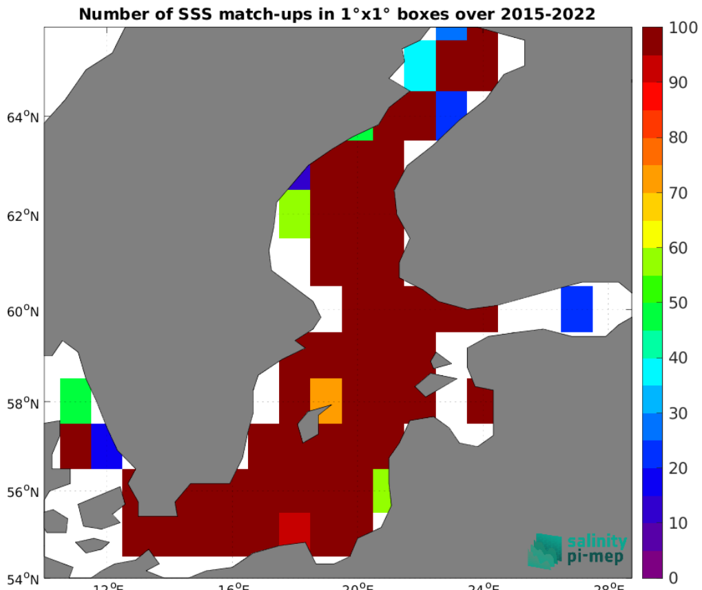
Figure 4: Number of SSS match-ups between ICES SSS and the SMAP SSS L2 v5.0 (JPL) SSS product for the Baltic Sea Pi-MEP region over 1^\circ \times 1^\circ boxes and for the full satellite product period.
