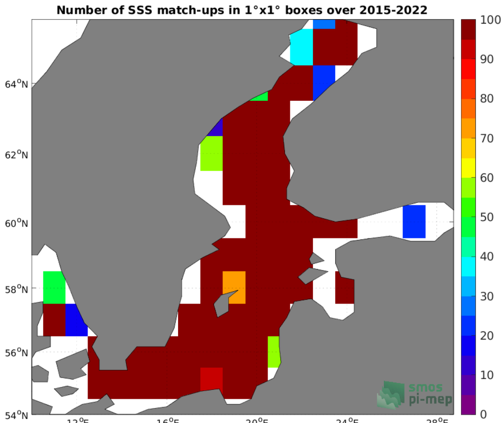
Figure 4: Number of SSS match-ups between ICES SSS and the SMAP SSS L2 v5.0 (JPL) SSS product for the Baltic Sea Pi-MEP region over 1°x1° boxes and for the full satellite product period.
