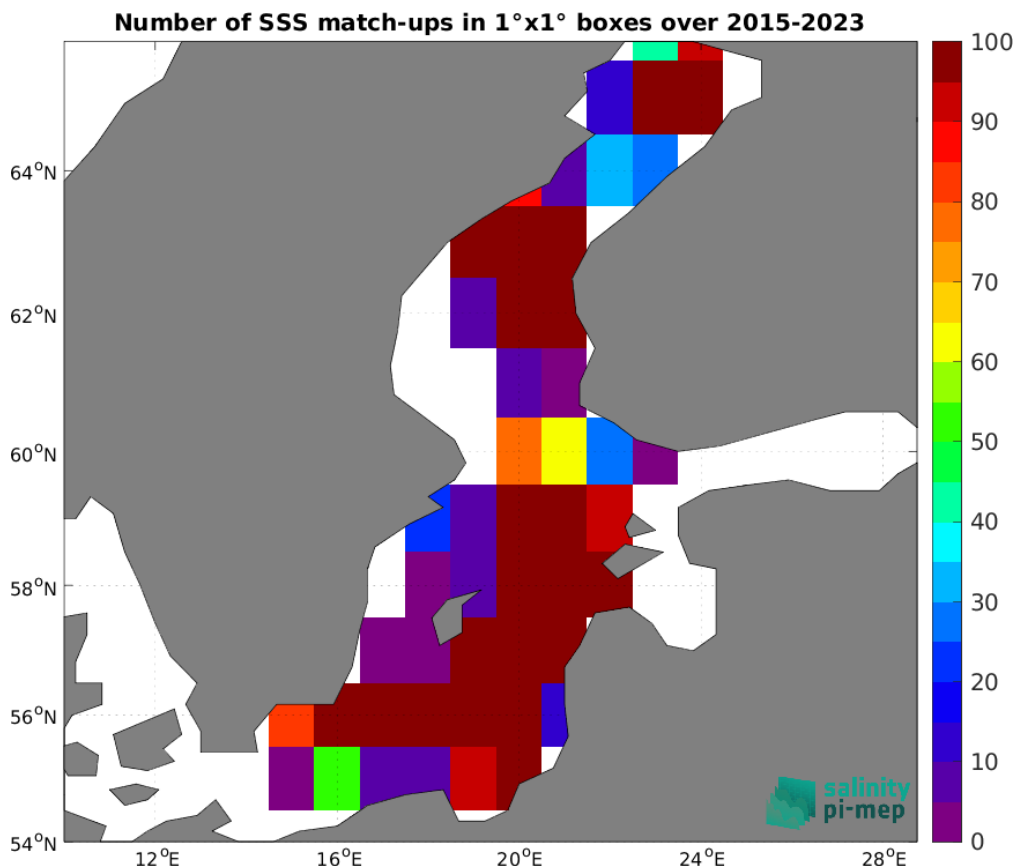
Figure 4: Number of SSS match-ups between Argo SSS and the SMAP SSS L2 v5.0 (JPL) SSS product for the Baltic Sea Pi-MEP region over 1^\circ \times 1^\circ boxes and for the full satellite product period.
