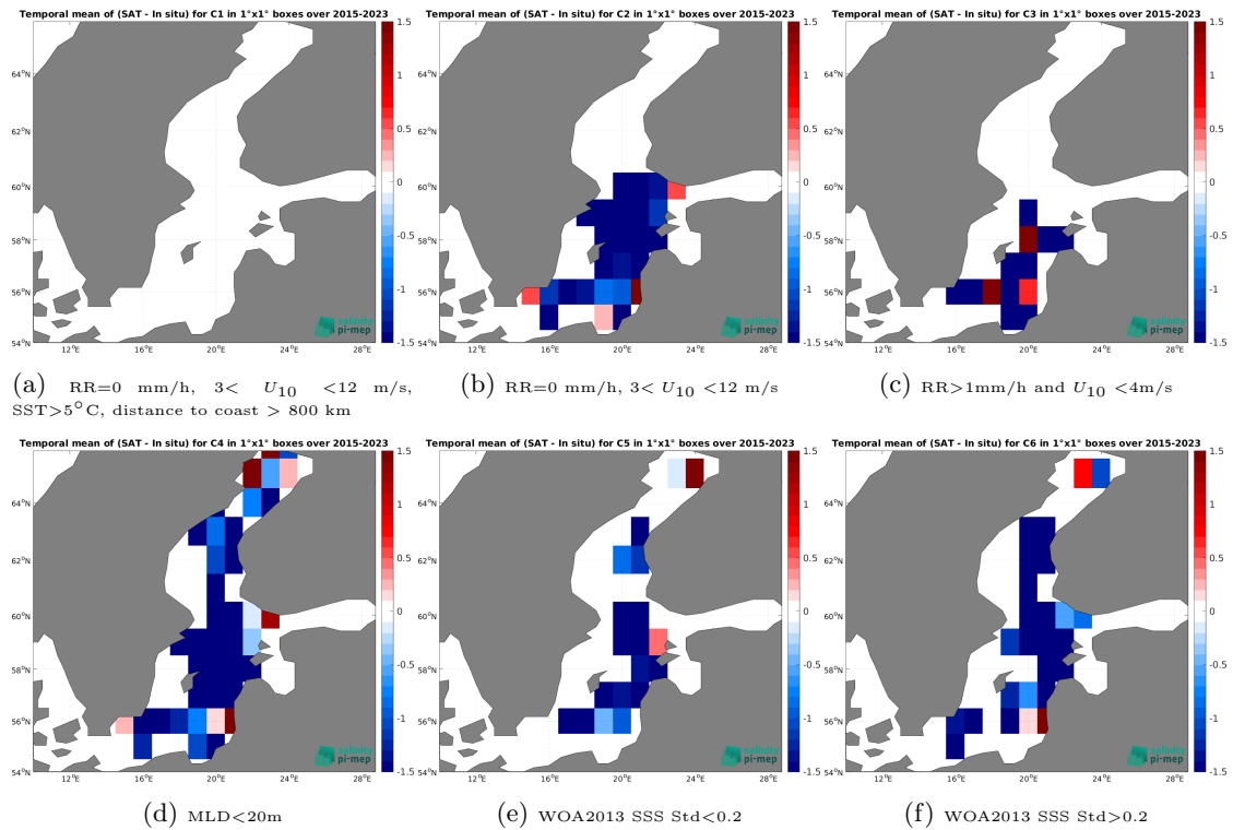
Figure 12: Temporal mean gridded over spatial boxes of size 1^{\circ}\times 1^{\circ} of \Delta\text{SSS} (SMAP SSS L2 v5.0 (JPL) - Argo) for 6 different subdatasets corresponding to:RR=0 mm/h, 3 < U_{10} < 12 m/s, SST >5^{\circ}\text{C} , distance to coast > 800 km (a), RR=0 mm/h, 3 < U_{10} < 12 m/s (b), RR >1 mm/h and U_{10} < 4 m/s (c),MLD <20 m (d),WOA2013 SSS Std <0.2 (e),WOA2013 SSS Std >0.2 (f).
