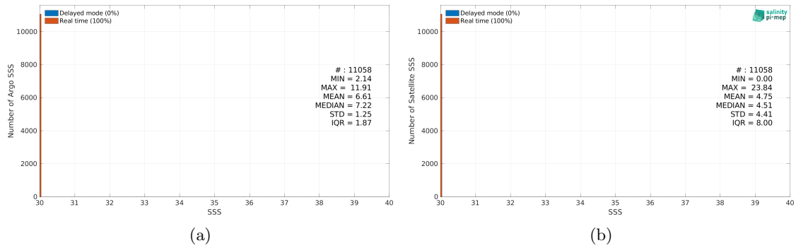
Figure 2: Histograms of SSS from Argo (a) and SMAP SSS L2 v5.0 (JPL) (b) considering all match-up pairs per bins of 0.1 over the Baltic Sea Pi-MEP region and for the full satellite product period.
