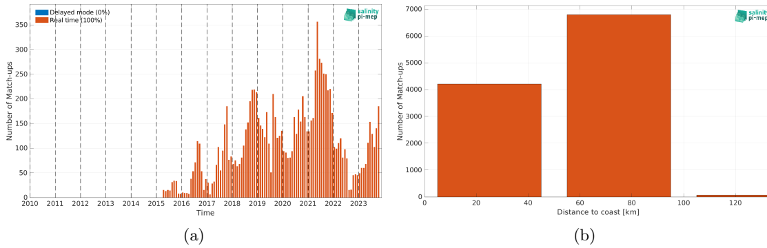
Figure 1: Number of match-ups between Argo and SMAP SSS L2 v5.0 (JPL) SSS as a function of time (a) and as function of the distance to coast (b) over the Baltic Sea Pi-MEP region and for the full satellite product period.
