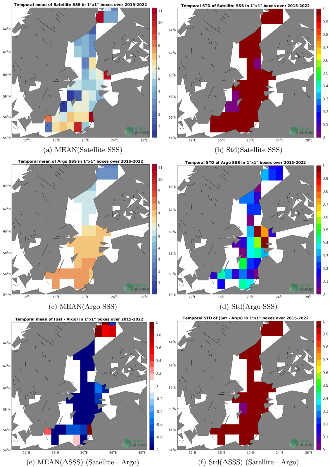
Figure 6: Temporal mean (left) and Std (right) of SSS from SMAP SSS L2 v5.0 (JPL) (top), Argo (middle), and of \Delta SSS (Satellite - Argo) (bottom). Only match-up pairs are used to generate these maps.
