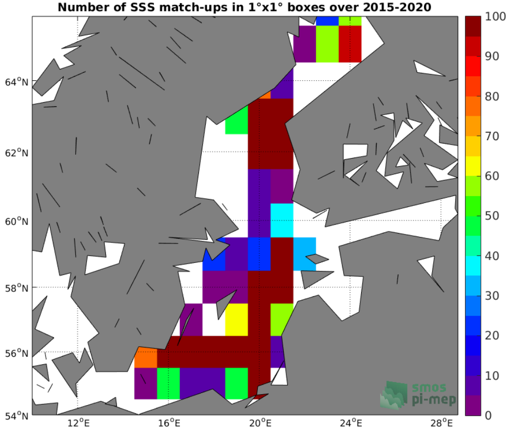
Figure 4: Number of SSS match-ups between Argo SSS and the SMAP SSS L2 v5.0 (JPL) SSS product for the Baltic Sea Pi-MEP region over 1°x1° boxes and for the full satellite product period.
