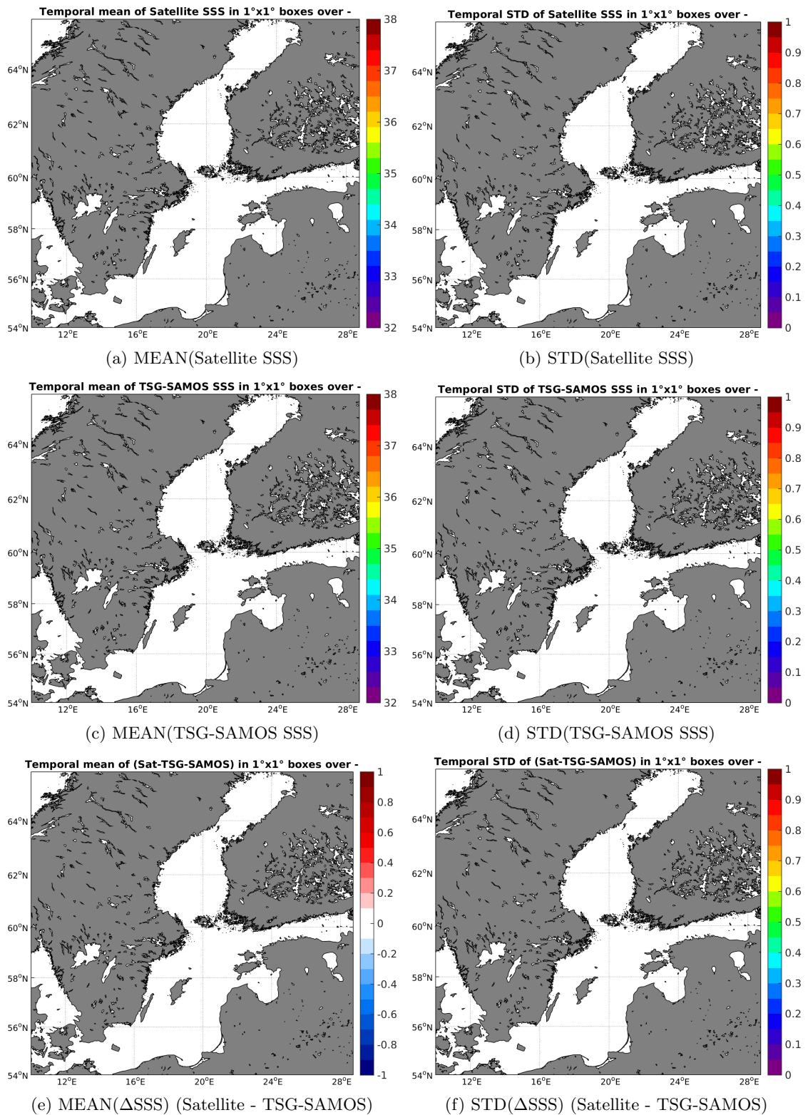
Figure 6: Temporal mean (left) and STD (right) of SSS from SMAP-L2-JPL-V4 (top), TSG-SAMOS (middle), and of \Delta SSS (Satellite - TSG-SAMOS). Only match-up pairs are used to generate these maps.
