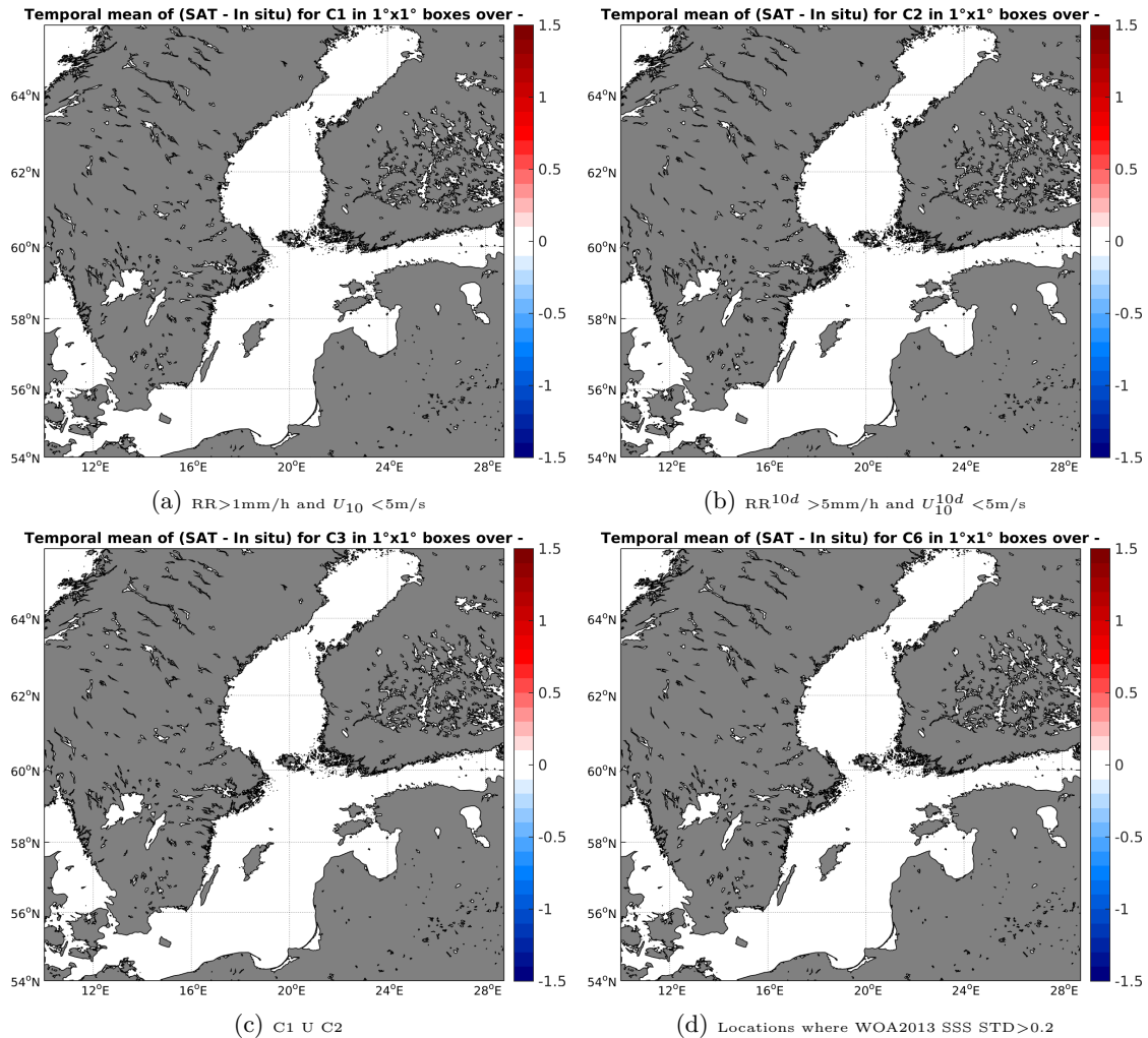
Figure 12: Temporal mean gridded over spatial boxes of size 1^\circ \times 1^\circ of \Delta SSS (SMAP-L2-JPL-V4 - TSG-SAMOS) for 4 different subdatasets corresponding to: RR > 1mm/h and U_{10} < 5\text{m/s} (a), RR^{10d} > 5\text{mm/h} and U_{10}^{10d} < 5\text{m/s} (b), C1 U C2 (c), Locations where WOA2013 SSS STD > 0.2 (d).
