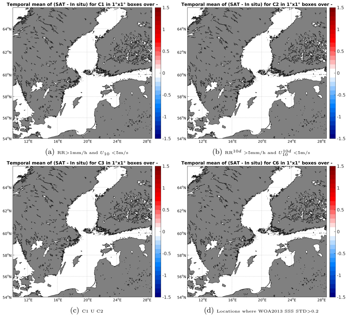
Figure 12: Temporal mean gridded over spatial boxes of size 1^\circ \times 1^\circ of \Delta SSS (SMAP-L2-JPL-V4 - TSG-SAMOS) for 4 different subdatasets corresponding to: RR > 1\text{mm/h} and U_{10} < 5\text{m/s} (a), RR^{10d} > 5\text{mm/h} and U_{10}^{10d} < 5\text{m/s} (b), C1 U C2 (c), Locations where WOA2013 SSS STD > 0.2 (d).
