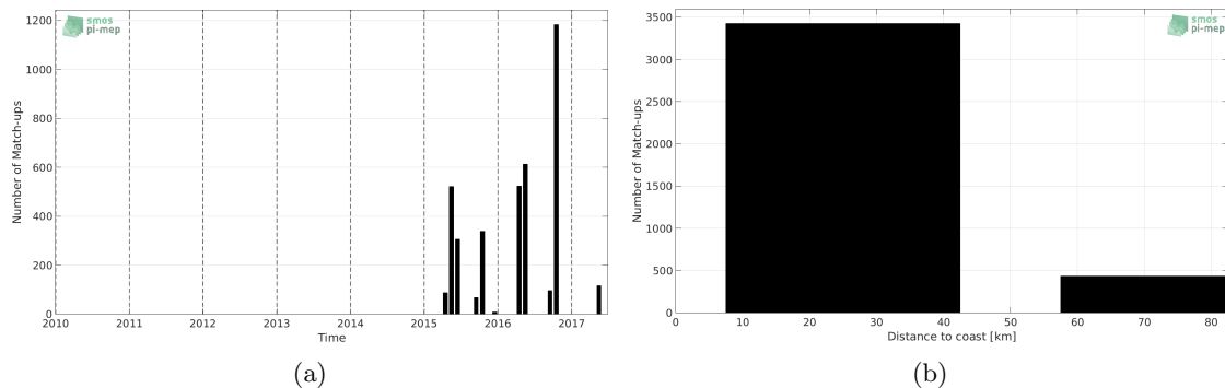
Figure 1: Number of match-ups between TSG-LEGOS-DM and SMAP-L2-JPL-V4 SSS as a function of time (a) and as function of the distance to coast (b) over the Baltic Sea Pi-MEP region and for the full satellite product period.
