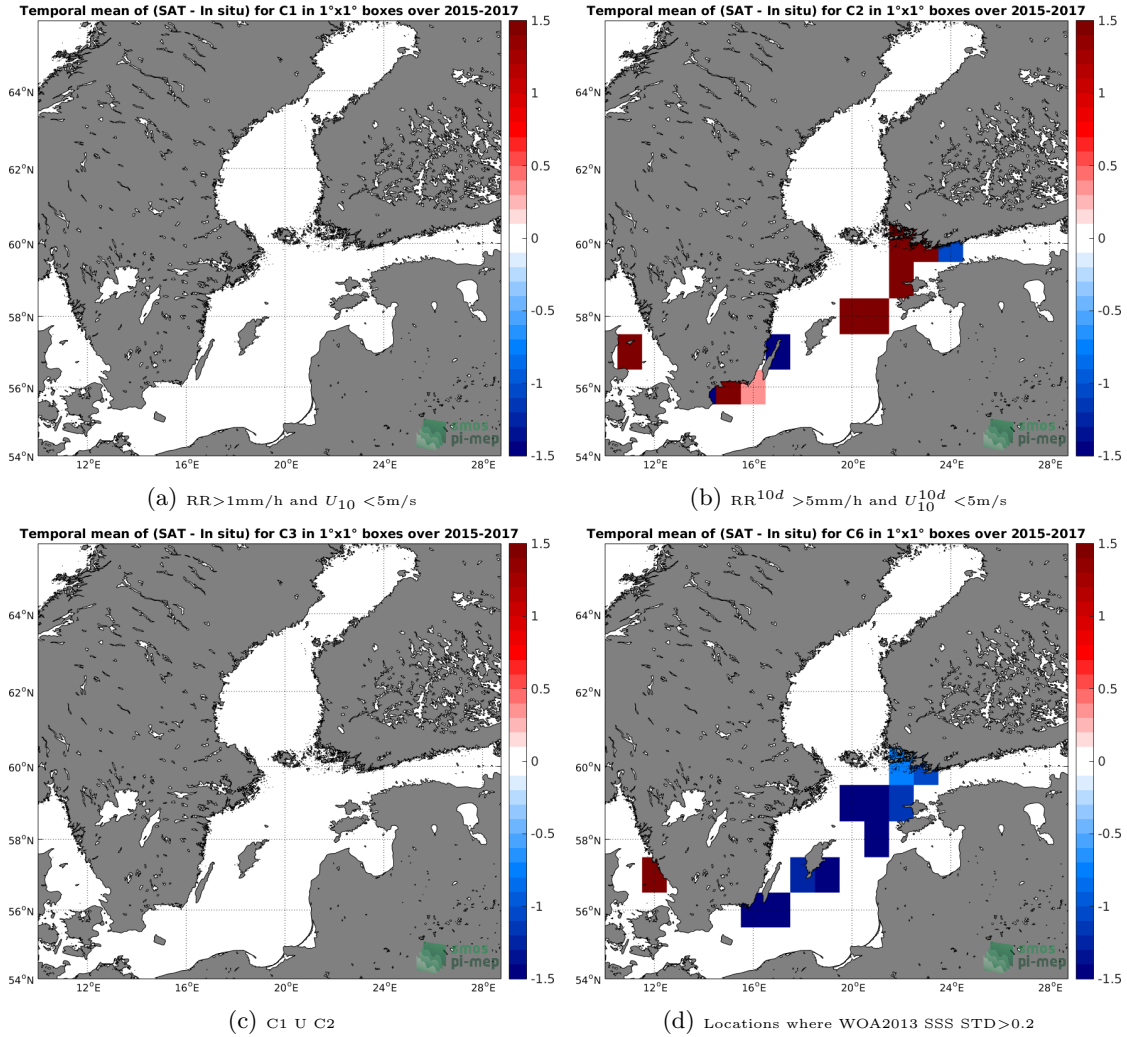
Figure 12: Temporal mean gridded over spatial boxes of size 1^\circ \times 1^\circ of \Delta SSS (SMAP-L2-JPL-V4 - TSG-LEGOS-DM) for 4 different subdatasets corresponding to: RR > 1\text{mm/h} and U_{10} < 5\text{m/s} (a), RR^{10d} > 5\text{mm/h} and U_{10}^{10d} < 5\text{m/s} (b), C1 U C2 (c), Locations where WOA2013 SSS STD > 0.2 (d).
