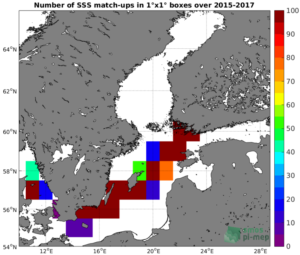
Figure 4: Number of SSS match-ups between TSG-LEGOS-DM SSS and the SMAP-L2-JPL-V4 SSS product for the Baltic Sea Pi-MEP region over 1°x1° boxes and for the full satellite product period.
