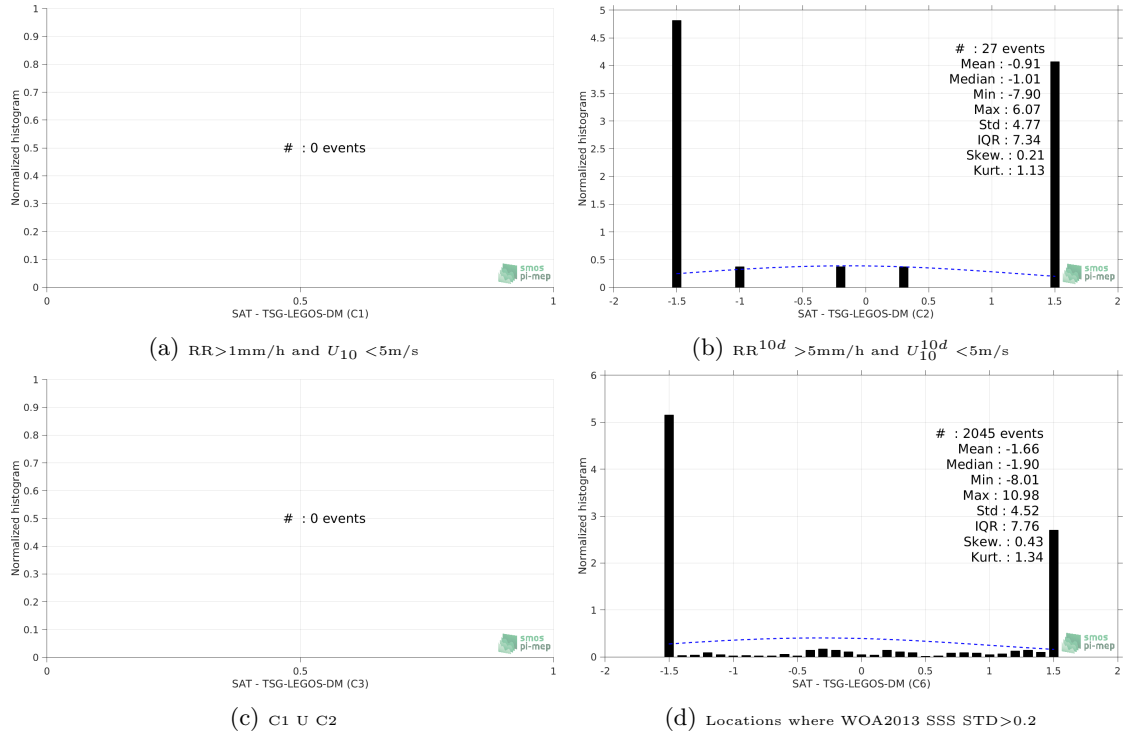
Figure 13: Normalized histogram of \Delta\text{SSS} (SMAP-L2-JPL-V4 - TSG-LEGOS-DM) for 6 different subdatasets corresponding to: RR > 1\text{mm/h} and U_{10} < 5\text{m/s} (a), RR^{10d} > 5\text{mm/h} and U_{10}^{10d} < 5\text{m/s} (b), C1 U C2 (c), Locations where WOA2013 SSS STD > 0.2 (d).
