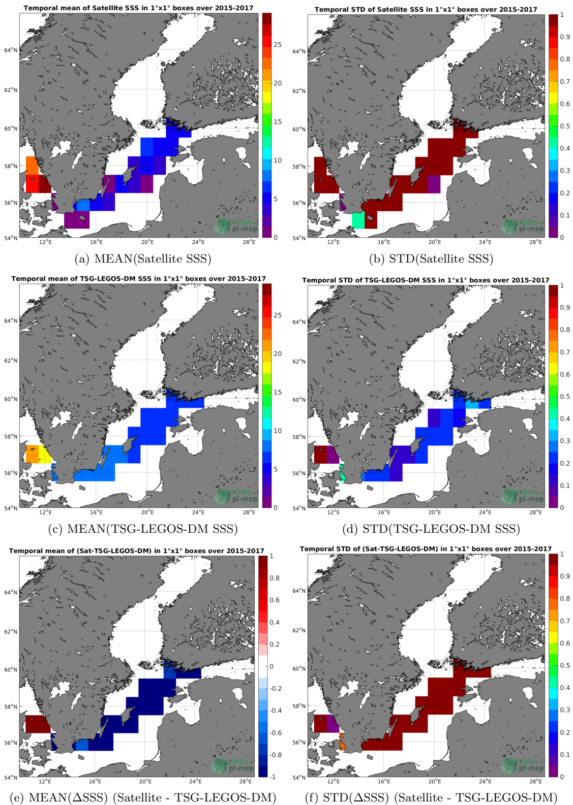
Figure 6: Temporal mean (left) and STD (right) of SSS from SMAP-L2-JPL-V4 (top), TSG-LEGOS-DM (middle), and of \Delta SSS (Satellite - TSG-LEGOS-DM). Only match-up pairs are used to generate these maps.
