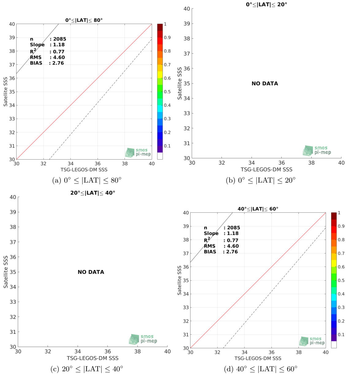
Figure 9: Contour maps of the concentration of SMAP-L2-JPL-V4 SSS (y-axis) versus TSG-LEGOS-DM SSS (x-axis) at match-up pairs for different latitude bands. For each plot, the red line shows x=y . The black thin and dashed lines indicate a linear fit through the data cloud and the \pm 95\% confidence levels, respectively. The number match-up pairs n , the slope and R^2 coefficient of the linear fit, the root mean square (RMS) and the mean bias between satellite and in situ data are indicated for each latitude band in each plots.
