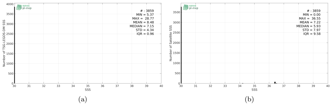
Figure 2: Histograms of SSS from TSG-LEGOS-DM (a) and SMAP-L2-JPL-V4 (b) considering all match-up pairs per bins of 0.1 over the Baltic Sea Pi-MEP region and for the full satellite product period.
