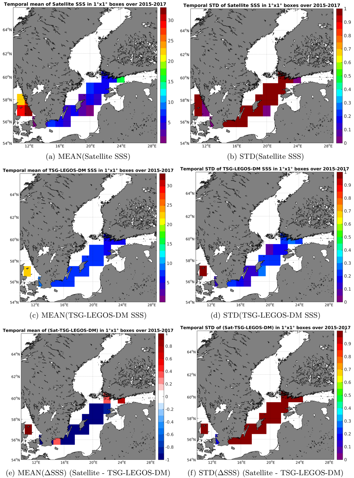
Figure 6: Temporal mean (left) and STD (right) of SSS from SMAP-L2-JPL-V4 (top), TSG-LEGOS-DM (middle), and of \Delta SSS (Satellite - TSG-LEGOS-DM). Only match-up pairs are used to generate these maps.
