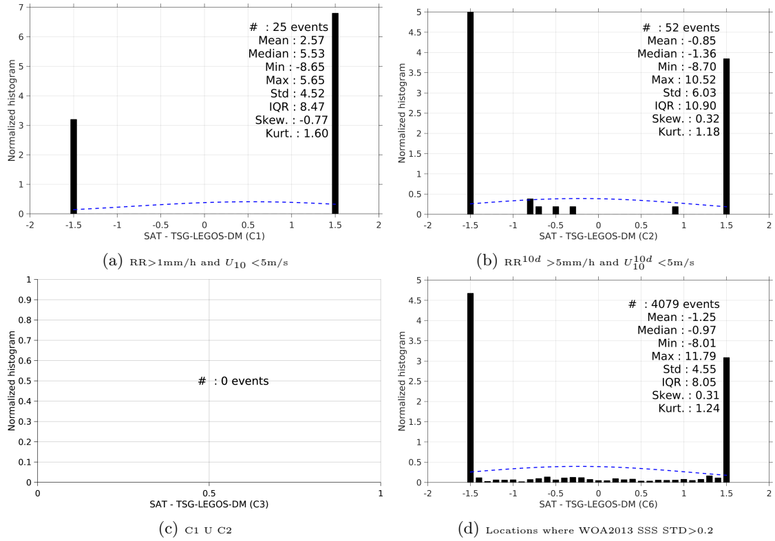
Figure 13: Normalized histogram of \Delta\text{SSS} (SMAP-L2-JPL-V4 - TSG-LEGOS-DM) for 6 different subdatasets corresponding to: RR > 1mm/h and U_{10} < 5\text{m/s} (a), RR^{10d} > 5\text{mm/h} and U_{10}^{10d} < 5\text{m/s} (b), C1 U C2 (c), Locations where WOA2013 SSS STD > 0.2 (d).
