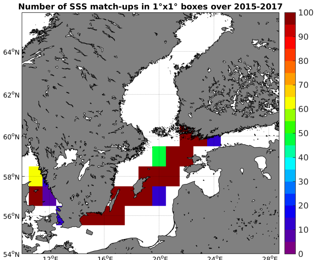
Figure 4: Number of SSS match-ups between TSG-LEGOS-DM SSS and the SMAP-L2-JPL-V4 SSS product for the Baltic Sea Pi-MEP region over 1°x1° boxes and for the full satellite product period.
