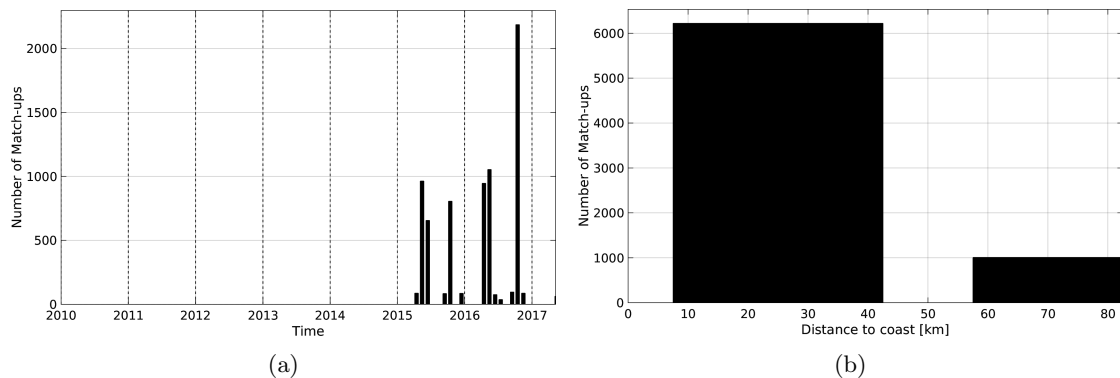
Figure 1: Number of match-ups between TSG-LEGOS-DM and SMAP-L2-JPL-V4 SSS as a function of time (a) and as function of the distance to coast (b) over the Baltic Sea Pi-MEP region and for the full satellite product period.
