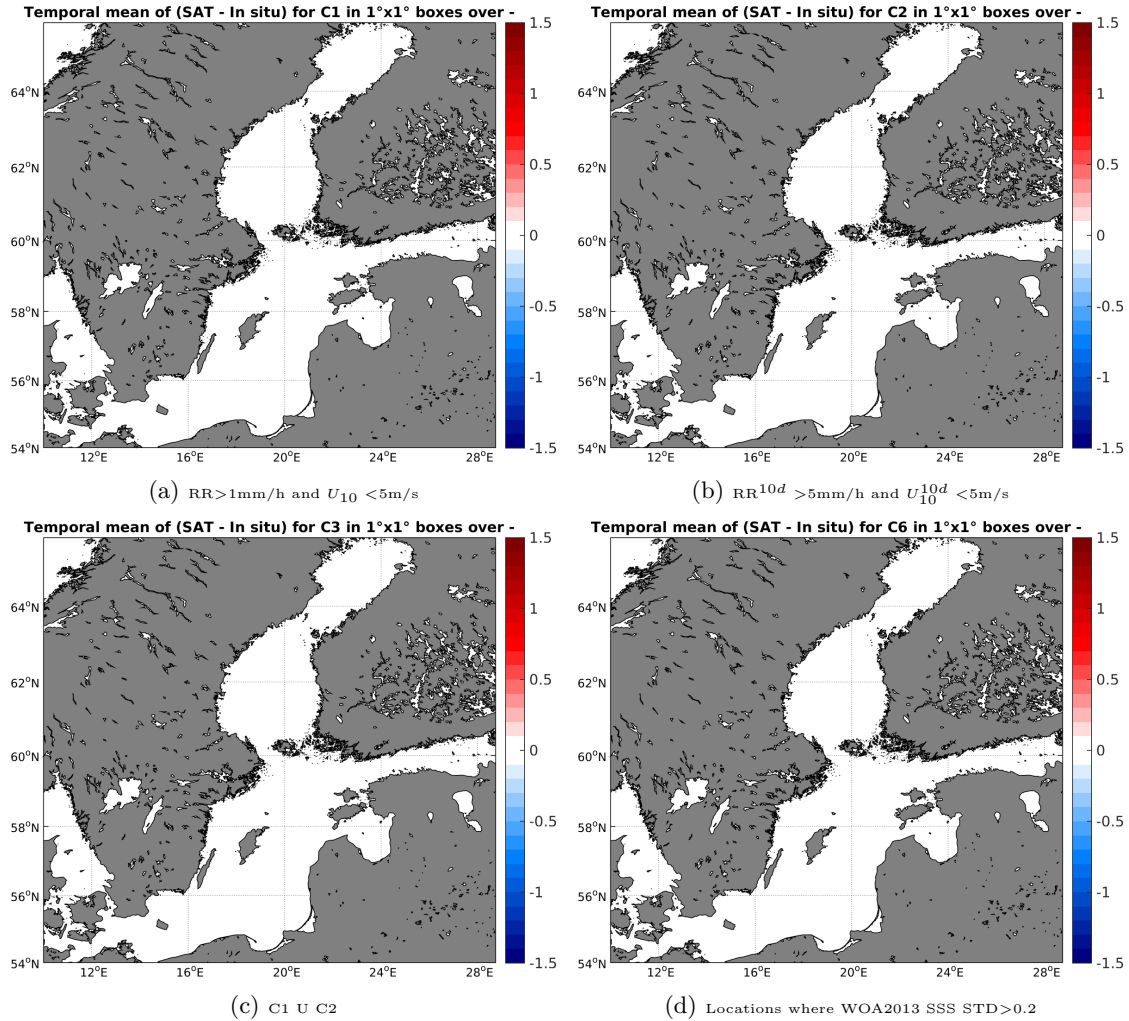
Figure 12: Temporal mean gridded over spatial boxes of size 1°x1° of \Delta SSS (SMAP-L2-JPL-V4 - TSG-GOSUD-Sailing-ship) for 4 different subdatasets corresponding to: RR > 1mm/h and U_{10} < 5m/s (a), RR^{10d} > 5mm/h and U_{10}^{10d} < 5m/s (b), C1 U C2 (c), Locations where WOA2013 SSS STD > 0.2 (d).
