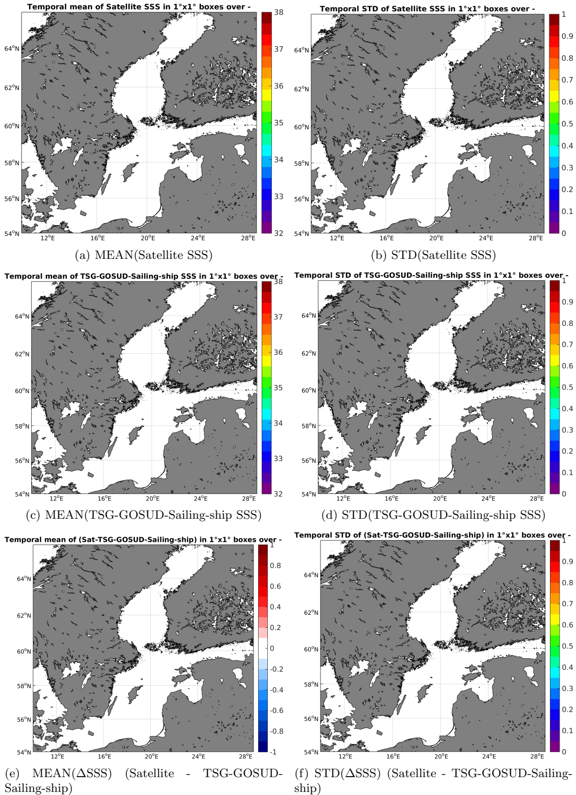
Figure 6: Temporal mean (left) and STD (right) of SSS from SMAP-L2-JPL-V4 (top), TSG-GOSUD-Sailing-ship (middle), and of \Delta SSS (Satellite - TSG-GOSUD-Sailing-ship). Only match-up pairs are used to generate these maps.
