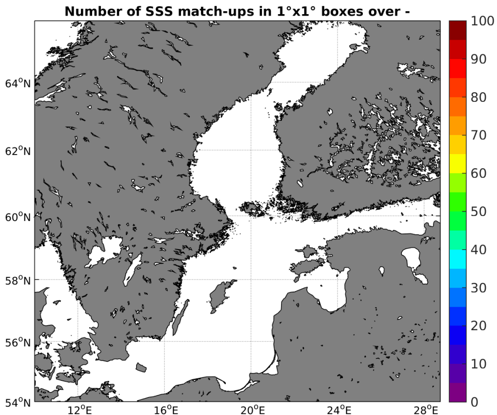
Figure 4: Number of SSS match-ups between TSG-GOSUD-Sailing-ship SSS and the SMAP-L2-JPL-V4 SSS product for the Baltic Sea Pi-MEP region over 1°x1° boxes and for the full satellite product period.
