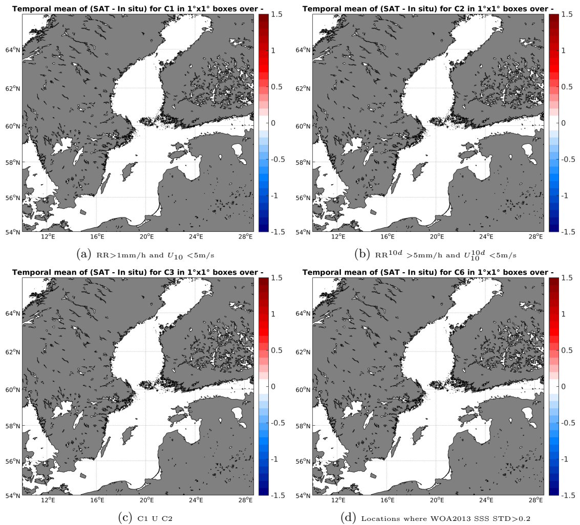
Figure 12: Temporal mean gridded over spatial boxes of size 1^\circ \times 1^\circ of \Delta SSS (SMAP-L2-JPL-V4 - TSG-GOSUD-Research-vessel) for 4 different subdatasets corresponding to:RR > 1 mm/h and U_{10} < 5 m/s (a), RR ^{10d} > 5 mm/h and U_{10}^{10d} < 5 m/s (b), C1 U C2 (c),Locations where WOA2013 SSS STD > 0.2 (d).
