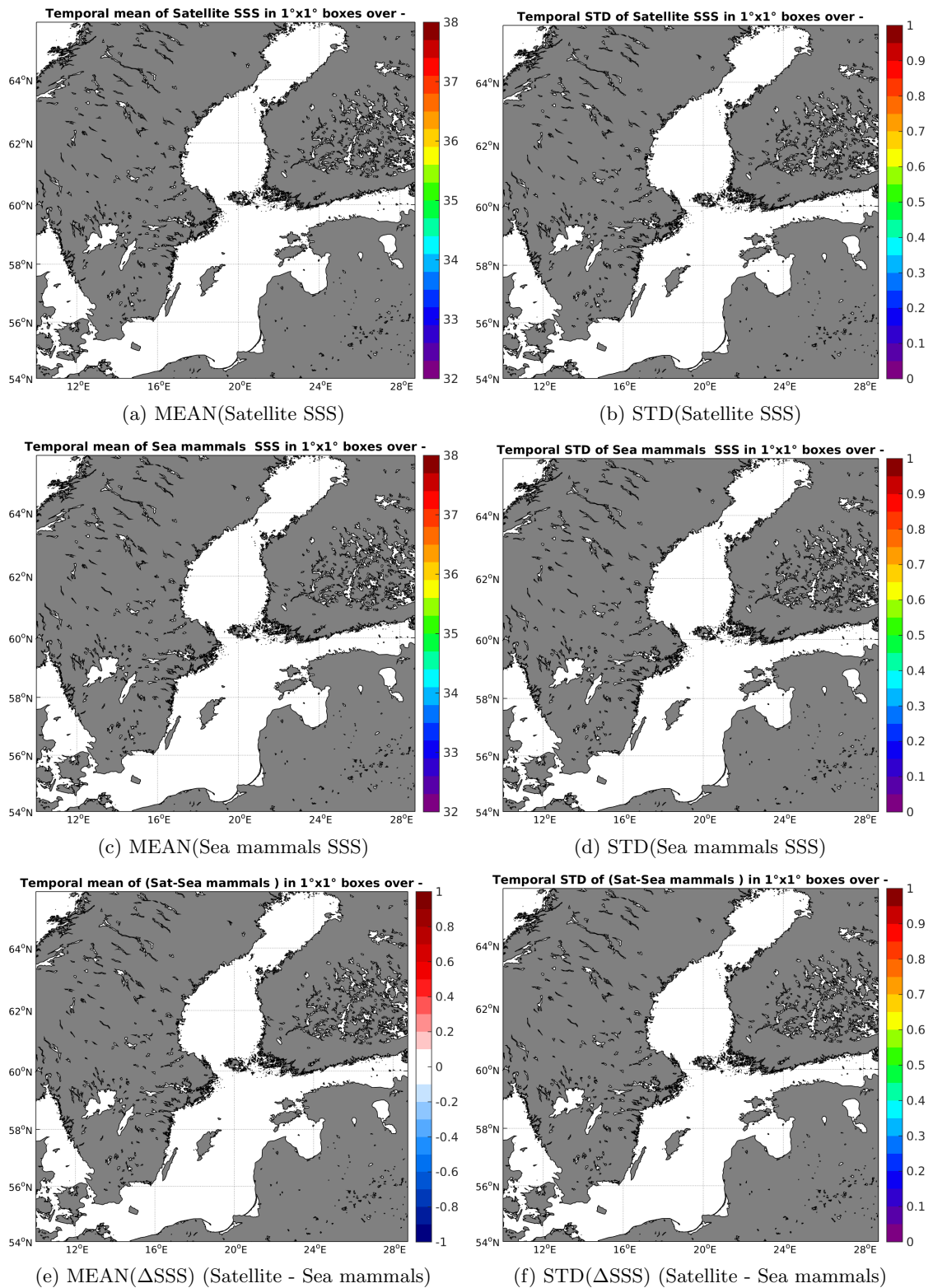
Figure 6: Temporal mean (left) and STD (right) of SSS from SMAP-L2-JPL-V4 (top), Sea mammals (middle), and of \Delta SSS (Satellite - Sea mammals). Only match-up pairs are used to generate these maps.
