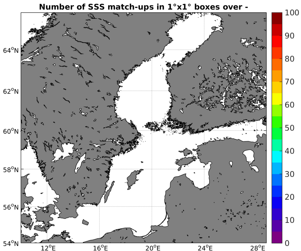
Figure 4: Number of SSS match-ups between Sea mammals SSS and the SMAP-L2-JPL-V4 SSS product for the Baltic Sea Pi-MEP region over 1°x1° boxes and for the full satellite product period.
