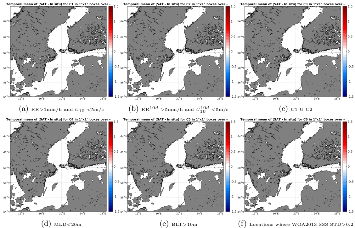
Figure 12: Temporal mean gridded over spatial boxes of size 1^\circ \times 1^\circ of \Delta SSS (SMAP-L2-JPL-V4 - Sea mammals) for 6 different subdatasets corresponding to: RR > 1mm/h and U_{10} < 5\text{m/s} (a), RR 10d > 5mm/h and U_{10}^{10d} < 5\text{m/s} (b), C1 U C2 (c), MLD < 20m (d), BLT > 10m (e), Locations where WOA2013 SSS STD > 0.2 (f).
